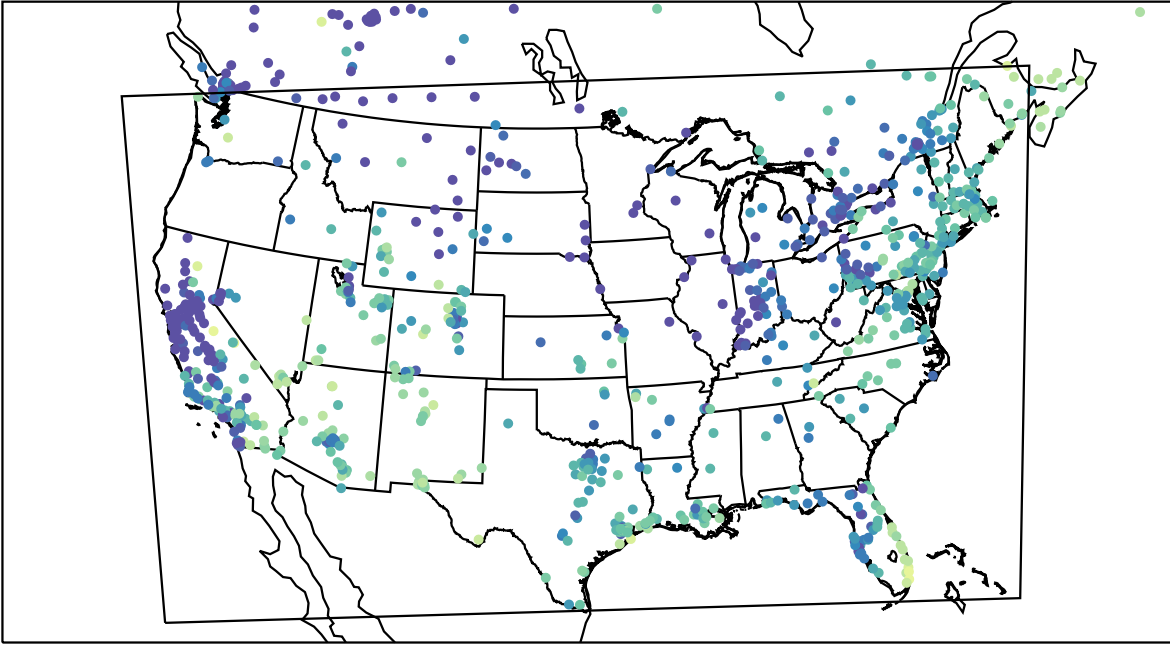
AirNOW (2024-01-08_17:00:00)
