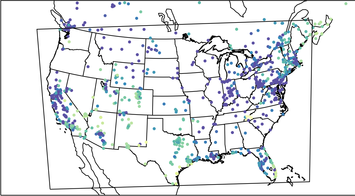
AirNOW (2024-01-08_10:00:00)
