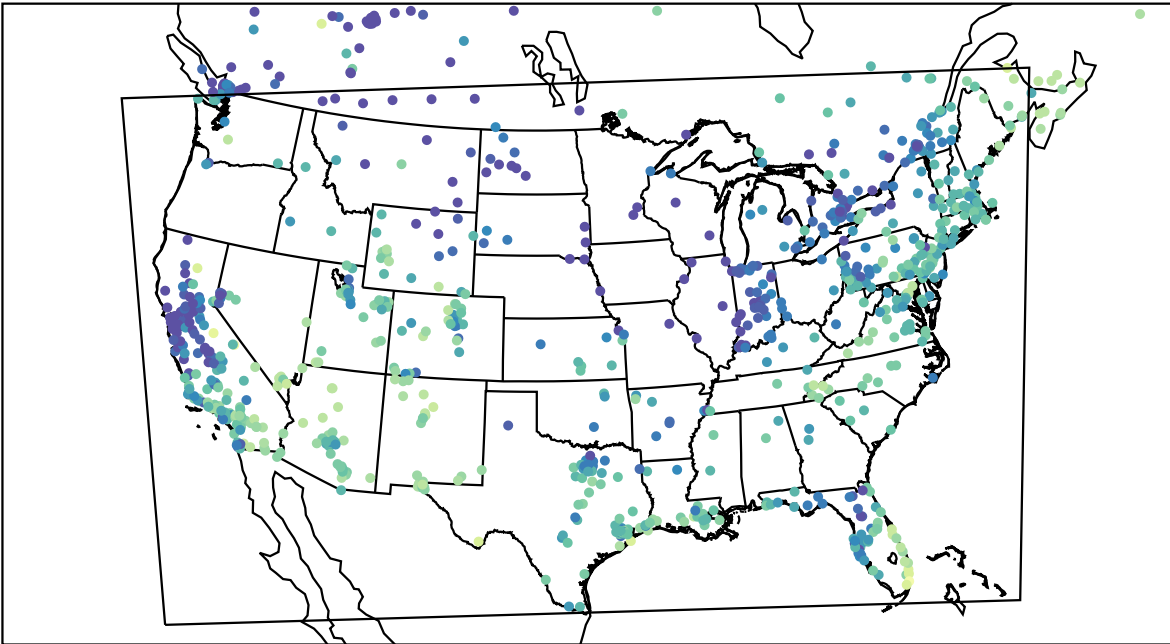
AirNOW (2024-01-08_18:00:00)
