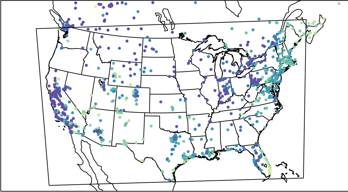
AirNOW (2024-01-08_16:00:00)
