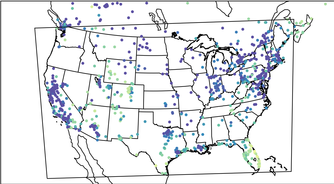
AirNOW (2024-01-09_03:00:00)
