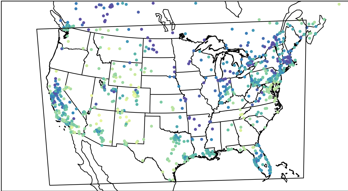
AirNOW (2024-01-09_20:00:00)
