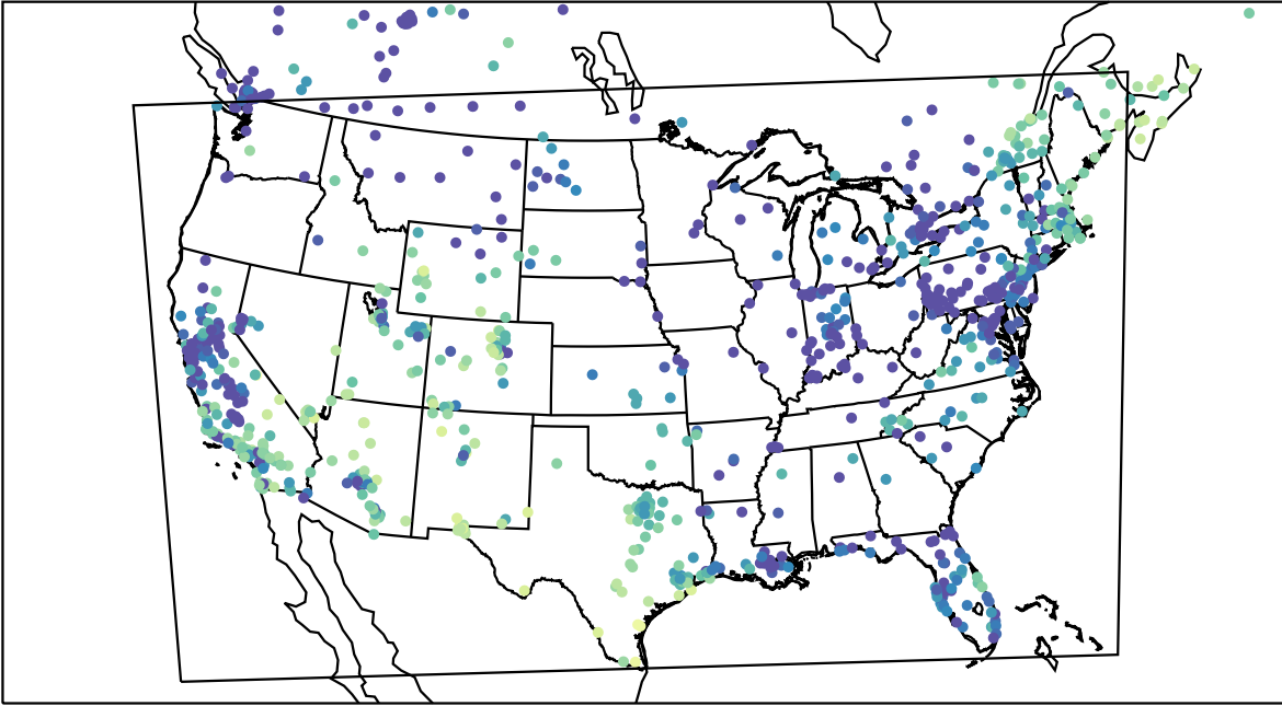
AirNOW (2024-01-08_03:00:00)
