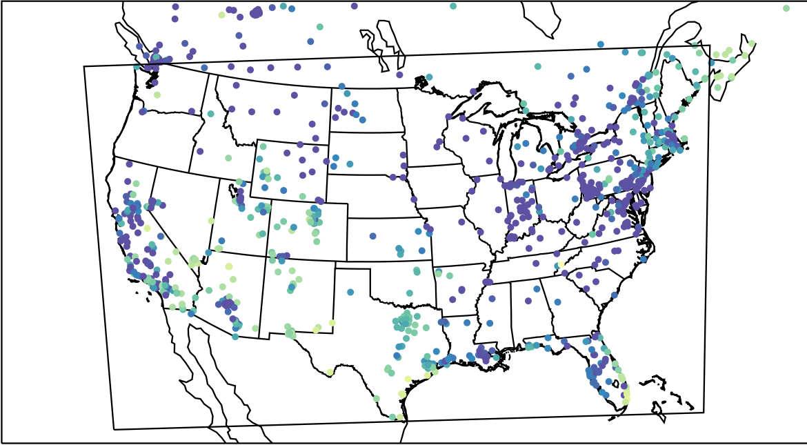
AirNOW (2024-01-08_11:00:00)
