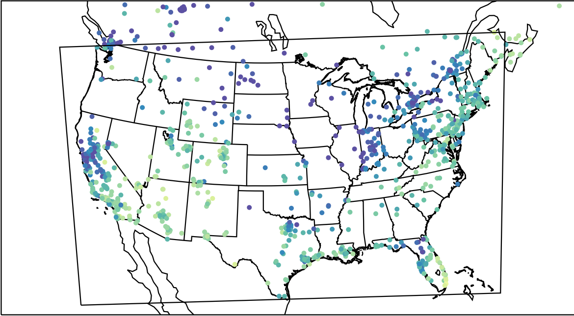
AirNOW (2024-01-08_19:00:00)
