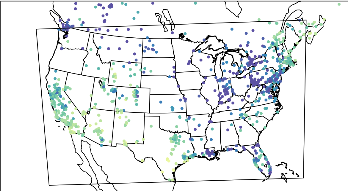
AirNOW (2024-01-08_00:00:00)
