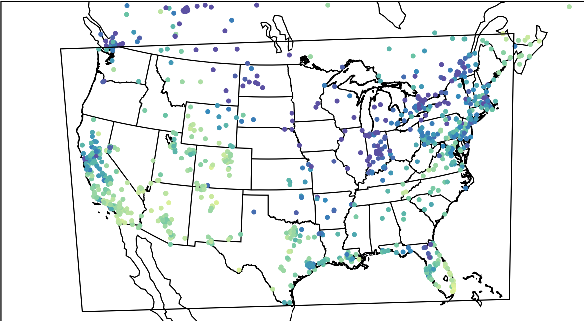
AirNOW (2024-01-08_21:00:00)
