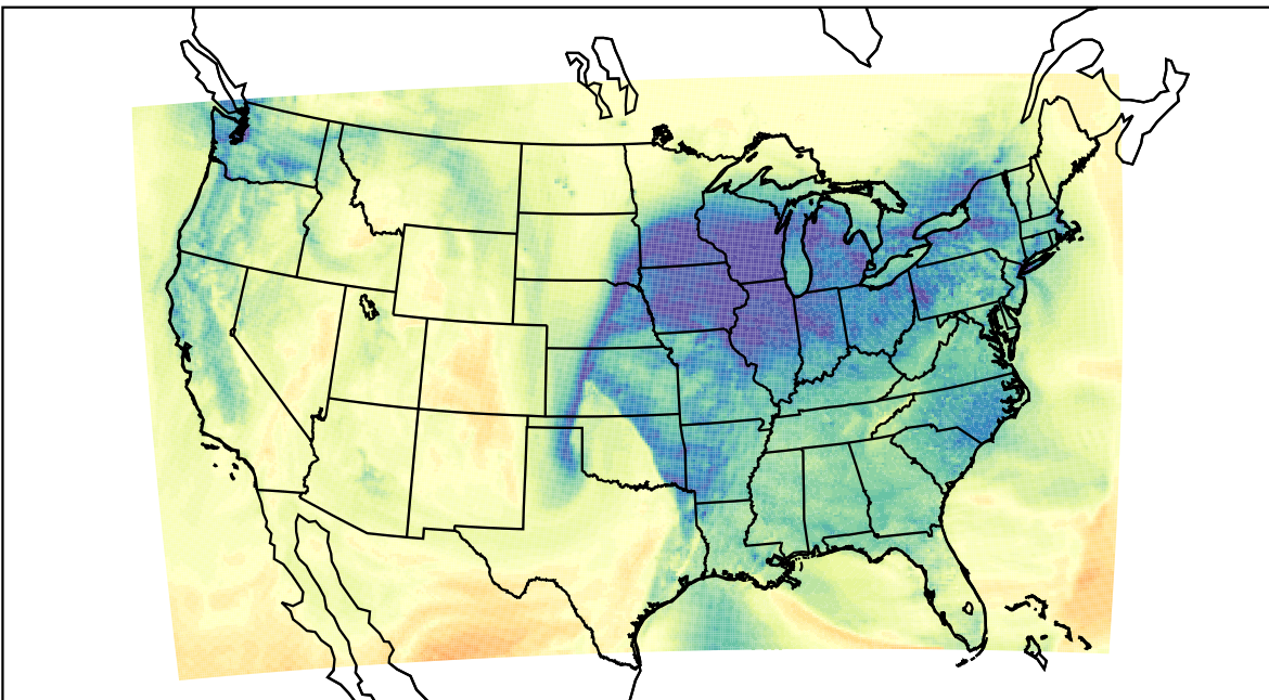
WRF (2024-01-08_22:00:00)
