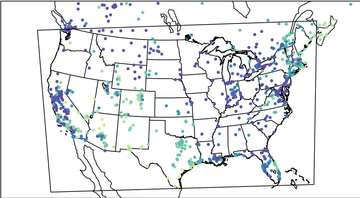
AirNOW (2024-01-08_06:00:00)
