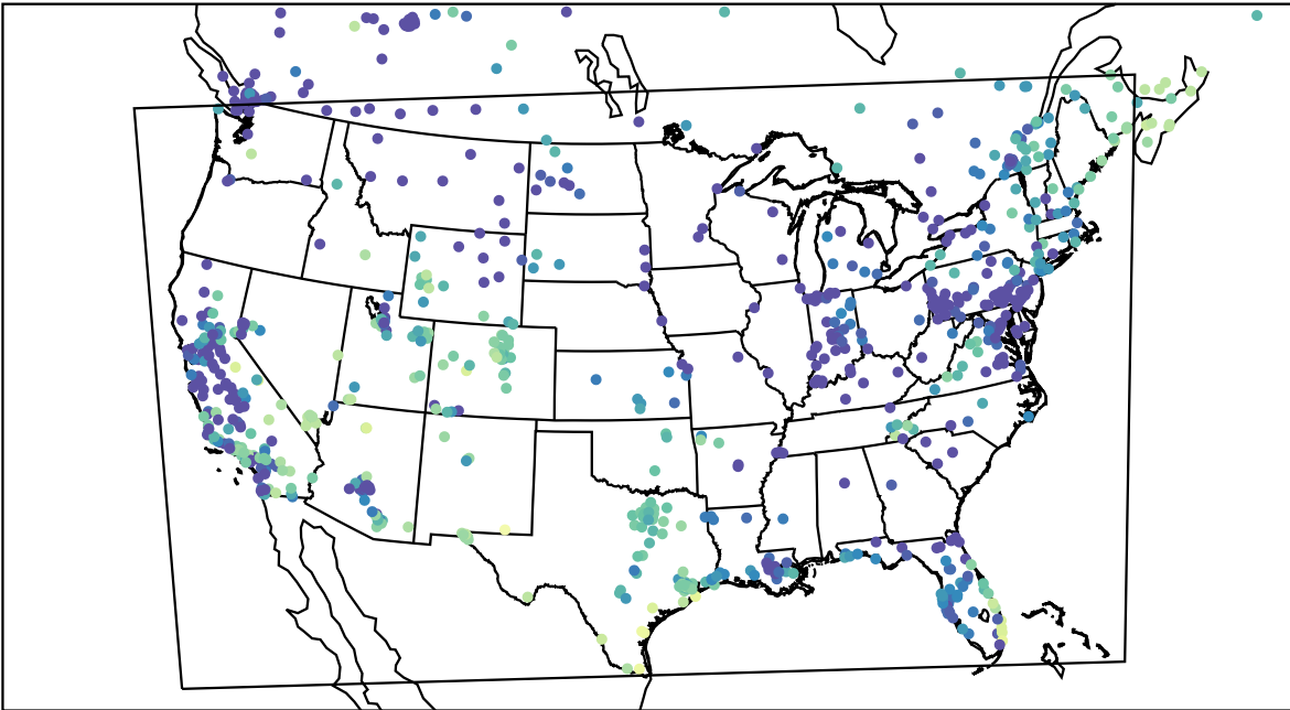
AirNOW (2024-01-08_08:00:00)
