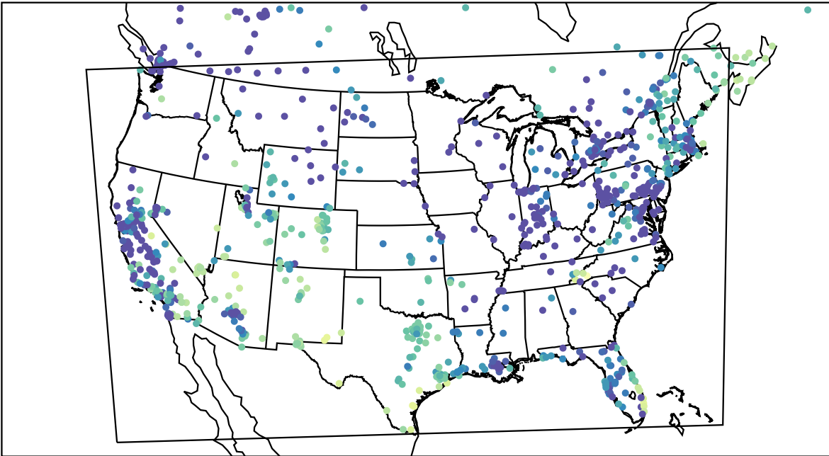
AirNOW (2024-01-08_09:00:00)
