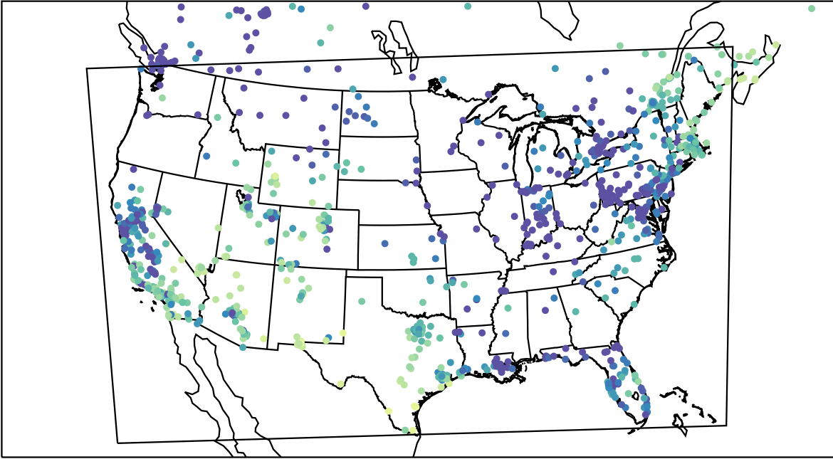
AirNOW (2024-01-08_02:00:00)
