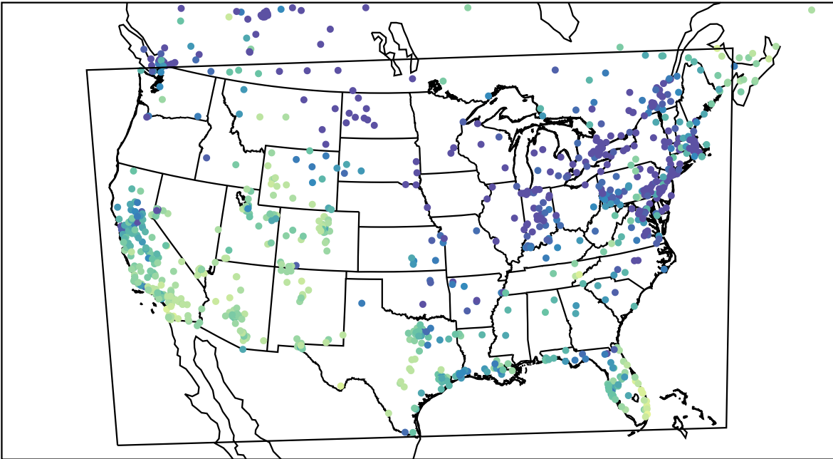
AirNOW (2024-01-08_23:00:00)
