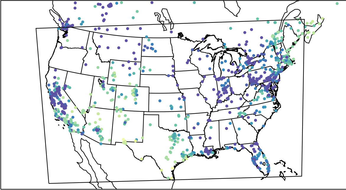
AirNOW (2024-01-08_04:00:00)
