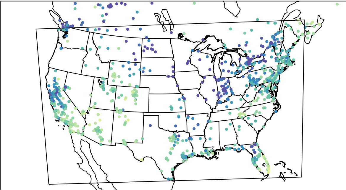
AirNOW (2024-01-08_20:00:00)
