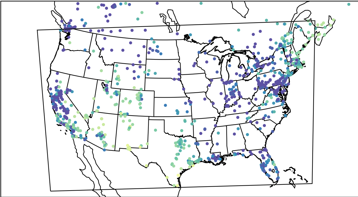
AirNOW (2024-01-08_05:00:00)
