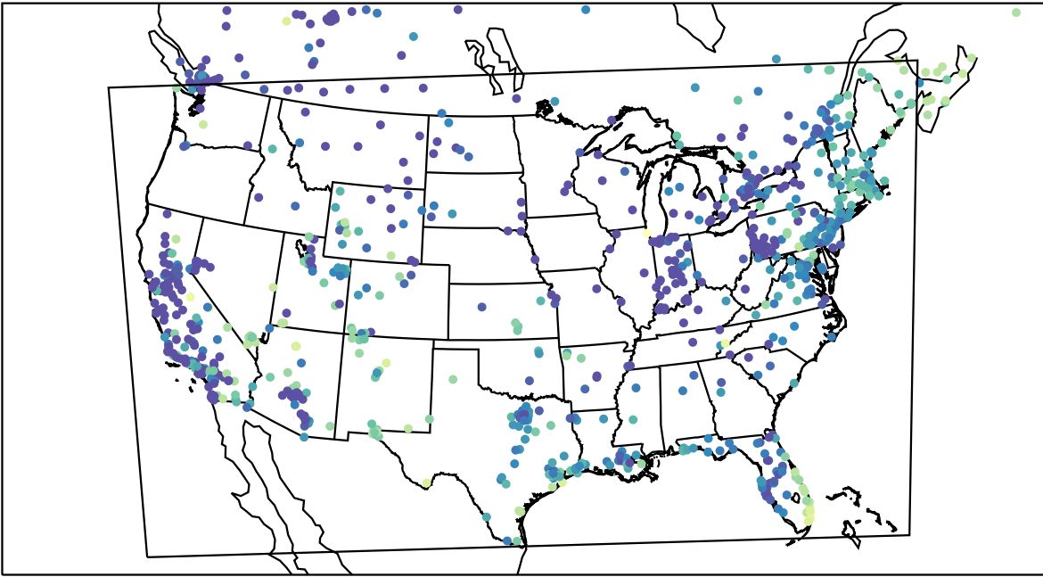
AirNOW (2024-01-08_15:00:00)
