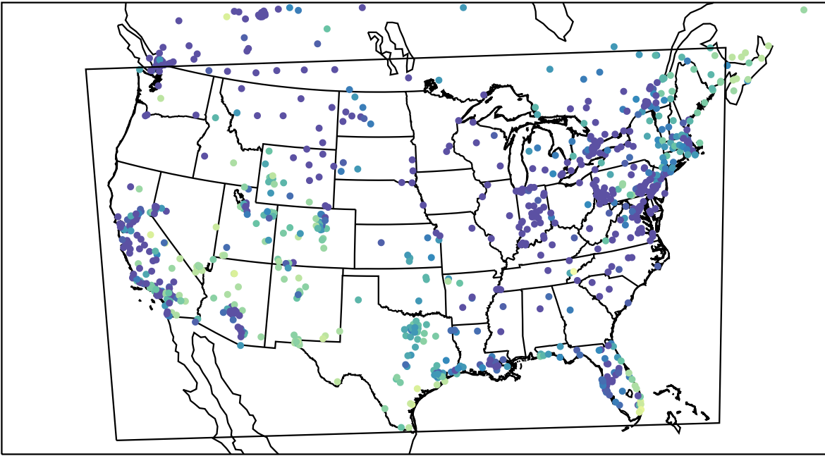
AirNOW (2024-01-08_12:00:00)
