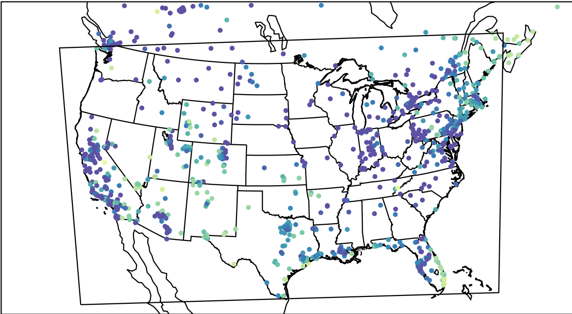
AirNOW (2024-01-08_14:00:00)
