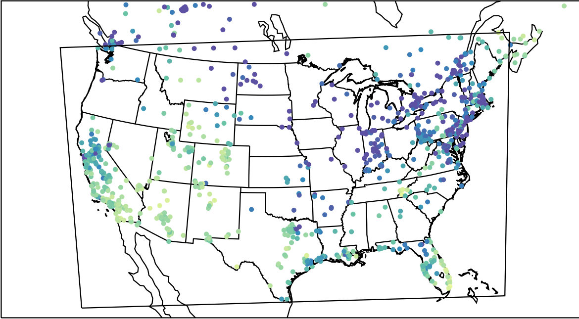
AirNOW (2024-01-08_22:00:00)
