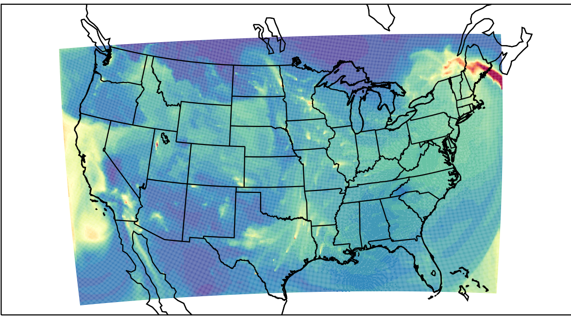
WRF 2024-01-10_17:00:00
