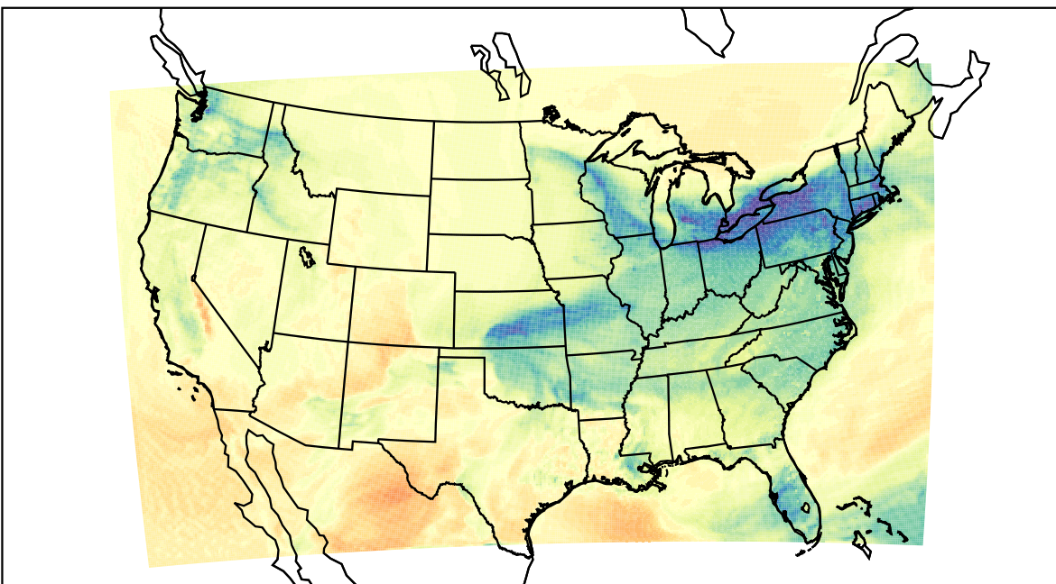
WRF (2024-01-11_21:00:00)
