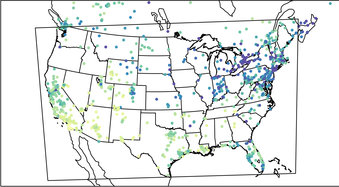
AirNOW (2024-01-11_22:00:00)
