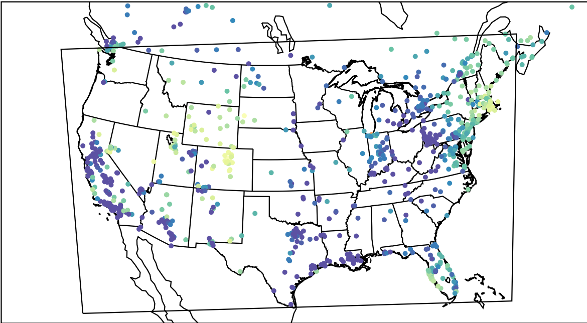
AirNOW (2024-01-10_10:00:00)
