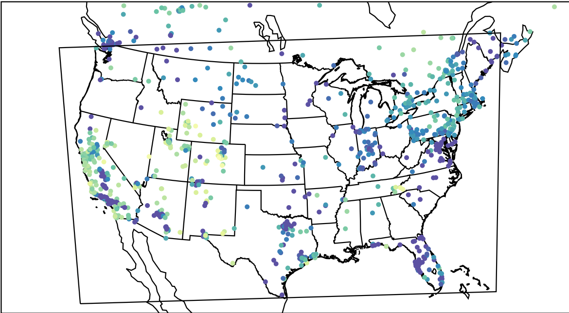
AirNOW (2024-01-11_07:00:00)
