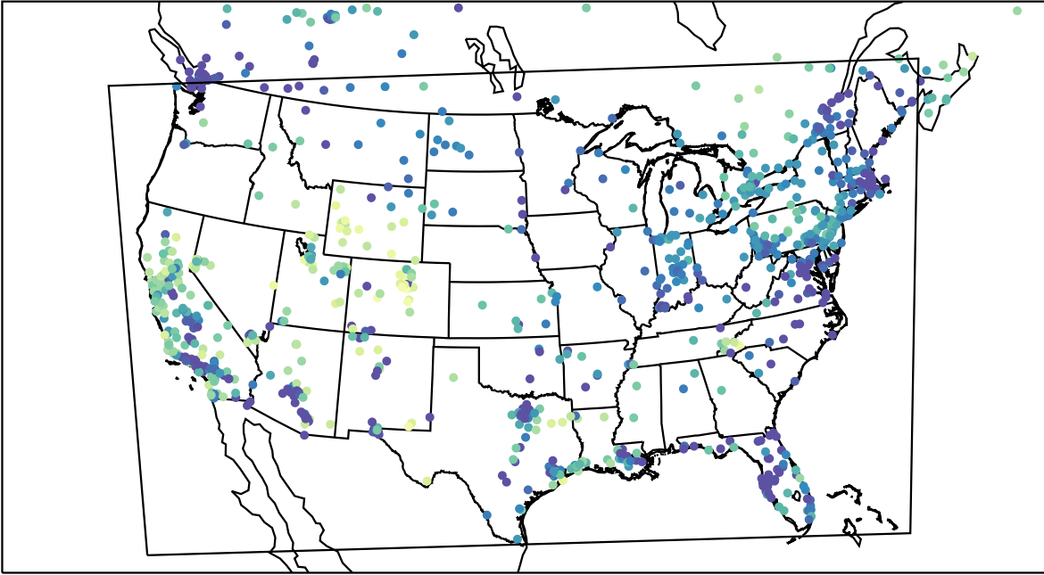
AirNOW (2024-01-11_03:00:00)
