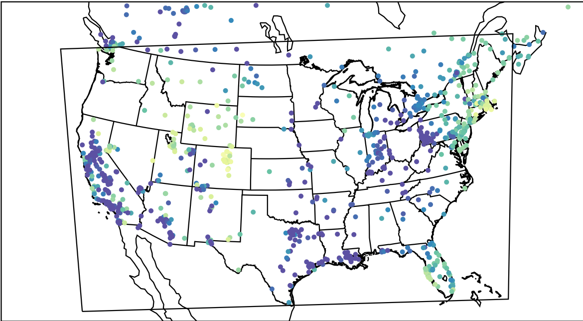
AirNOW (2024-01-10_09:00:00)
