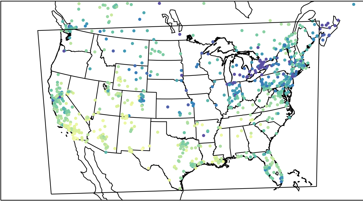
AirNOW (2024-01-11_21:00:00)
