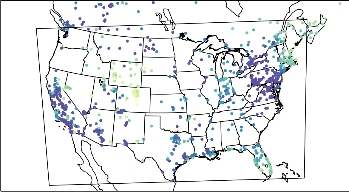
AirNOW (2024-01-10_15:00:00)
