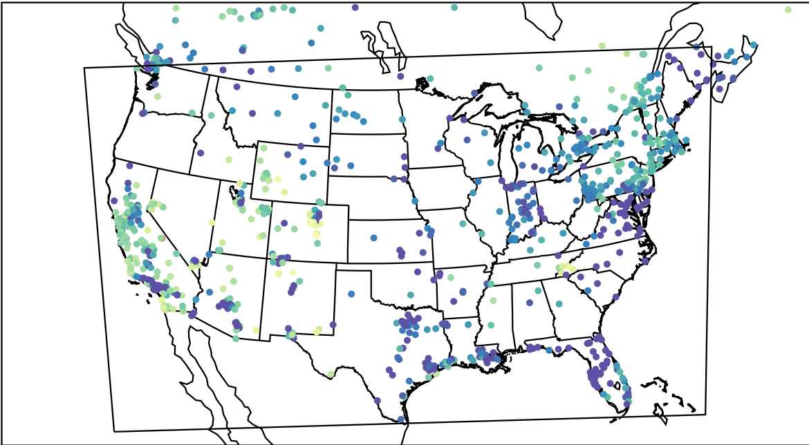
AirNOW (2024-01-11_09:00:00)
