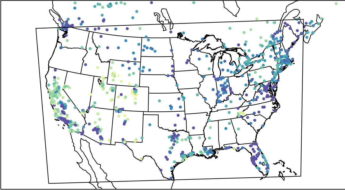
AirNOW (2024-01-11_06:00:00)
