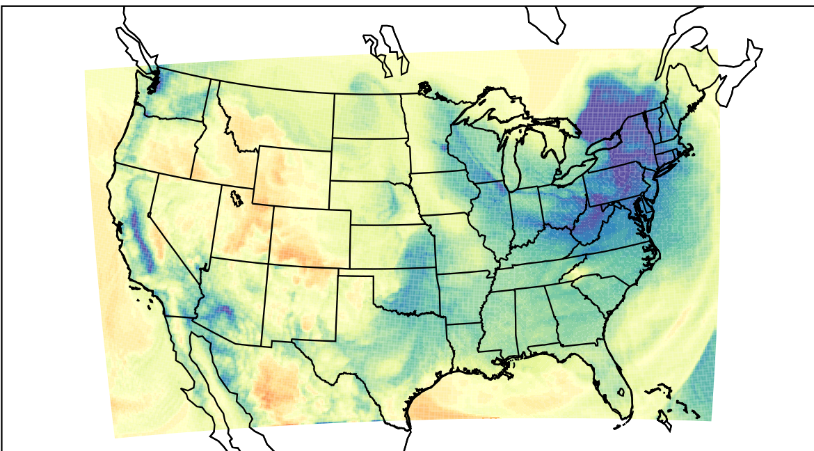
WRF (2024-01-10_17:00:00)
