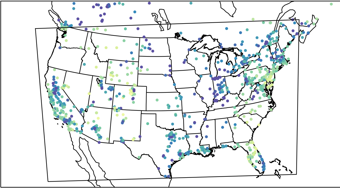
AirNOW (2024-01-10_00:00:00)
