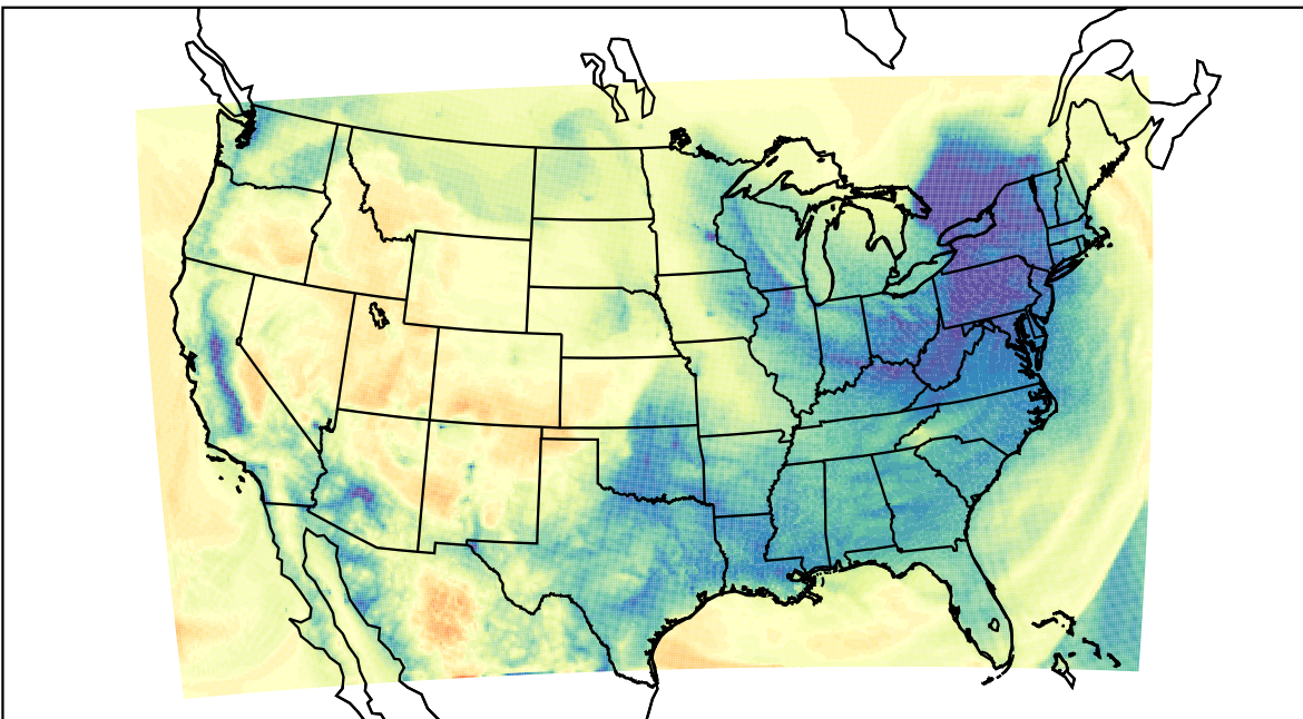
WRF (2024-01-10_15:00:00)
