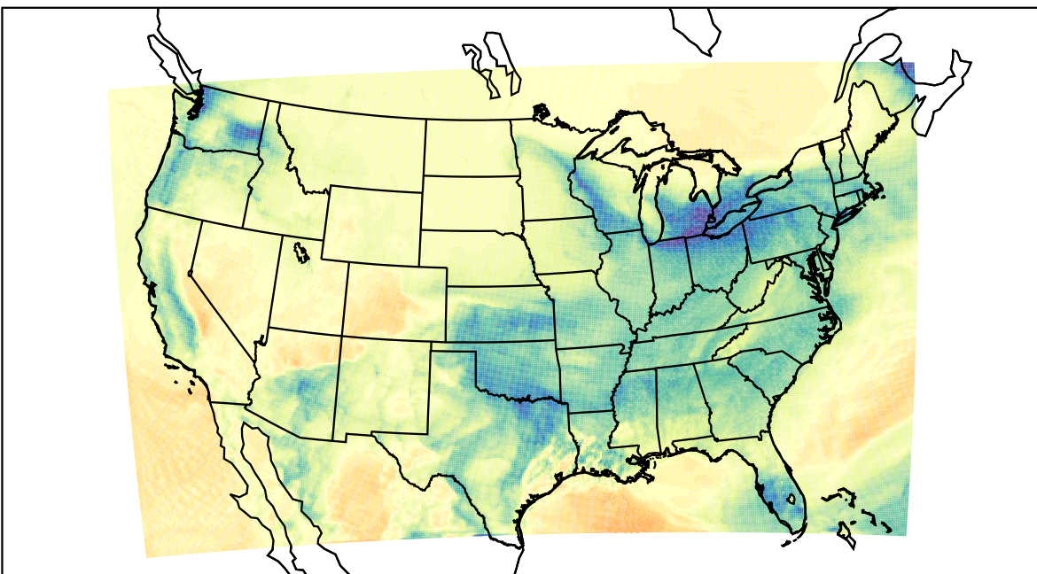
WRF (2024-01-11_17:00:00)
