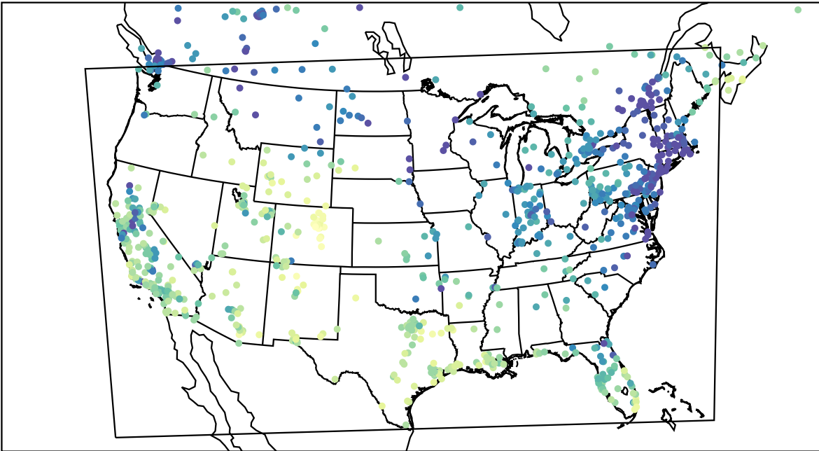
AirNOW (2024-01-10_22:00:00)
