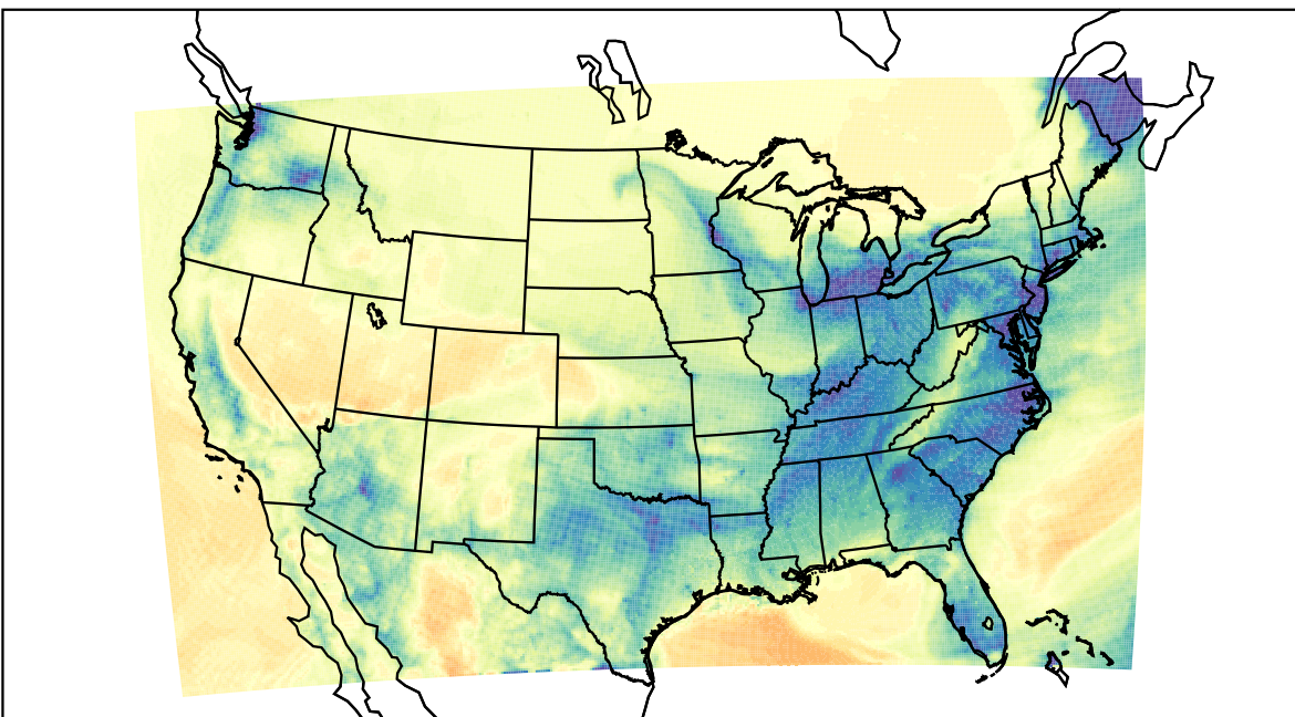
WRF (2024-01-11_12:00:00)
