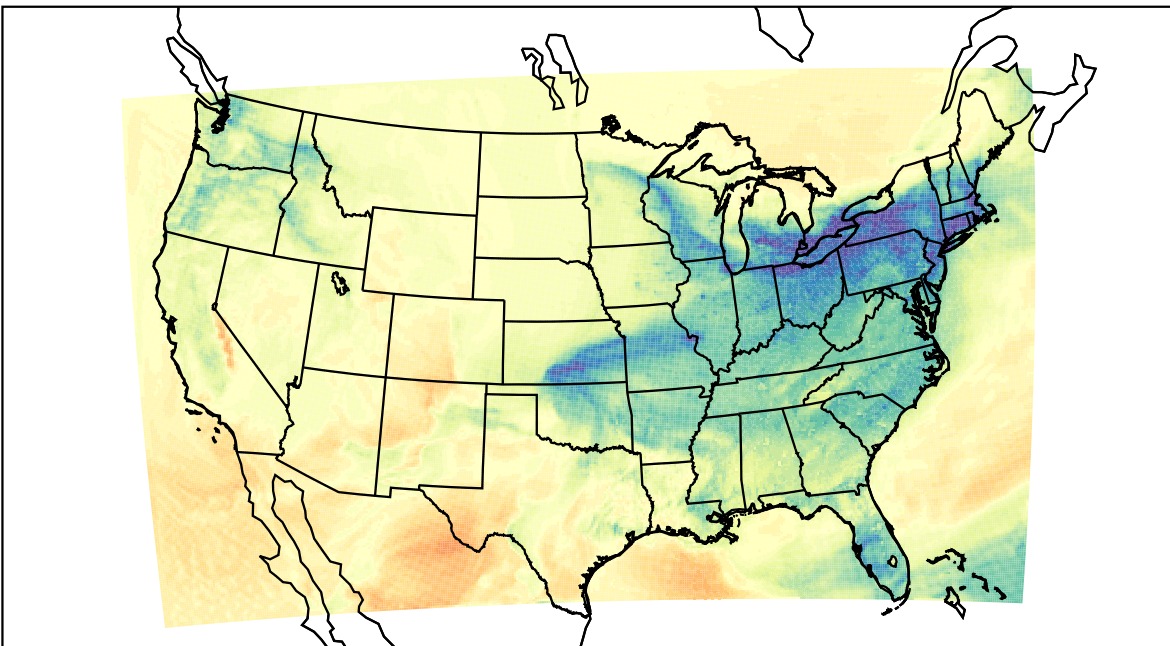
WRF (2024-01-11_22:00:00)
