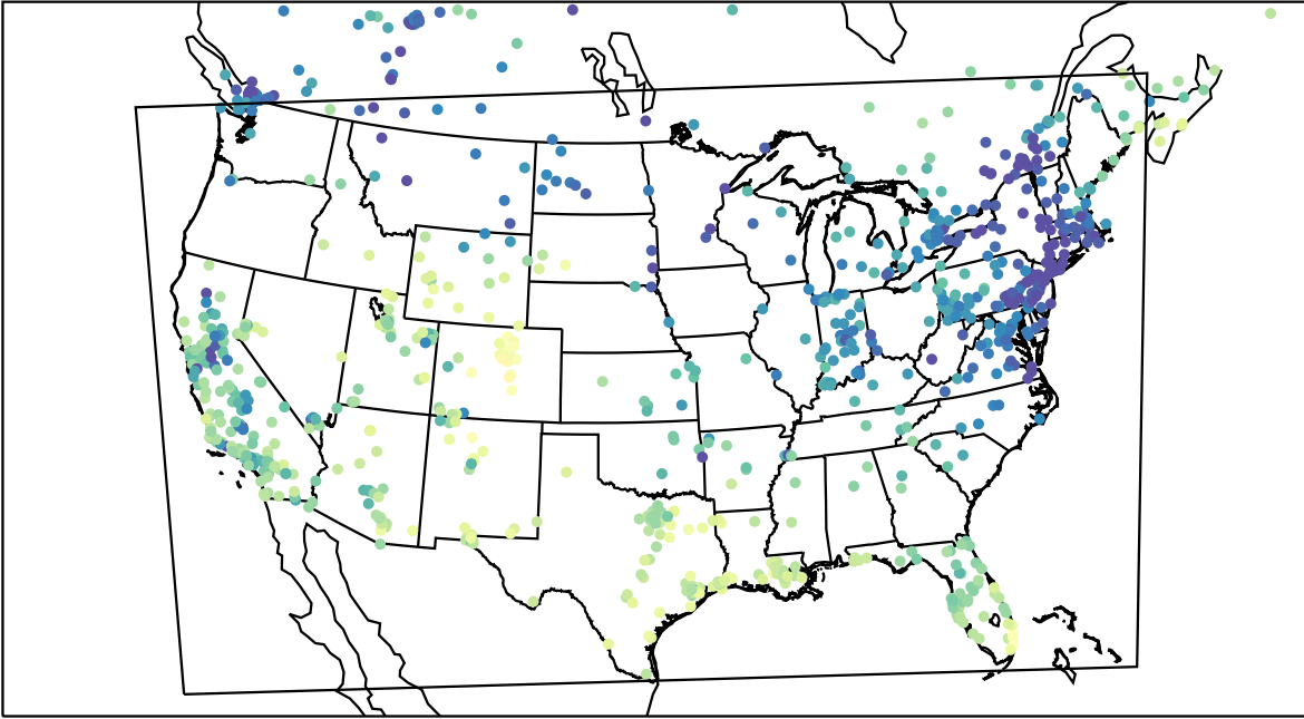
AirNOW (2024-01-10_21:00:00)
