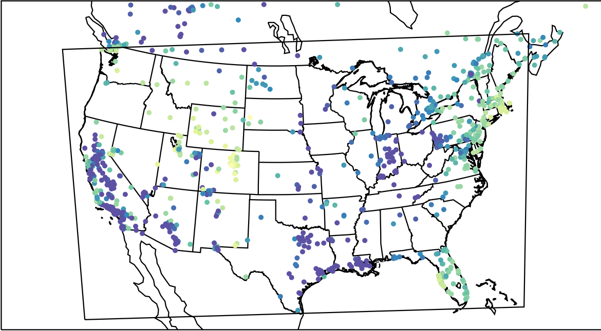
AirNOW (2024-01-10_07:00:00)
