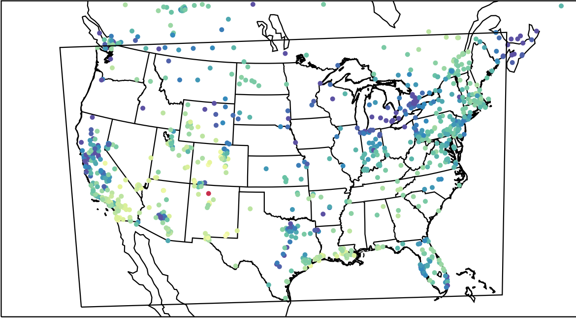
AirNOW (2024-01-11_17:00:00)
