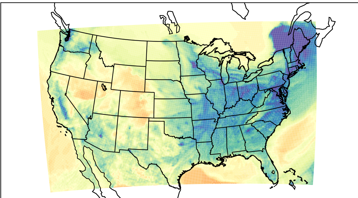
WRF (2024-01-11_02:00:00)
