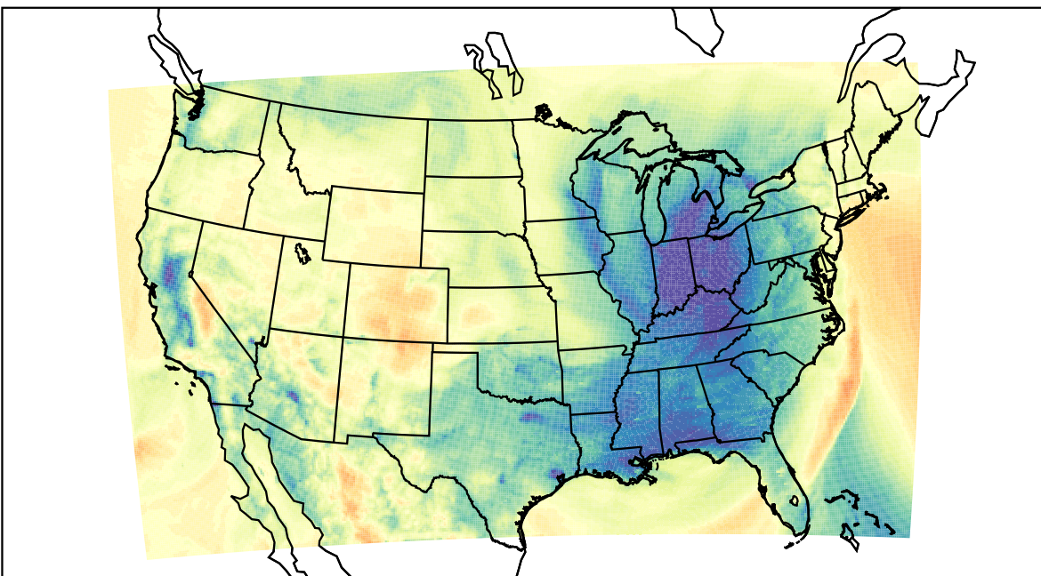
WRF (2024-01-10_06:00:00)
