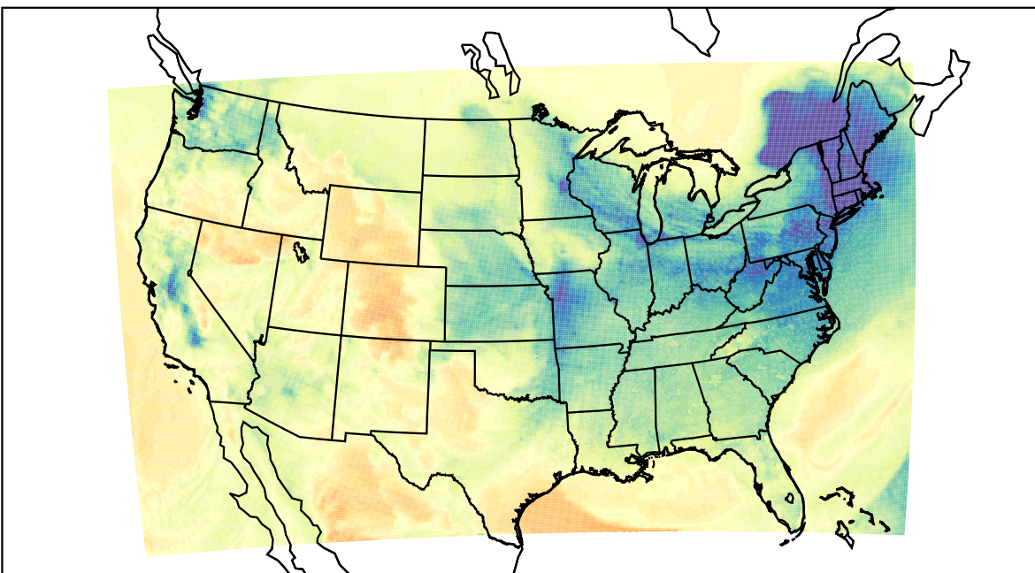
WRF (2024-01-10_22:00:00)
