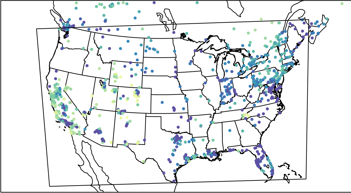
AirNOW (2024-01-11_08:00:00)
