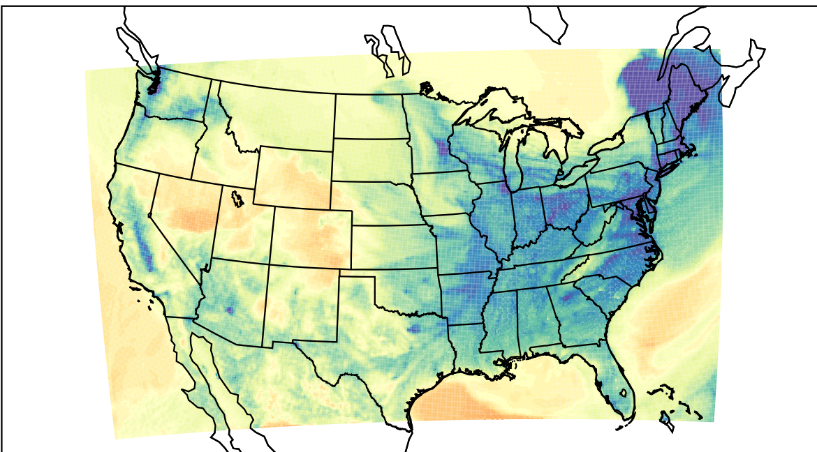
WRF (2024-01-11_03:00:00)
