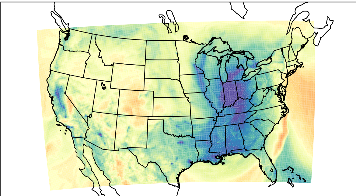
WRF (2024-01-10_04:00:00)
