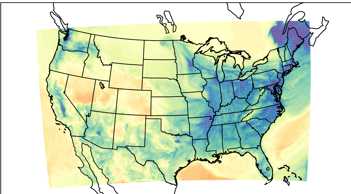
WRF (2024-01-11_05:00:00)
