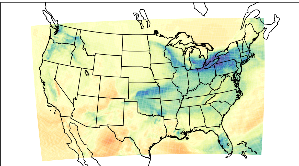
WRF (2024-01-11_20:00:00)
