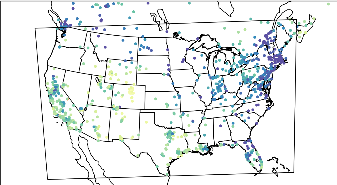
AirNOW (2024-01-10_23:00:00)
