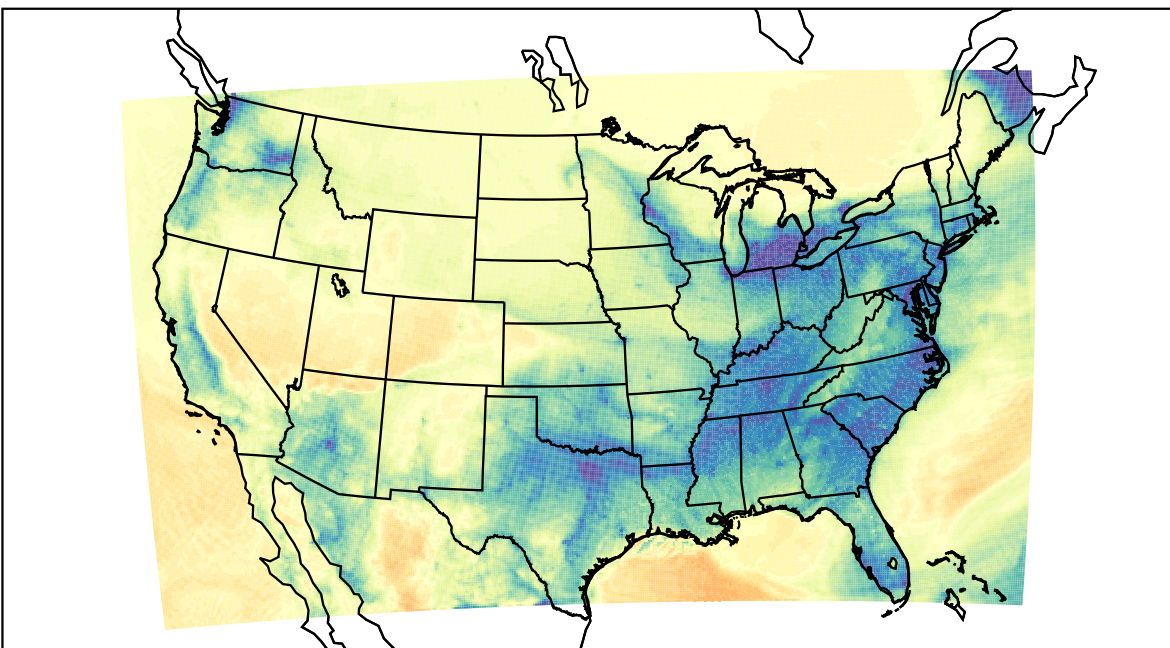
WRF (2024-01-11_14:00:00)
