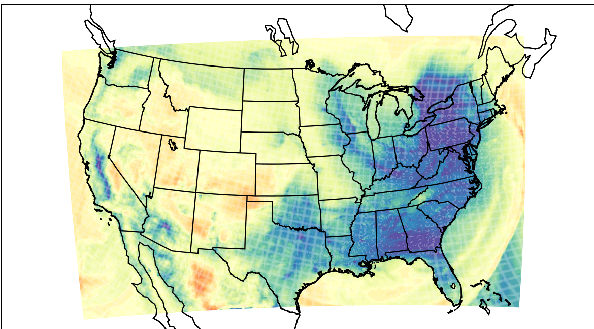
WRF (2024-01-10_13:00:00)
