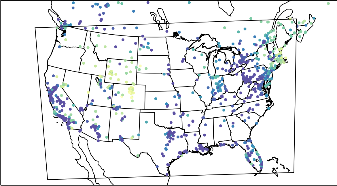
AirNOW (2024-01-10_12:00:00)
