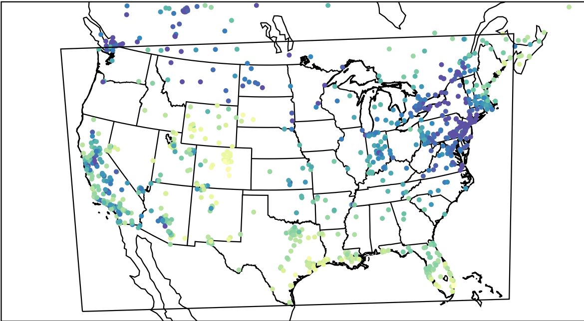
AirNOW (2024-01-10_19:00:00)
