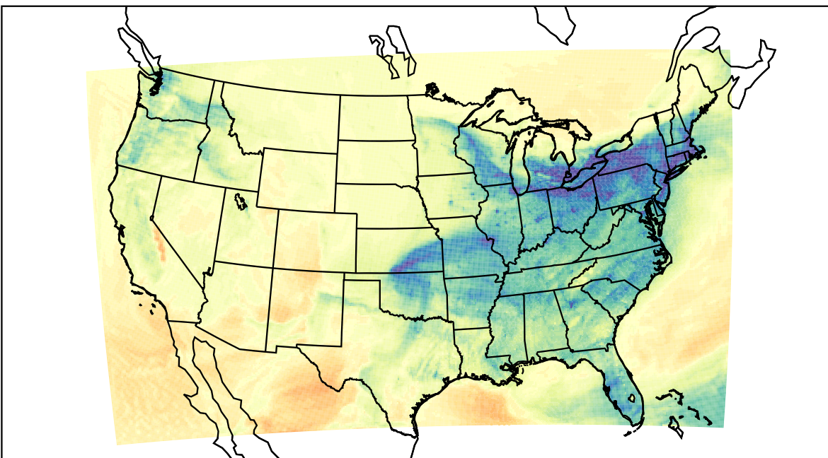
WRF (2024-01-11_23:00:00)
