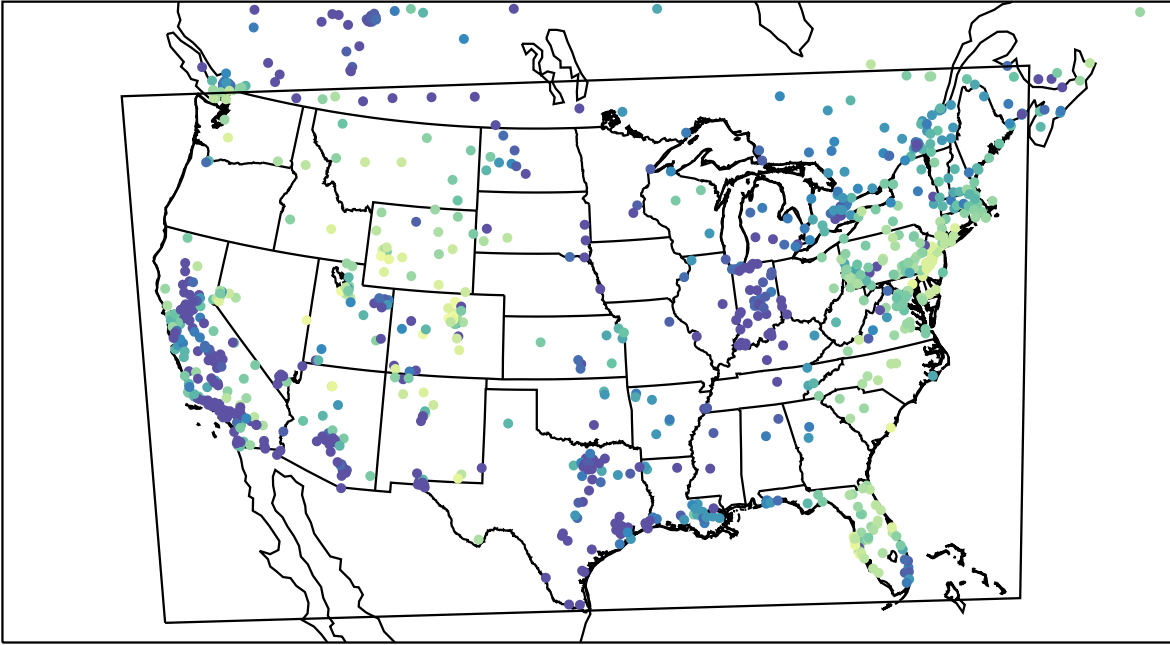
AirNOW (2024-01-10_02:00:00)
