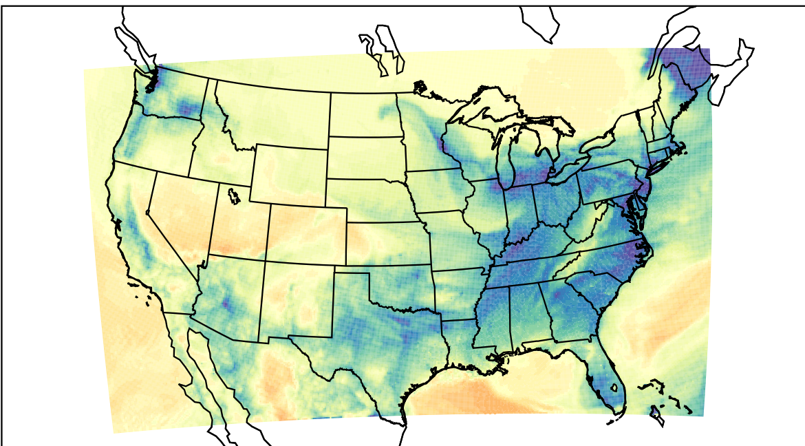
WRF (2024-01-11_11:00:00)
