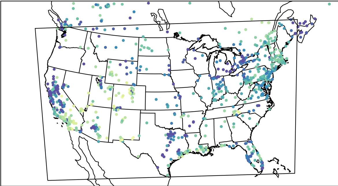
AirNOW (2024-01-11_16:00:00)
