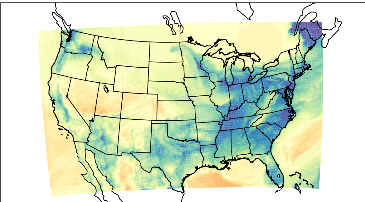
WRF (2024-01-11_10:00:00)
