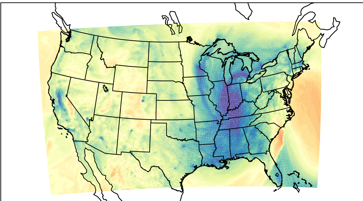
WRF (2024-01-10_01:00:00)
