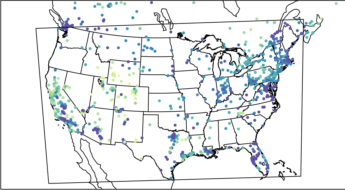
AirNOW (2024-01-11_04:00:00)
