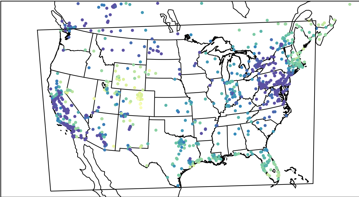
AirNOW (2024-01-10_16:00:00)
