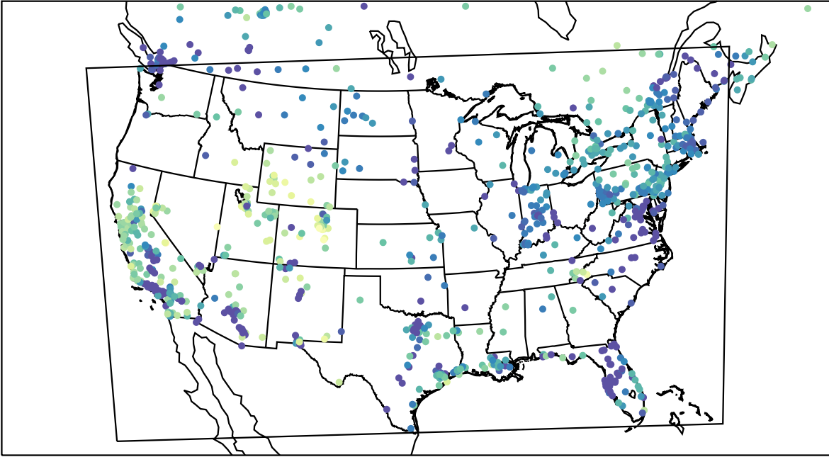
AirNOW (2024-01-11_05:00:00)
