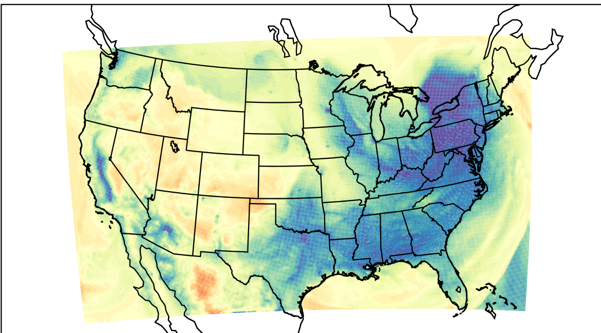
WRF (2024-01-10_14:00:00)
