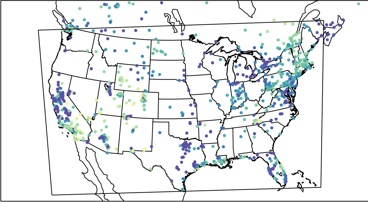
AirNOW (2024-01-11_15:00:00)
