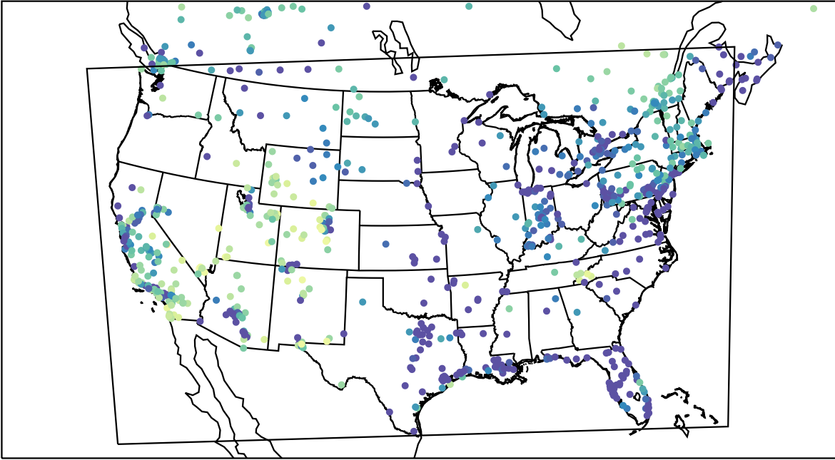
AirNOW (2024-01-11_12:00:00)
