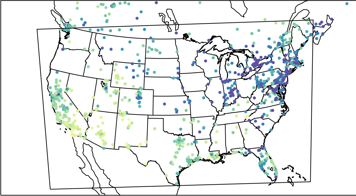
AirNOW (2024-01-11_23:00:00)
