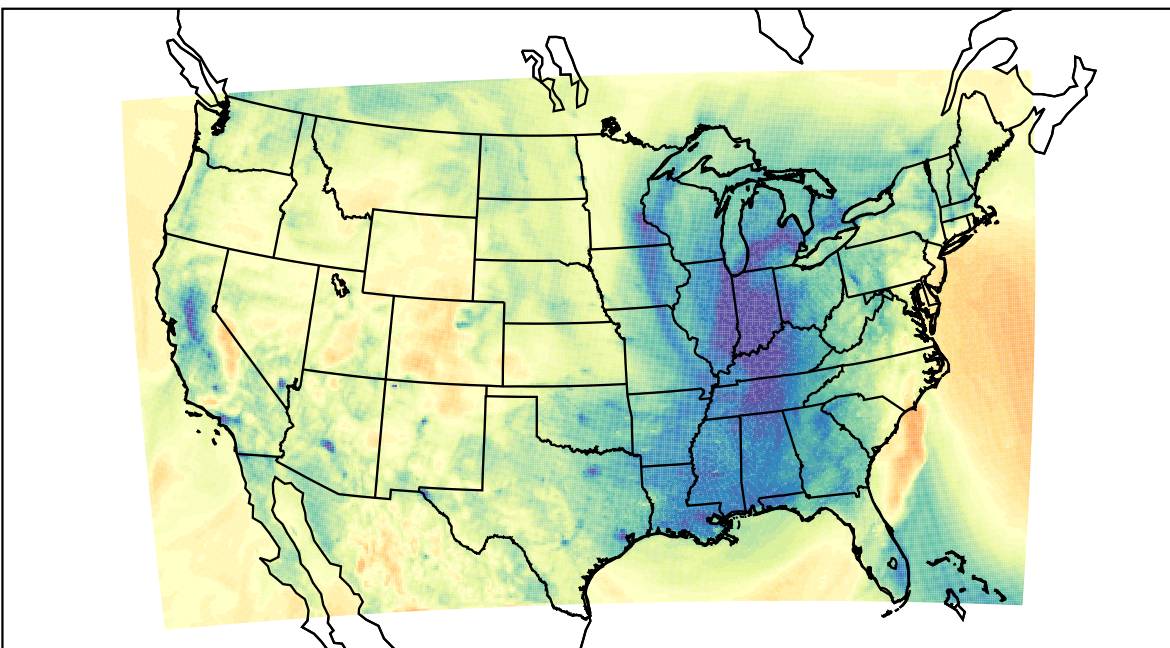
WRF (2024-01-10_02:00:00)
