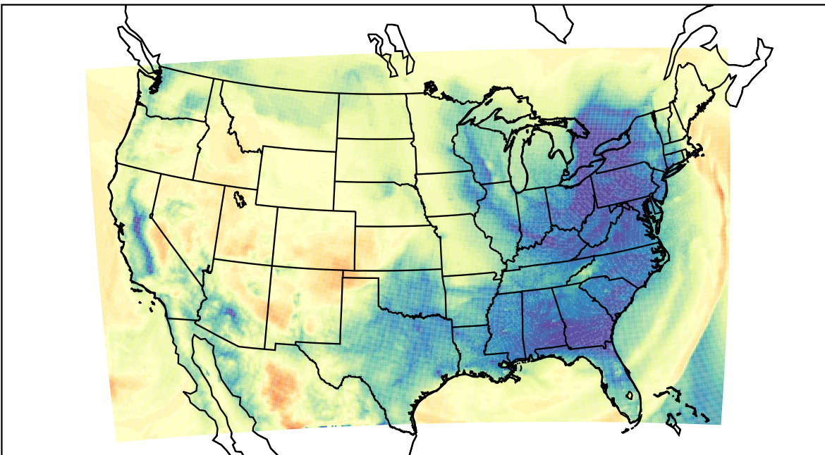
WRF (2024-01-10_12:00:00)
