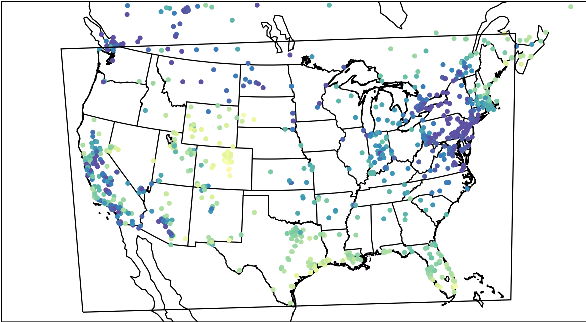
AirNOW (2024-01-10_18:00:00)
