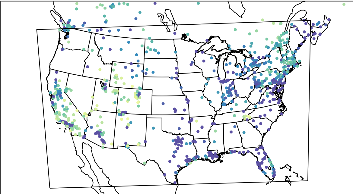
AirNOW (2024-01-11_11:00:00)
