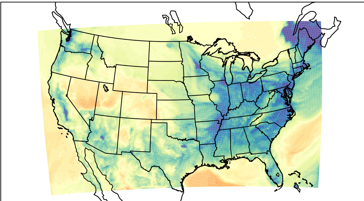
WRF (2024-01-11_06:00:00)
