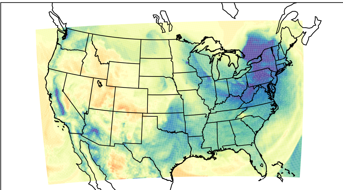
WRF (2024-01-10_16:00:00)
