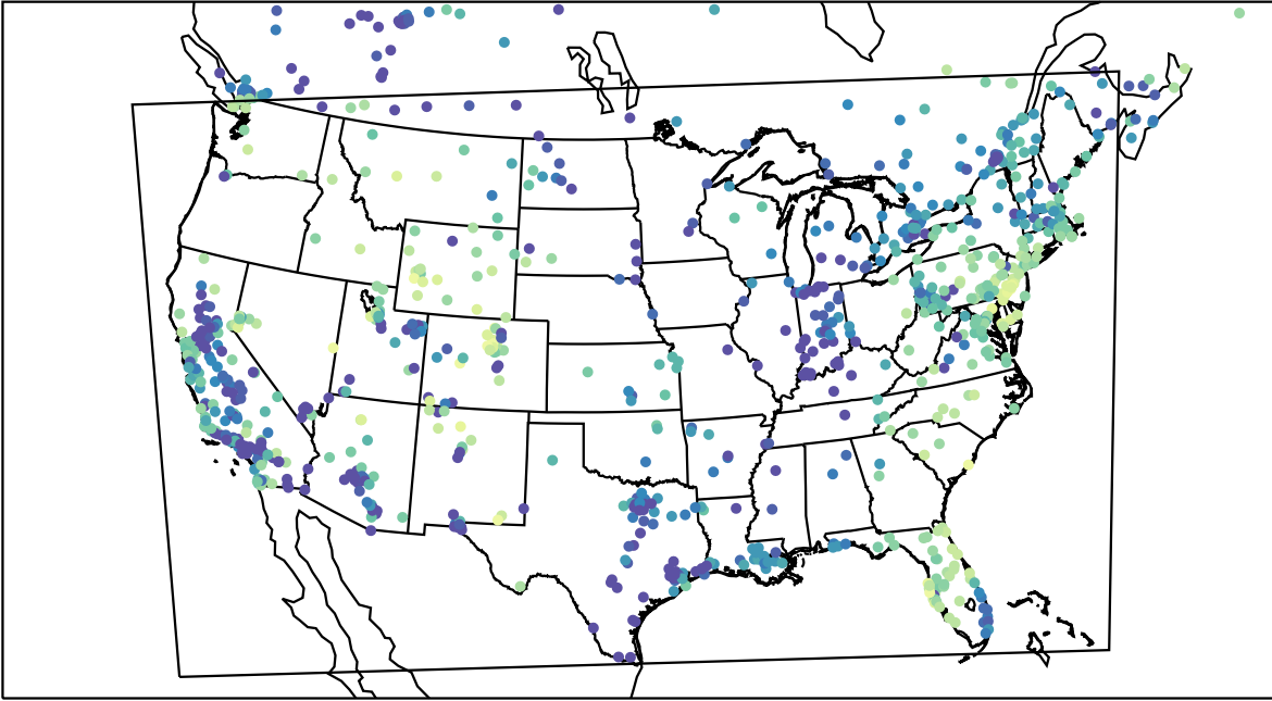
AirNOW (2024-01-10_01:00:00)
