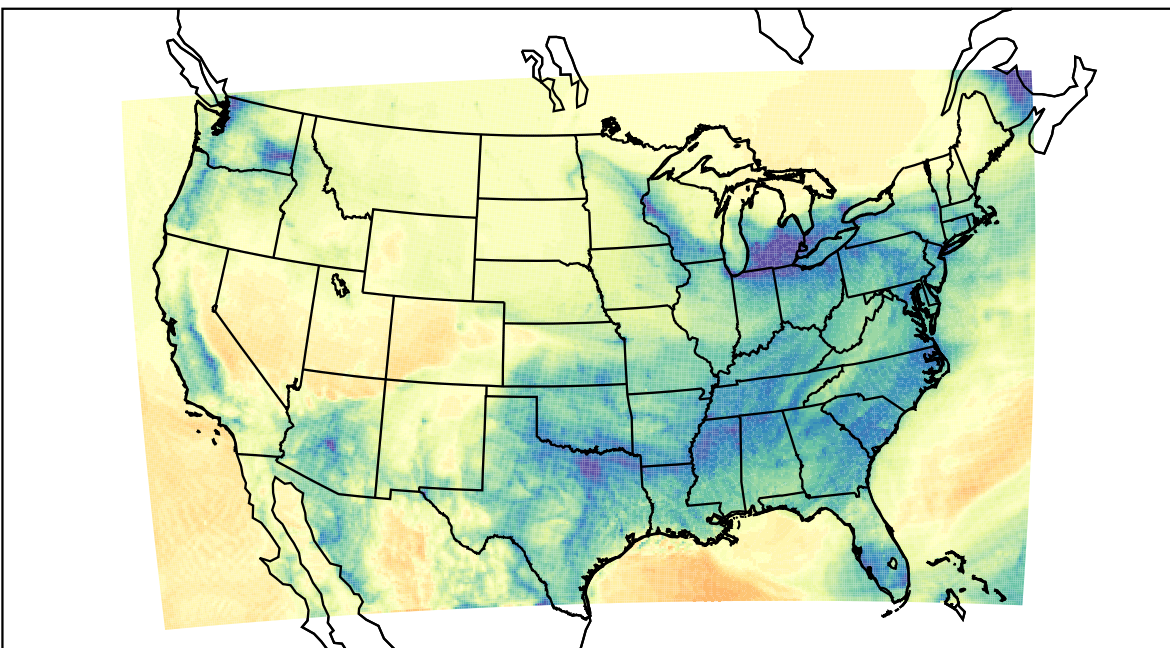
WRF (2024-01-11_15:00:00)
