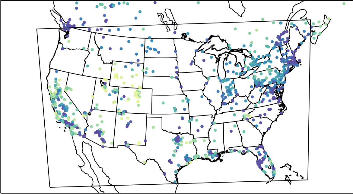
AirNOW (2024-01-11_02:00:00)
