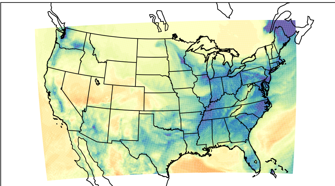
WRF (2024-01-11_09:00:00)
