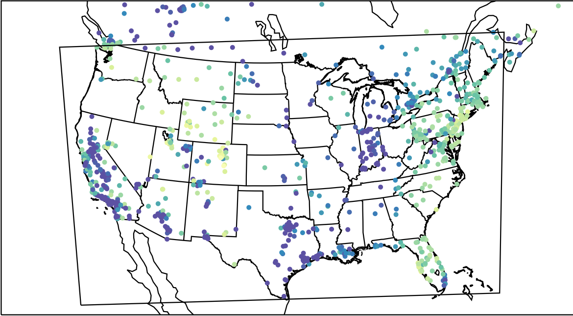
AirNOW (2024-01-10_03:00:00)
