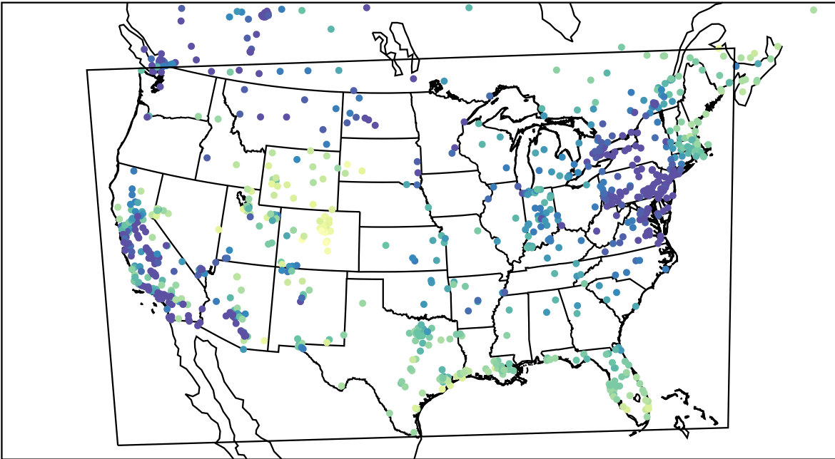
AirNOW (2024-01-10_17:00:00)
