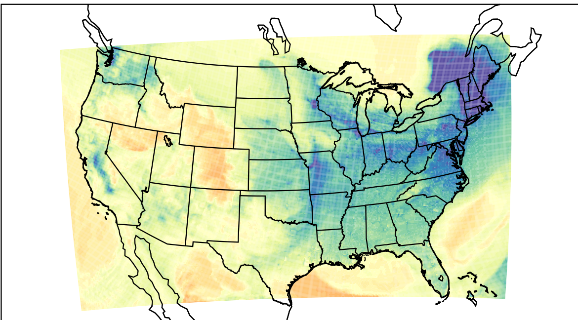
WRF (2024-01-10_23:00:00)
