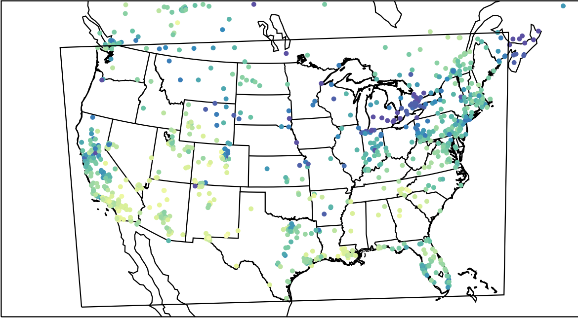
AirNOW (2024-01-11_19:00:00)
