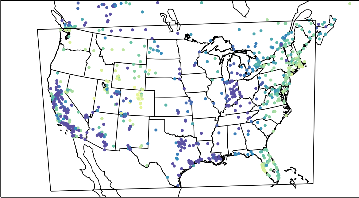
AirNOW (2024-01-10_06:00:00)
