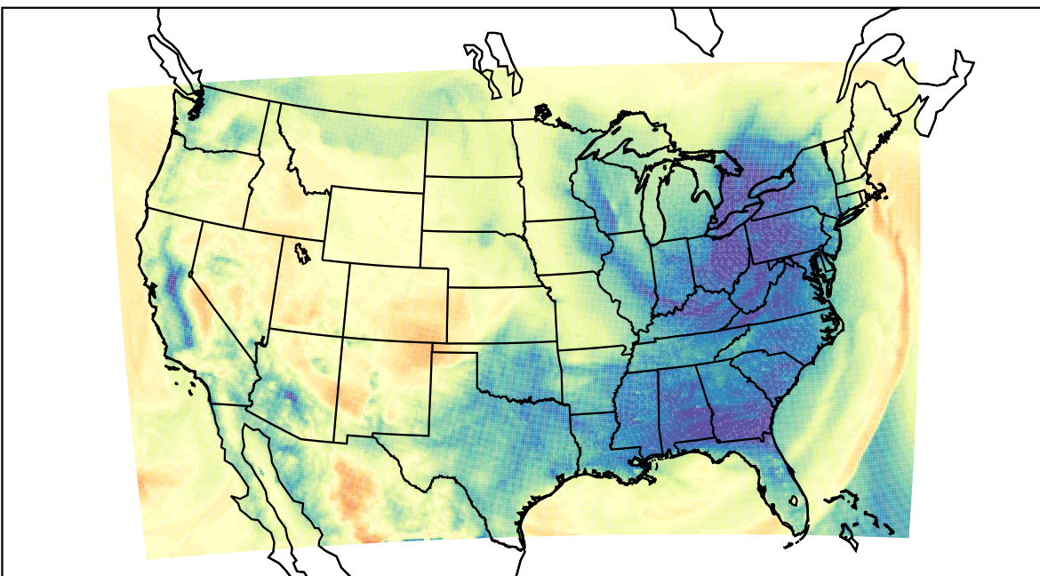
WRF (2024-01-10_11:00:00)
