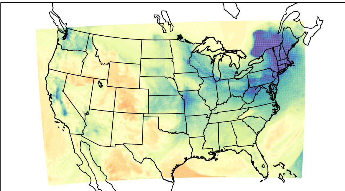
WRF (2024-01-10_21:00:00)
