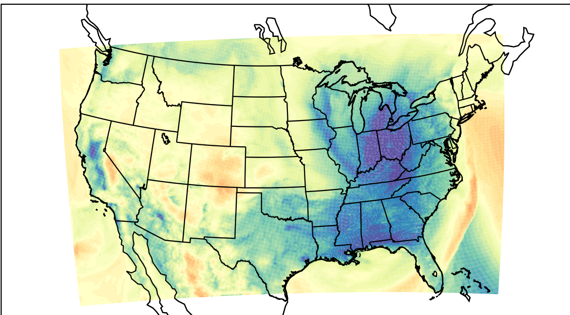
WRF (2024-01-10_07:00:00)
