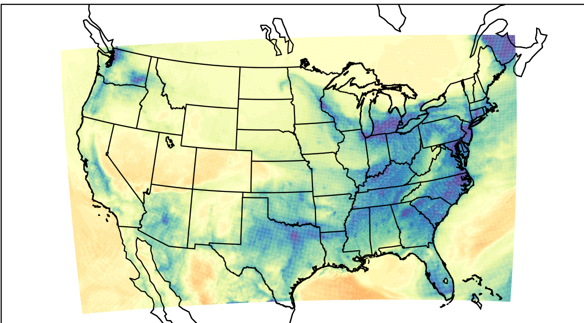
WRF (2024-01-11_13:00:00)
