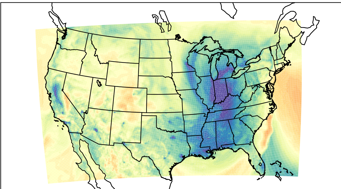
WRF (2024-01-10_03:00:00)
