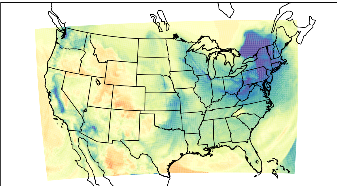
WRF (2024-01-10_18:00:00)
