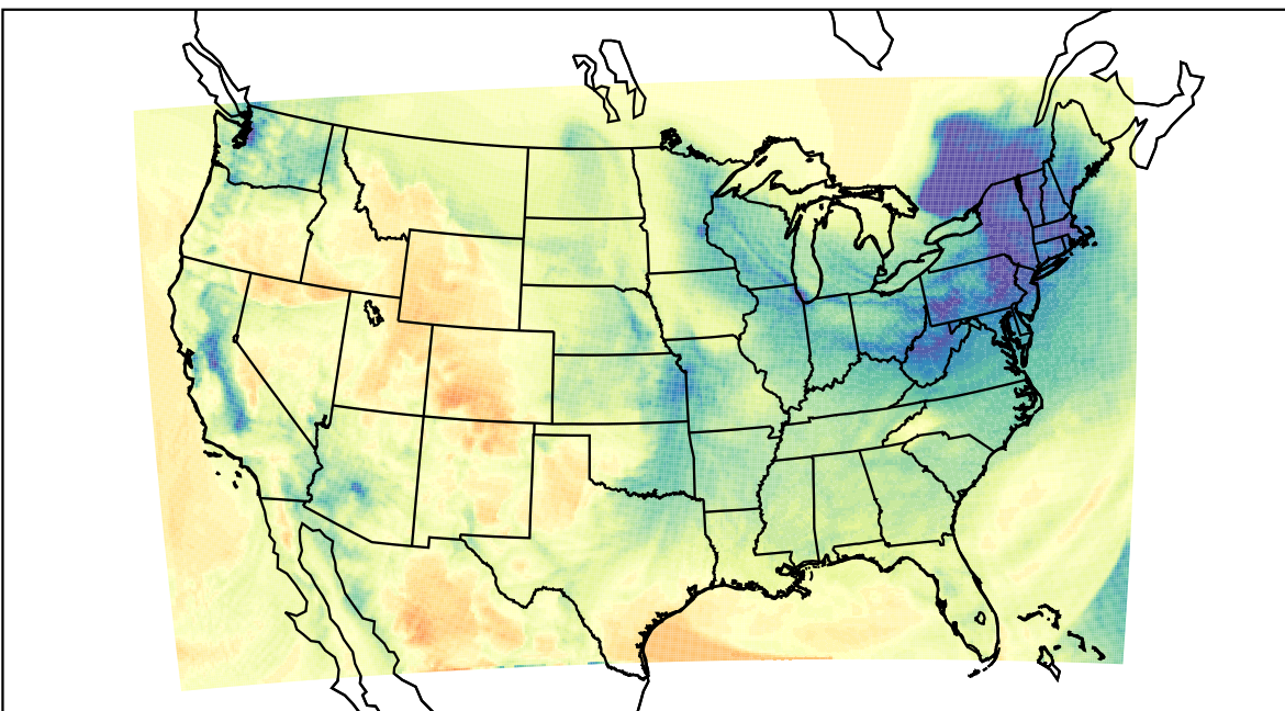
WRF (2024-01-10_19:00:00)
