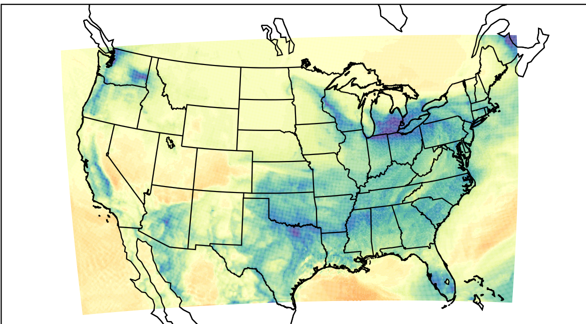
WRF (2024-01-11_16:00:00)
