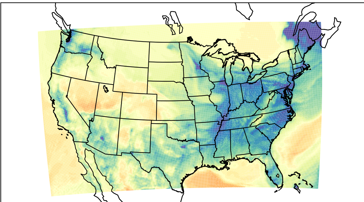
WRF (2024-01-11_07:00:00)
