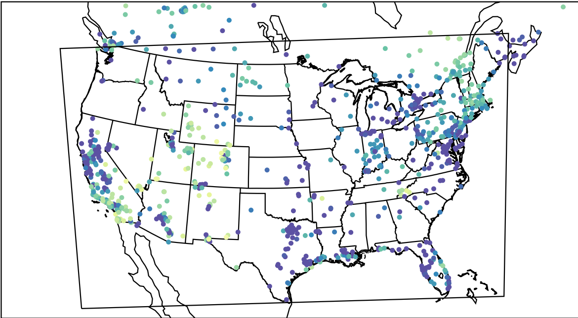
AirNOW (2024-01-11_14:00:00)
