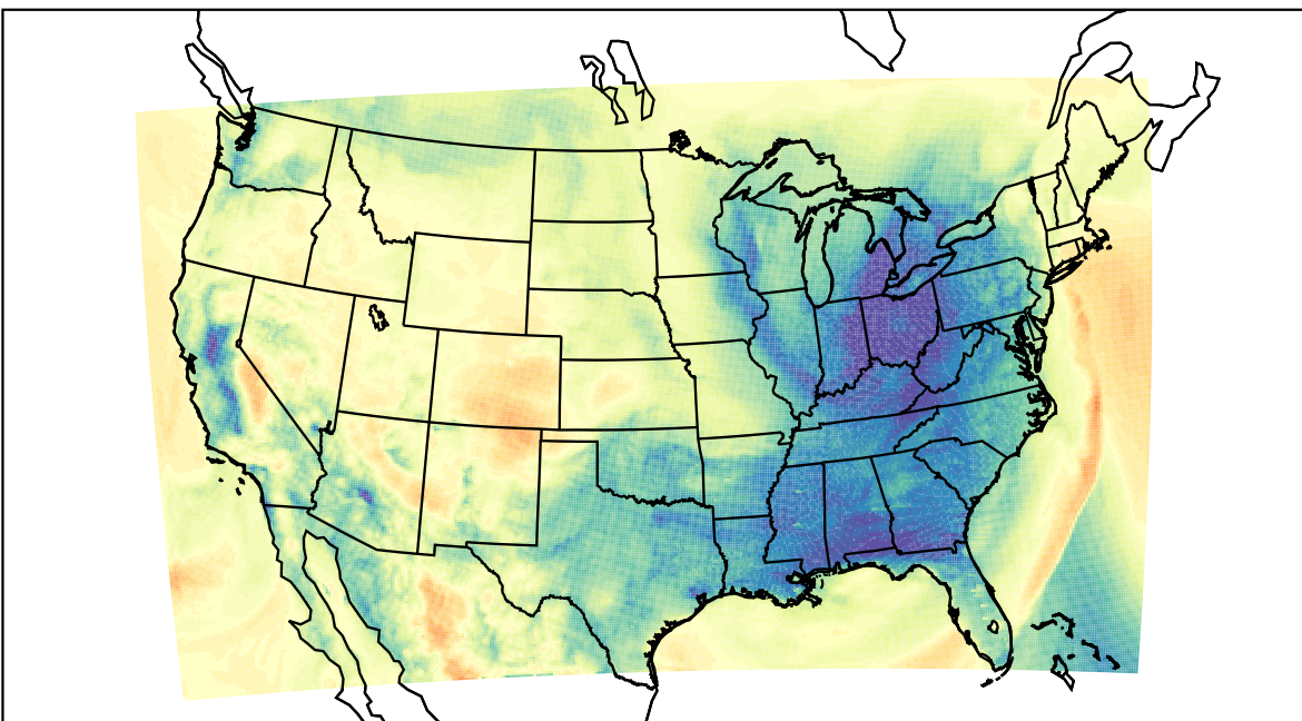
WRF (2024-01-10_08:00:00)
