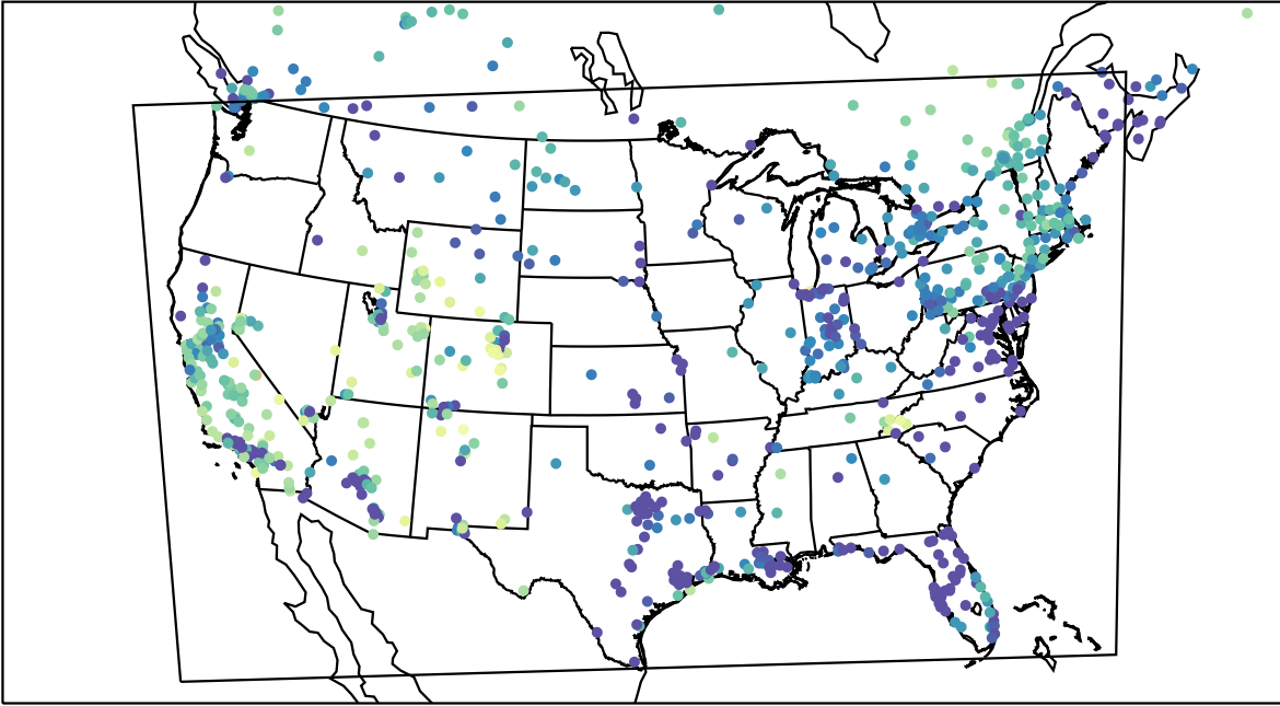
AirNOW (2024-01-11_10:00:00)
