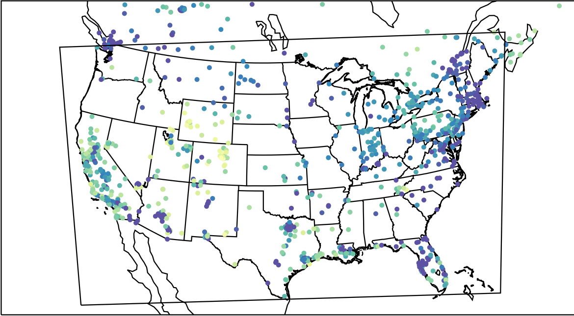
AirNOW (2024-01-11_01:00:00)
