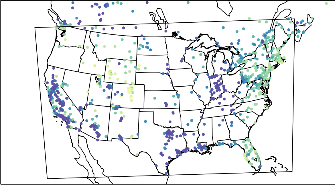
AirNOW (2024-01-10_05:00:00)
