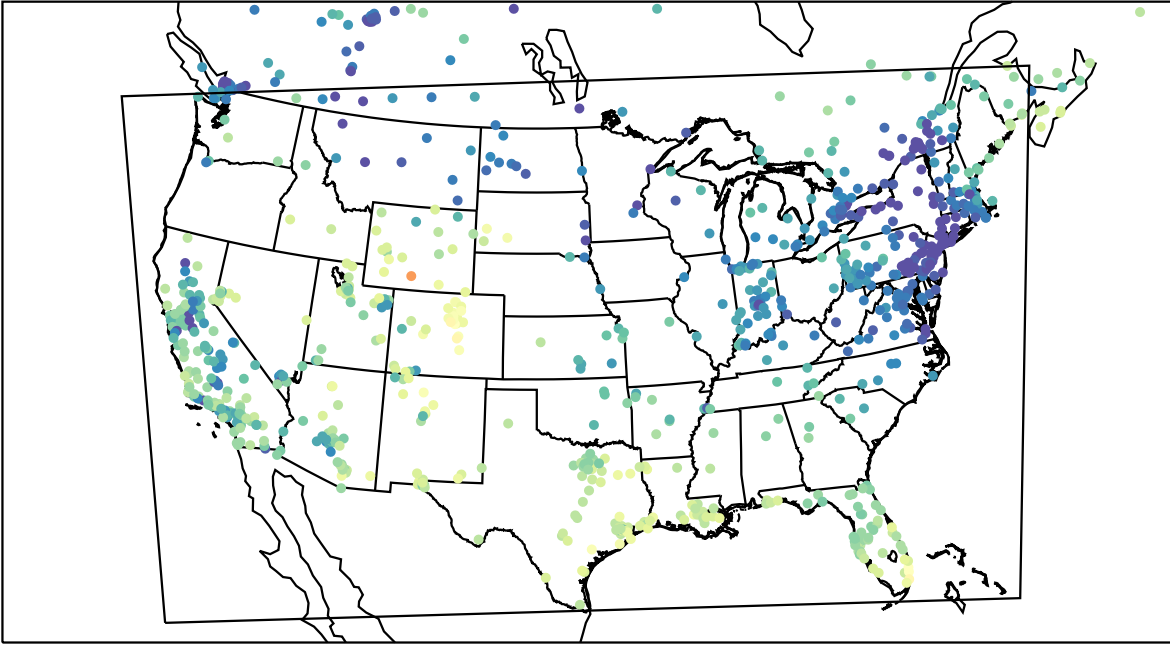
AirNOW (2024-01-10_20:00:00)
