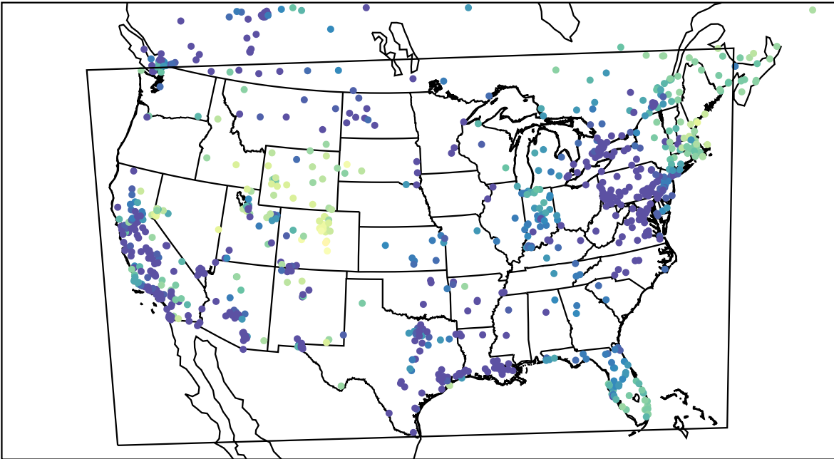
AirNOW (2024-01-10_14:00:00)
