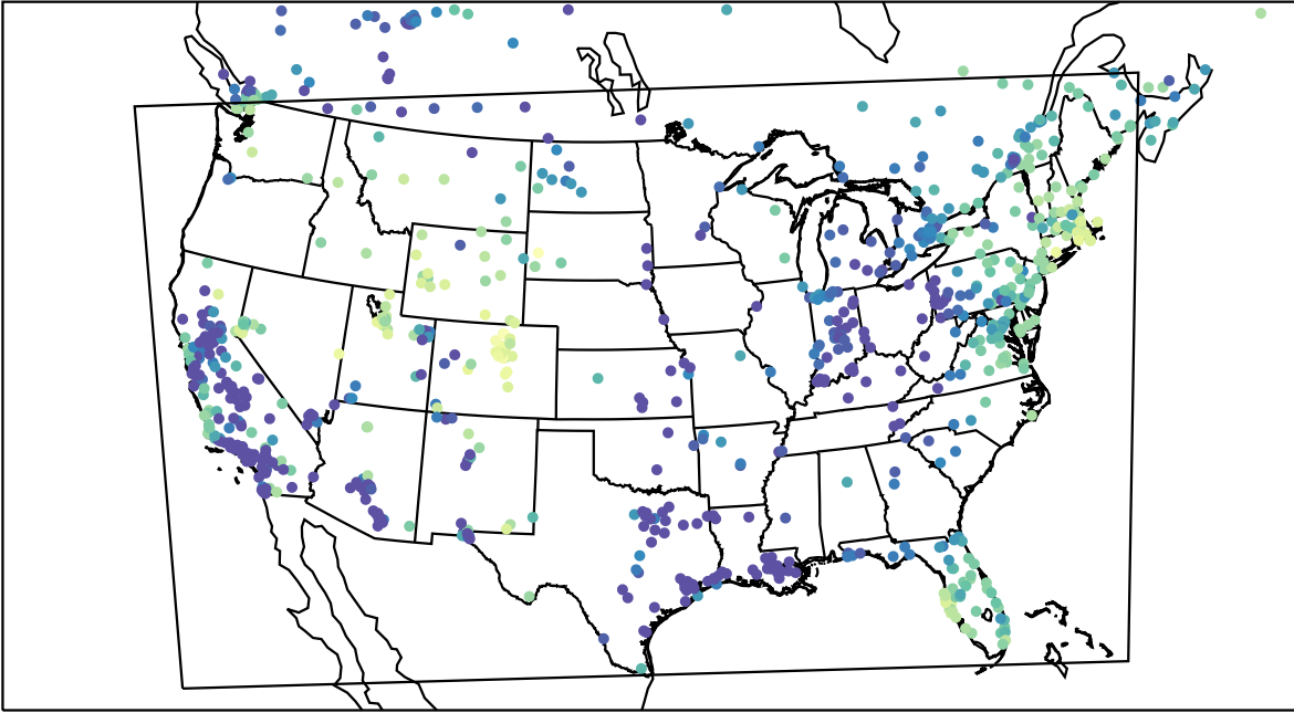
AirNOW (2024-01-10_08:00:00)
