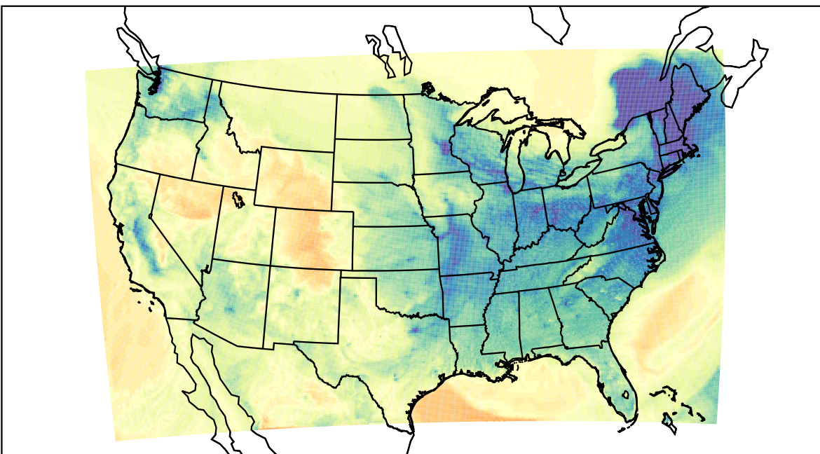
WRF (2024-01-11_00:00:00)
