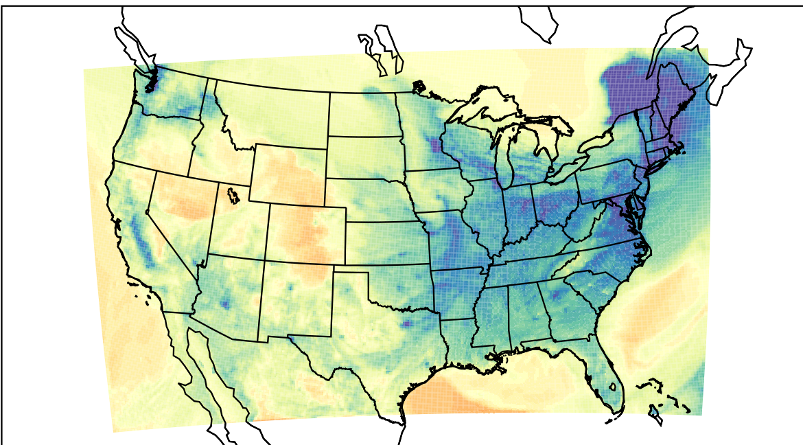
WRF (2024-01-11_01:00:00)
