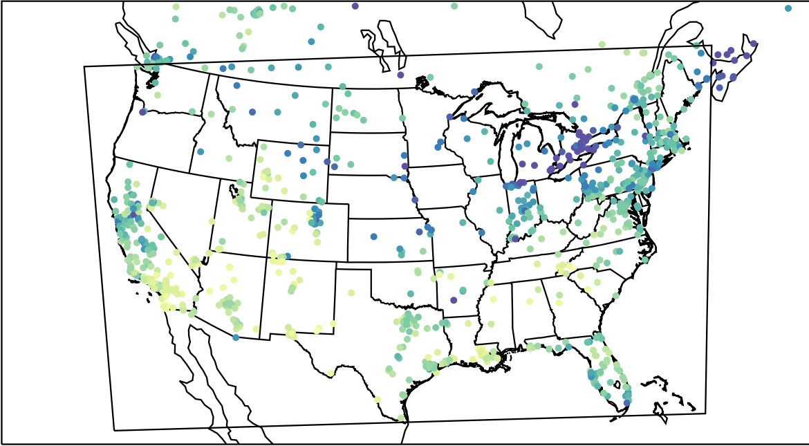
AirNOW (2024-01-11_20:00:00)
