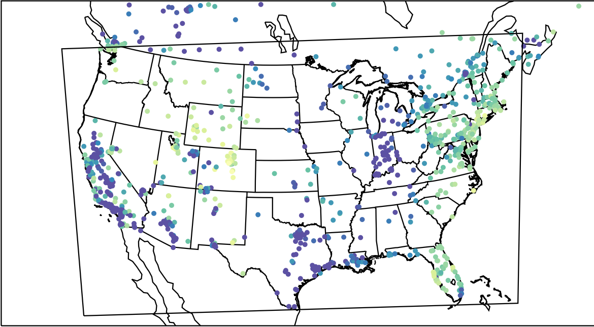
AirNOW (2024-01-10_04:00:00)
