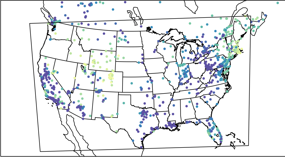
AirNOW (2024-01-10_11:00:00)
