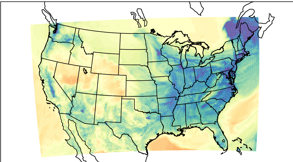
WRF (2024-01-11_04:00:00)
