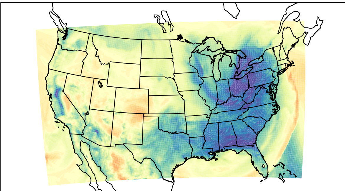
WRF (2024-01-10_10:00:00)
