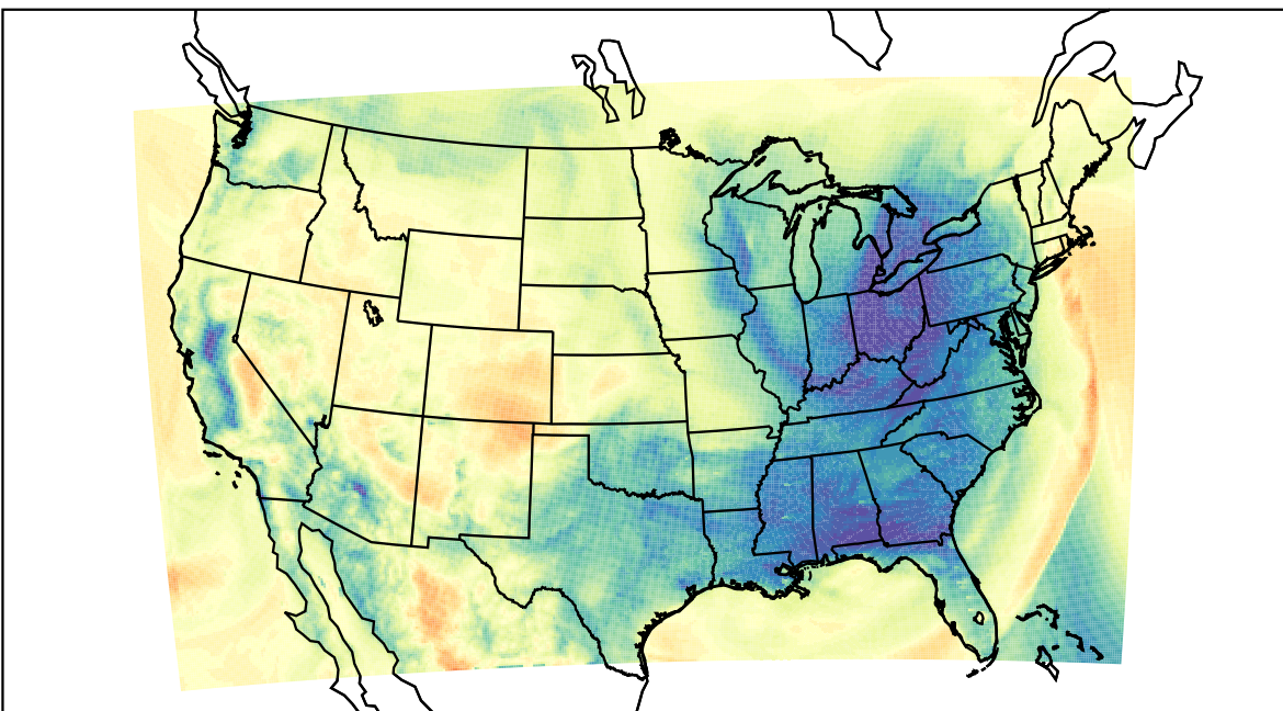
WRF (2024-01-10_09:00:00)
