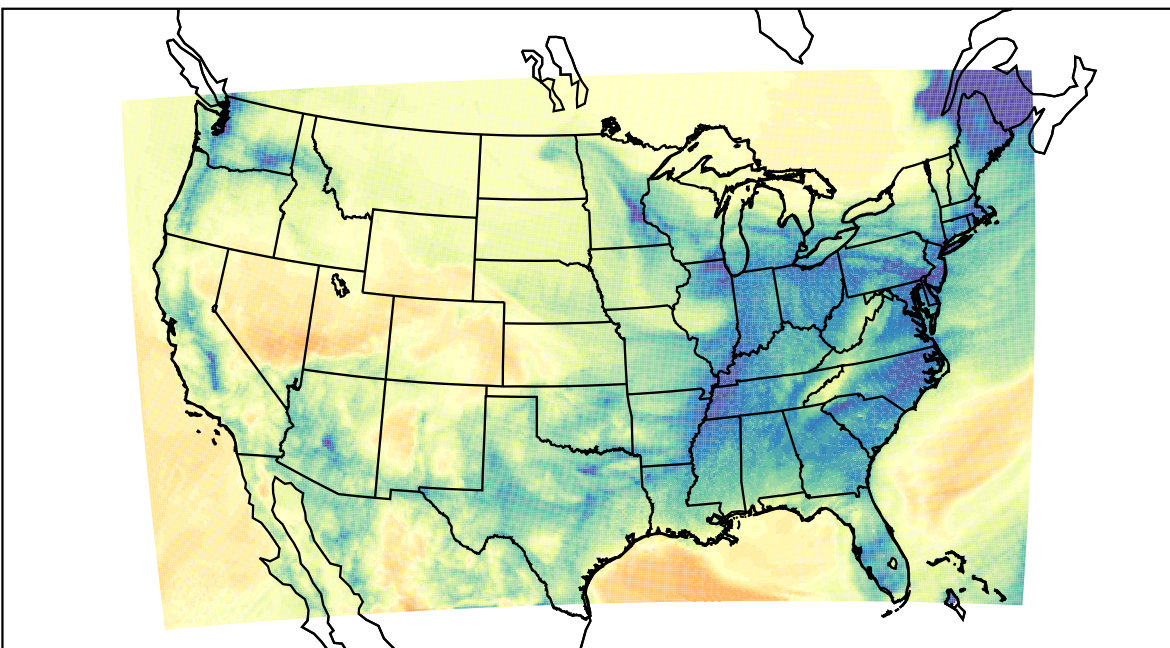
WRF (2024-01-11_08:00:00)
