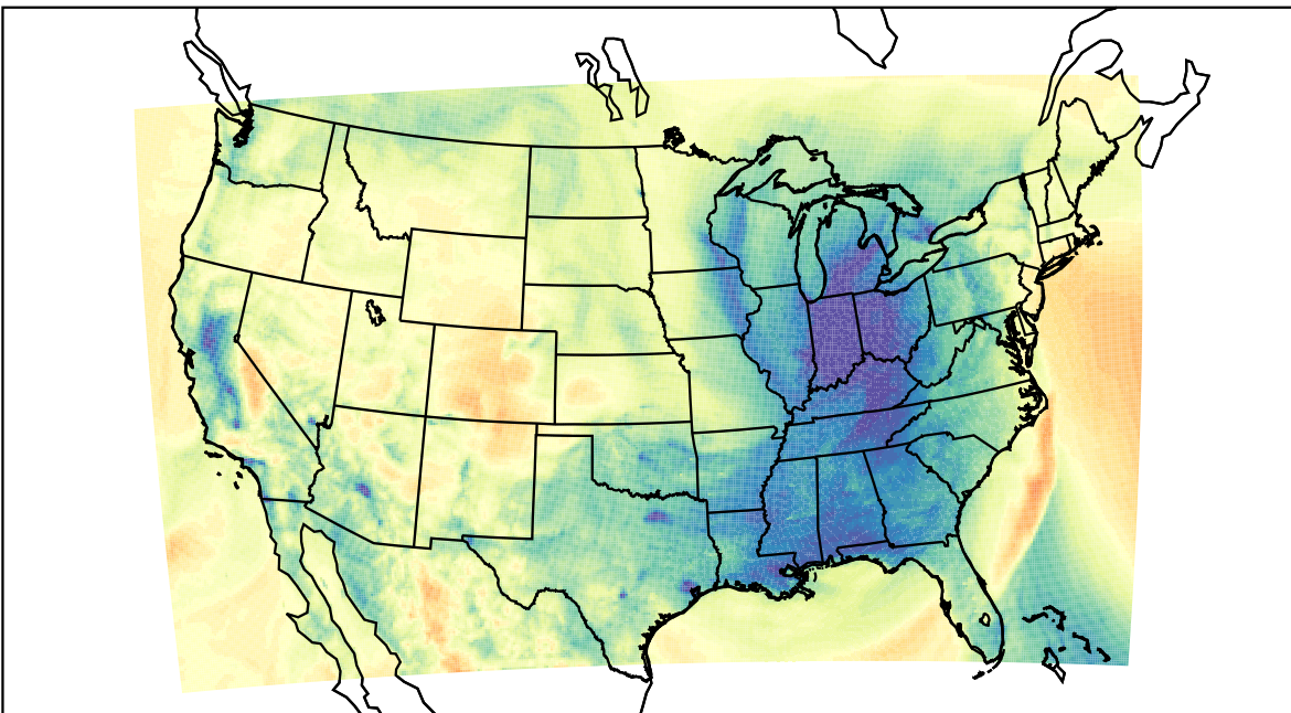
WRF (2024-01-10_05:00:00)
