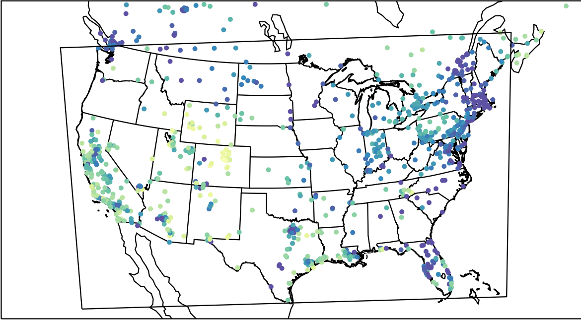
AirNOW (2024-01-11_00:00:00)
