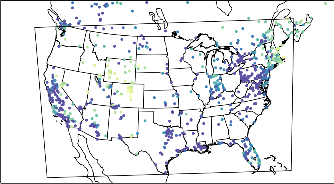
AirNOW (2024-01-10_13:00:00)
