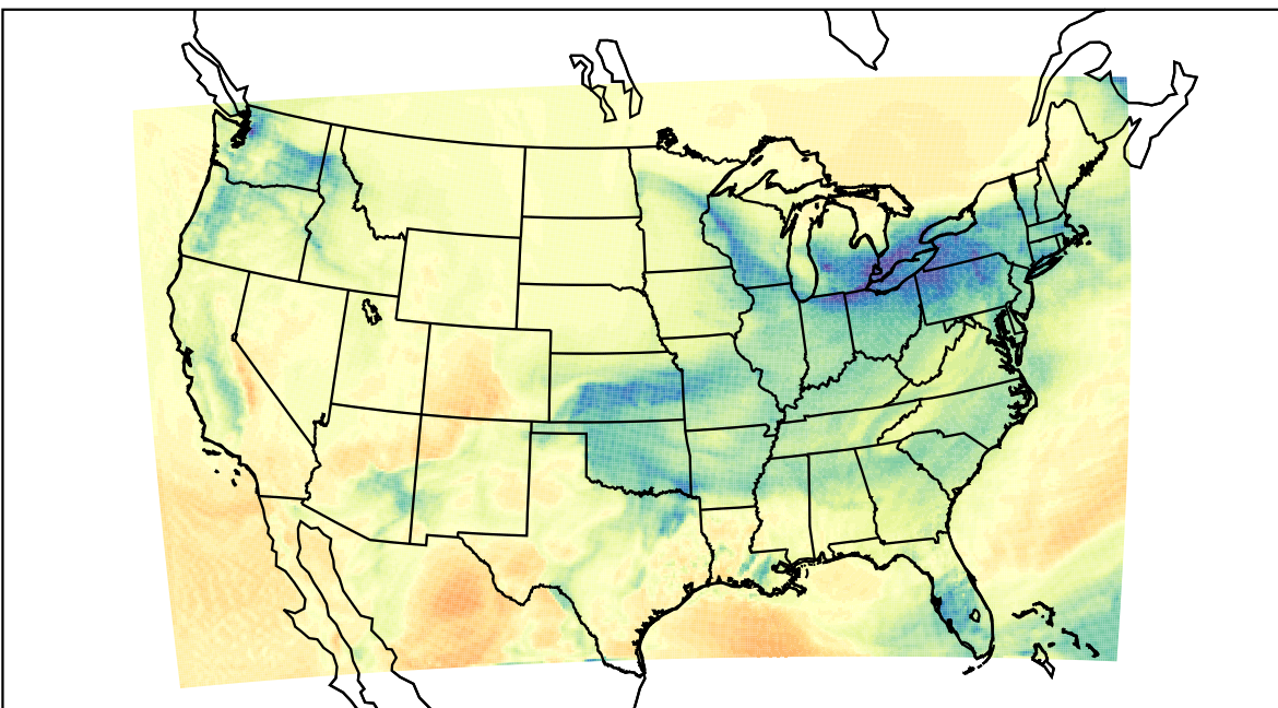
WRF (2024-01-11_19:00:00)
