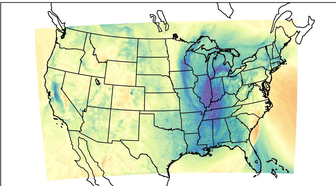
WRF (2024-01-10_00:00:00)
