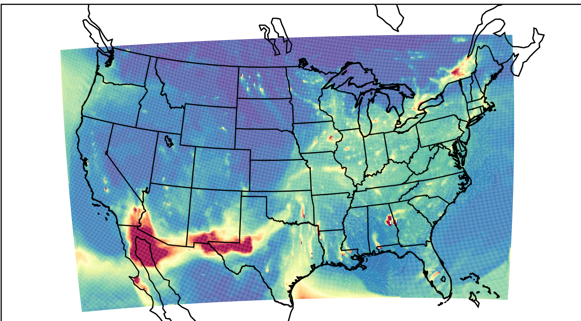
WRF 2024-01-12_01:00:00
