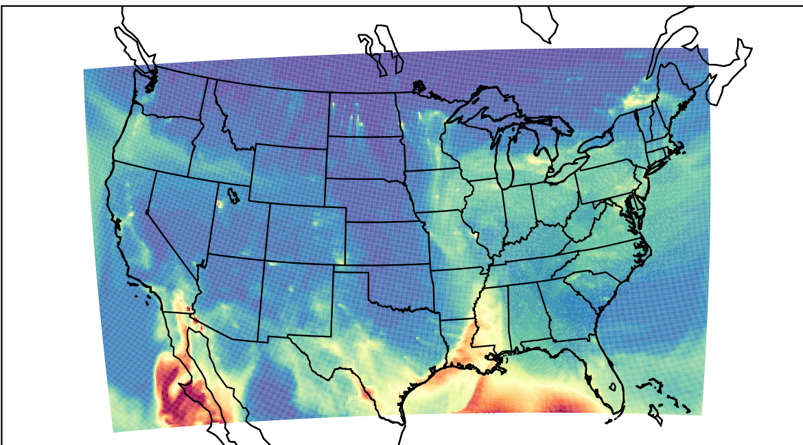
WRF 2024-01-12_15:00:00
