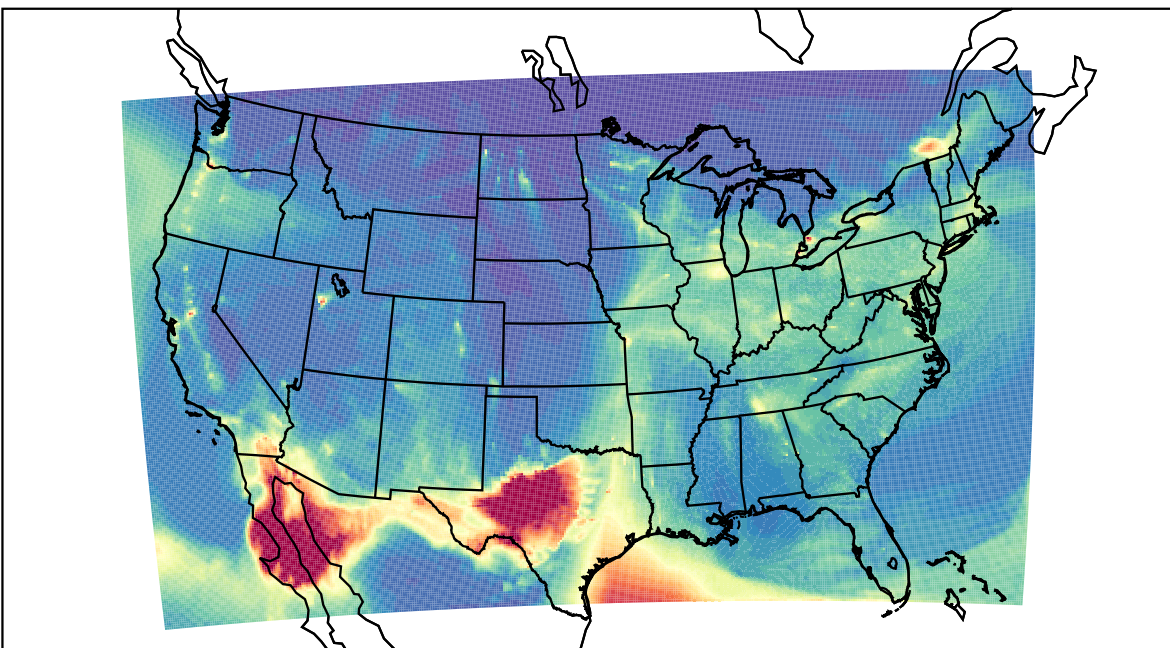
WRF 2024-01-12_07:00:00
