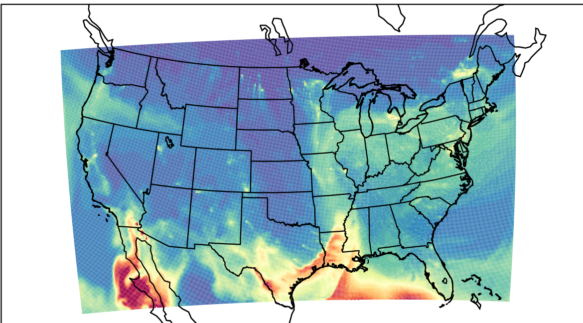
WRF 2024-01-12_14:00:00
