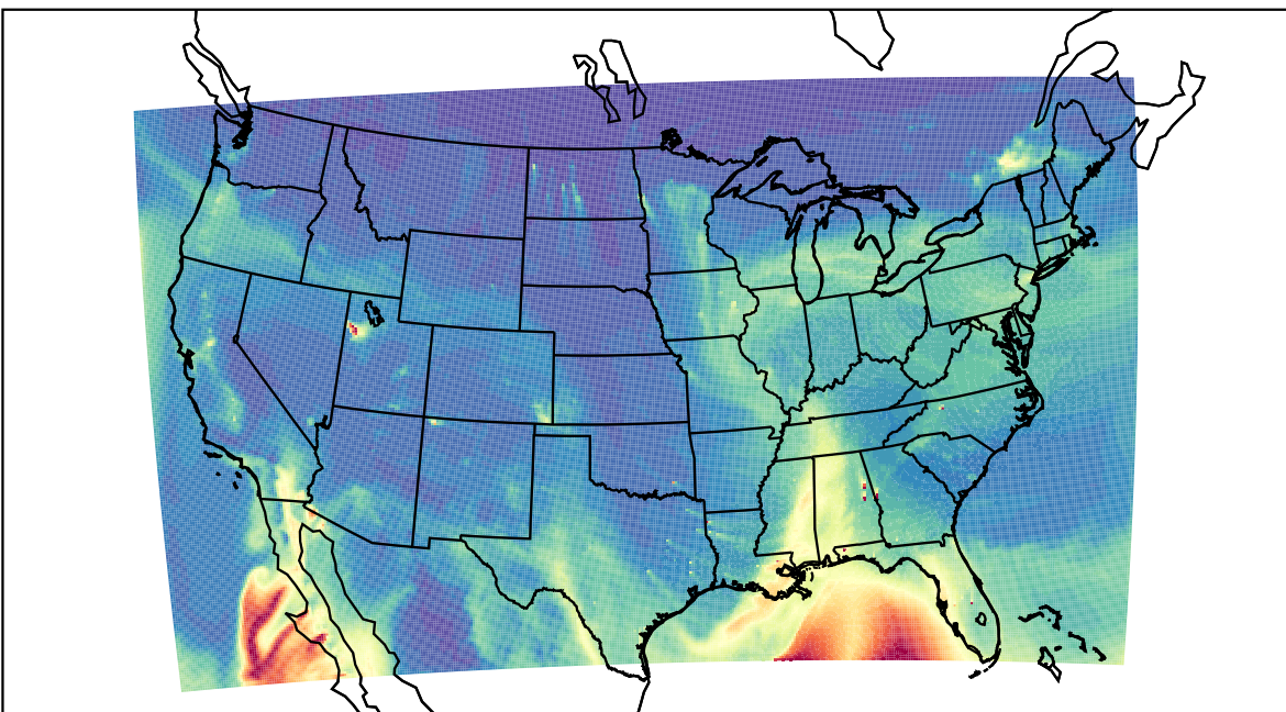
WRF 2024-01-12_18:00:00
