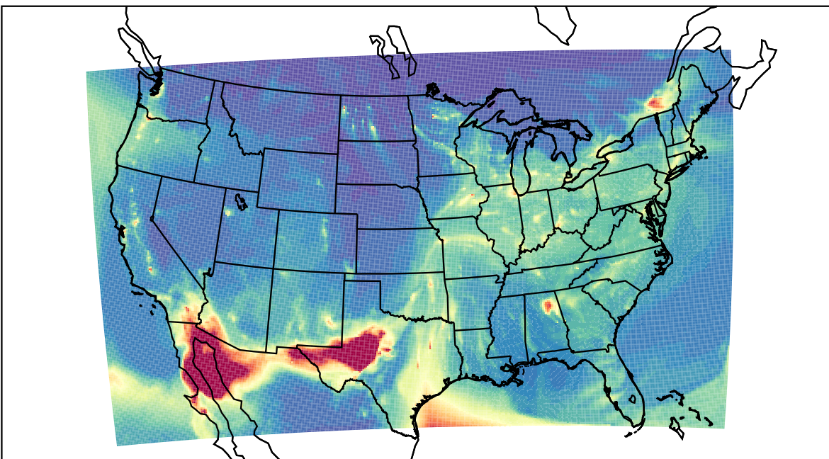
WRF 2024-01-12_04:00:00
