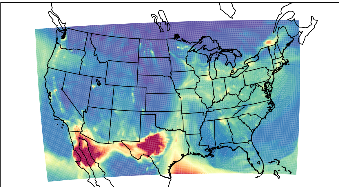
WRF 2024-01-12_06:00:00
