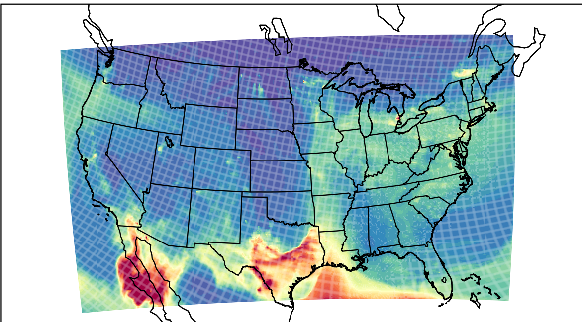
WRF 2024-01-12_11:00:00
