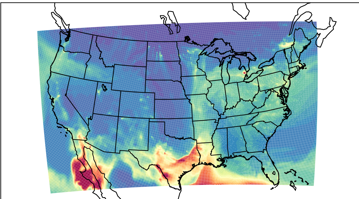
WRF 2024-01-12_12:00:00
