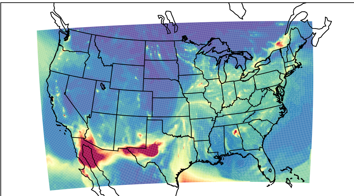
WRF 2024-01-12_03:00:00
