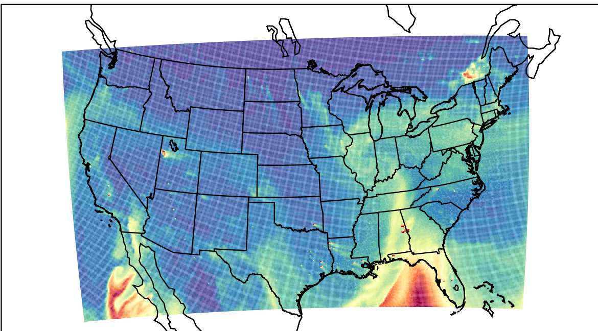
WRF 2024-01-12_21:00:00
