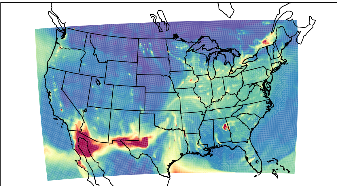
WRF 2024-01-12_02:00:00
