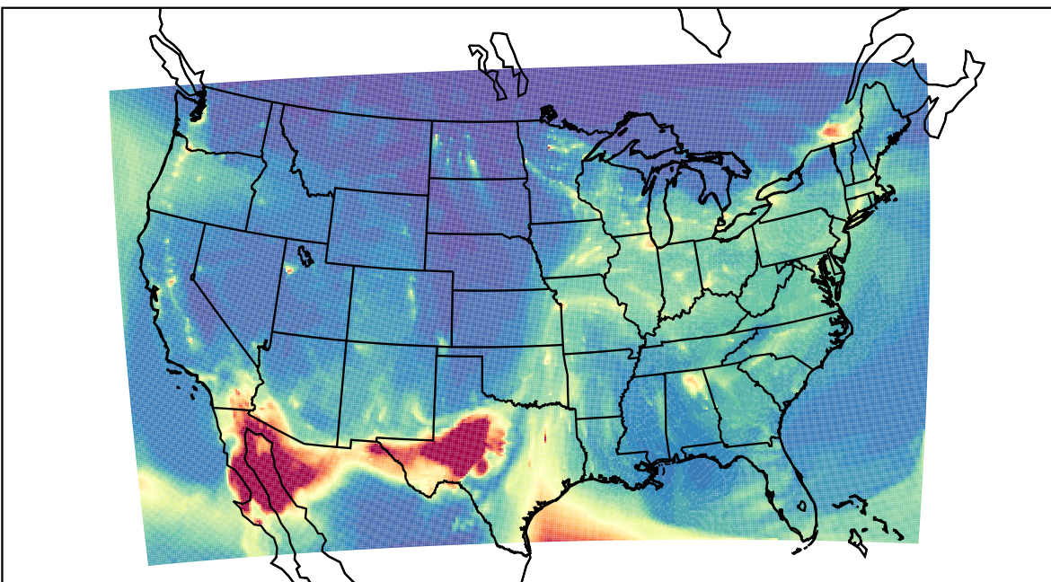
WRF 2024-01-12_05:00:00
