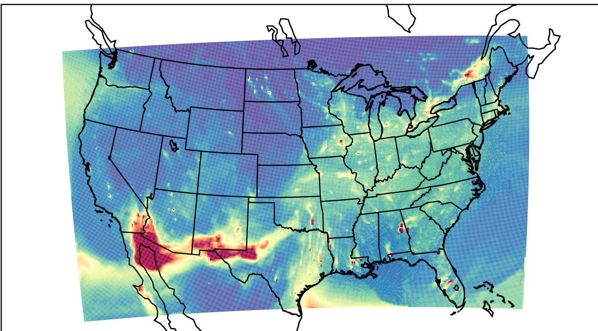
WRF 2024-01-12_00:00:00
