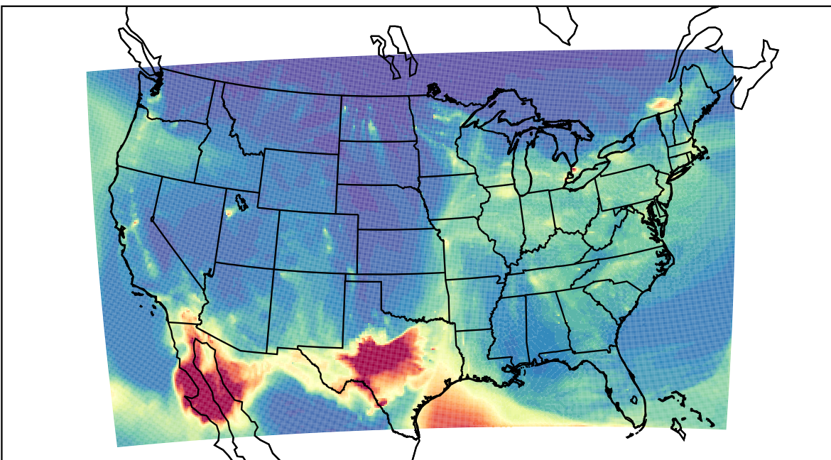
WRF 2024-01-12_08:00:00
