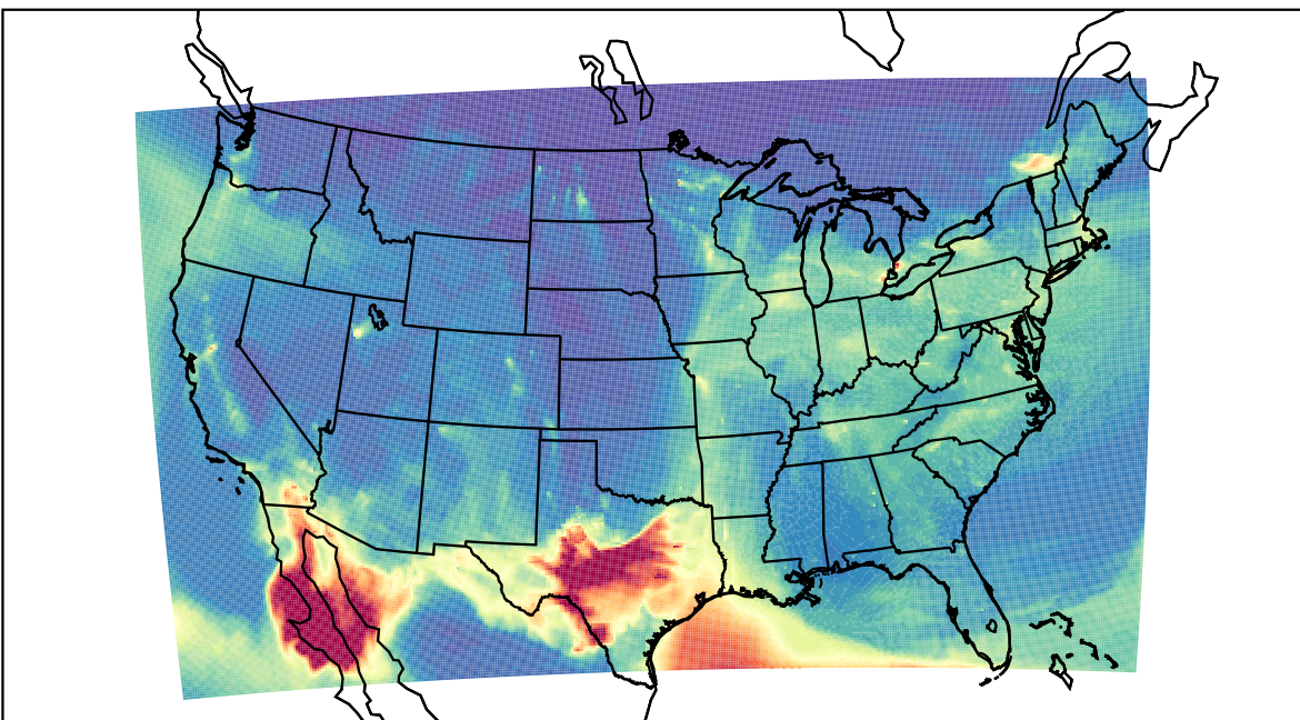
WRF 2024-01-12_09:00:00
