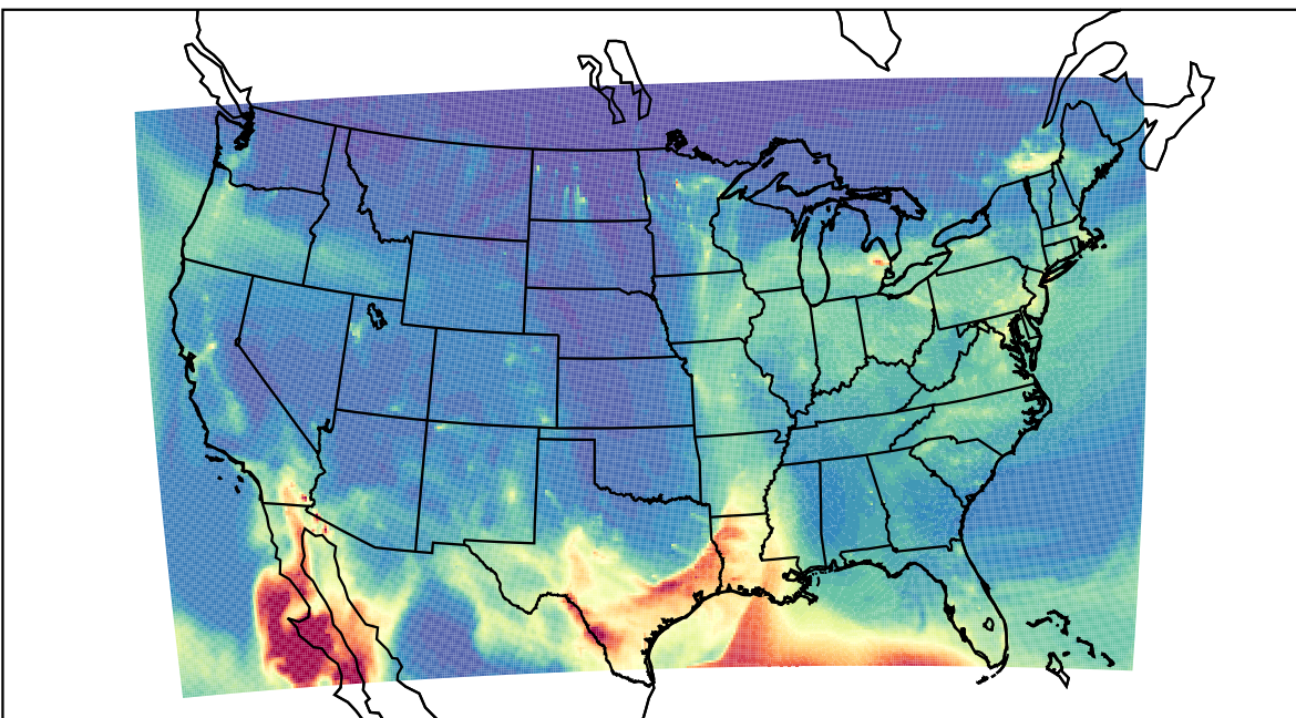
WRF 2024-01-12_13:00:00
