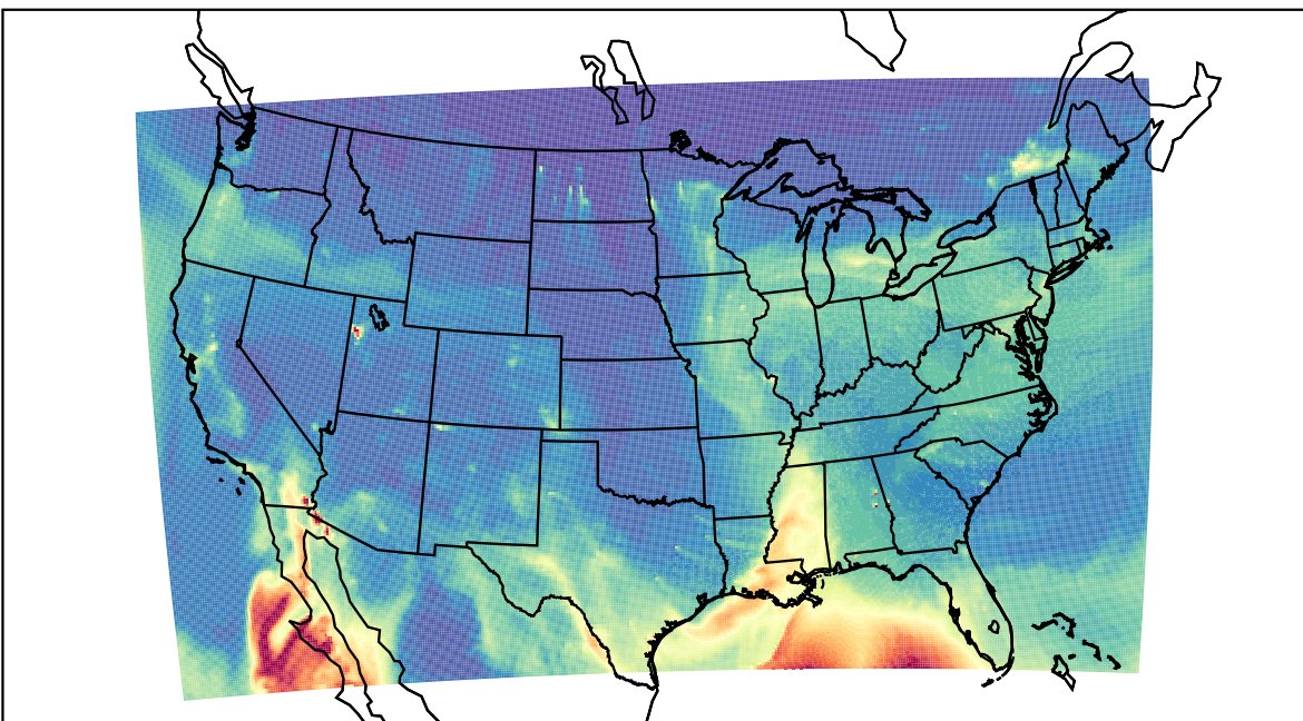
WRF 2024-01-12_16:00:00
