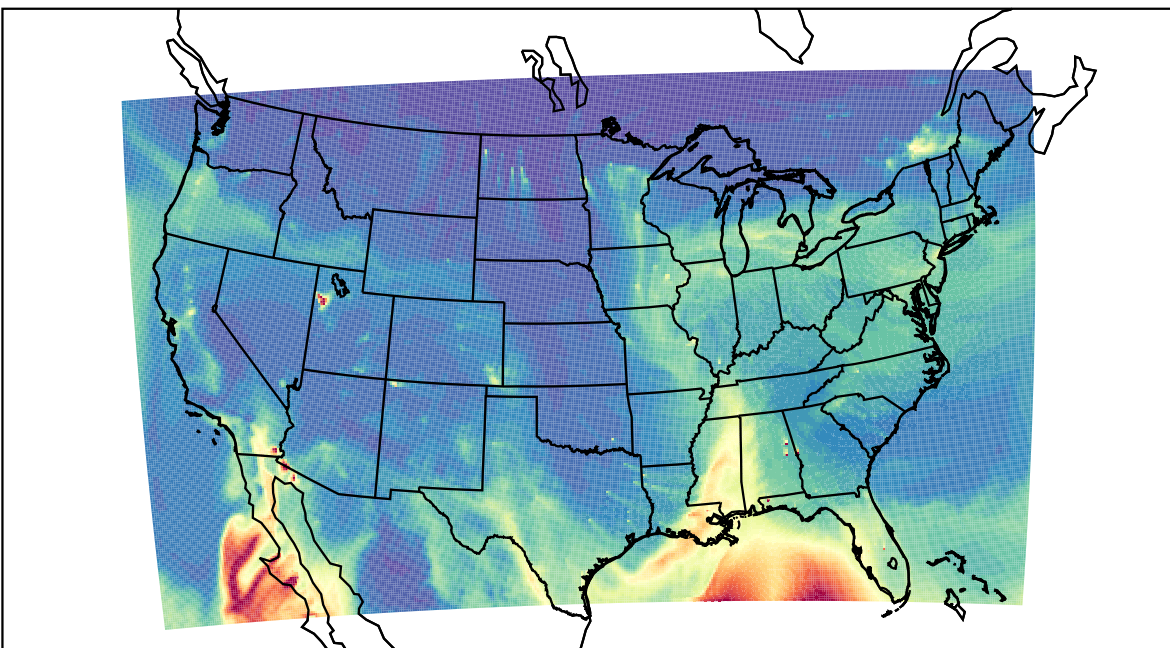
WRF 2024-01-12_17:00:00
