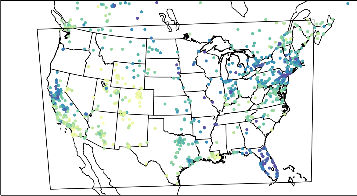
AirNOW (2024-01-12_21:00:00)
