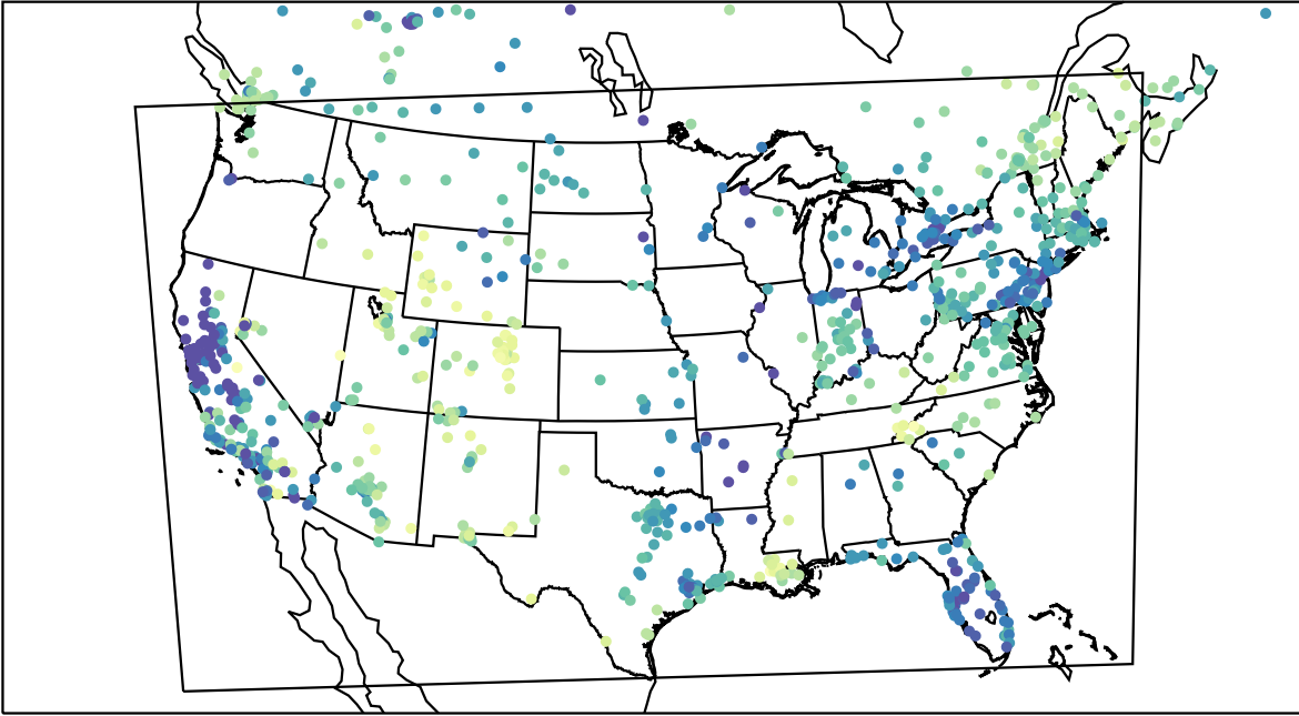
AirNOW (2024-01-12_18:00:00)
