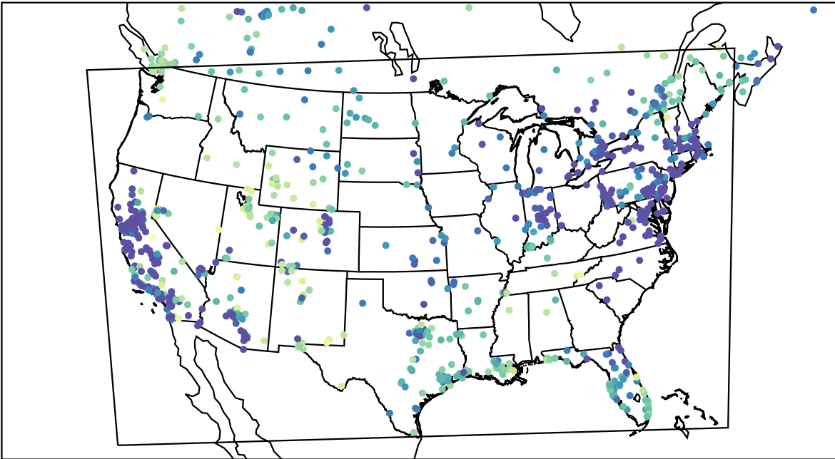
AirNOW (2024-01-12_07:00:00)
