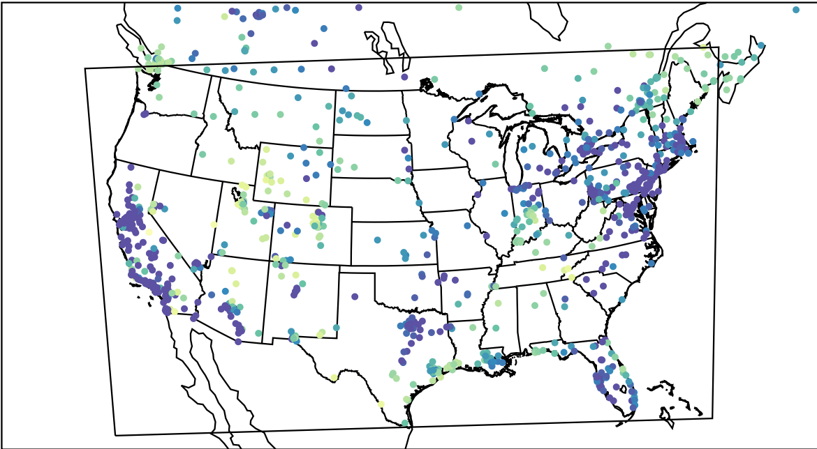
AirNOW (2024-01-12_14:00:00)
