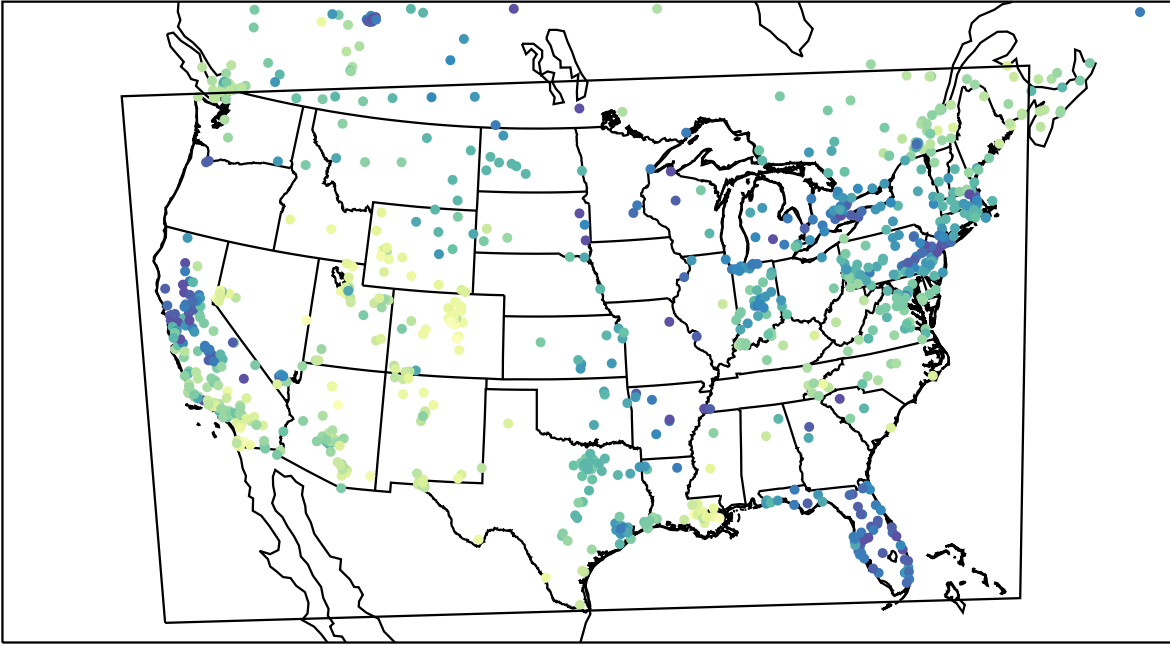
AirNOW (2024-01-12_20:00:00)
