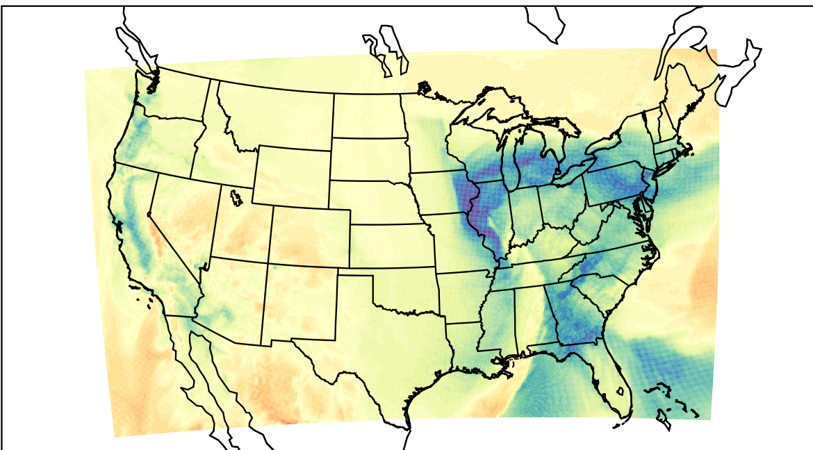
WRF (2024-01-12_19:00:00)
