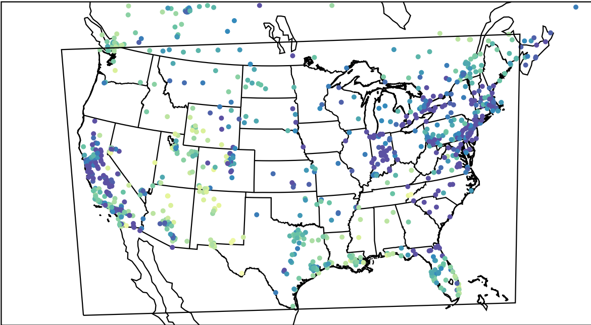
AirNOW (2024-01-12_02:00:00)
