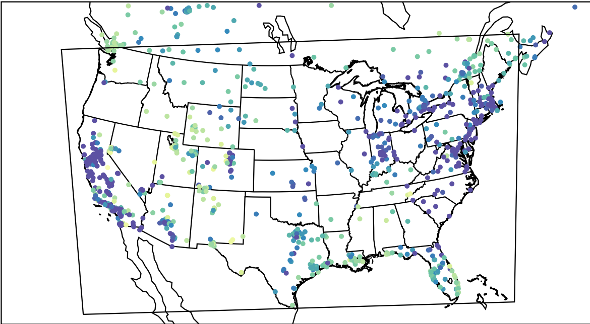
AirNOW (2024-01-12_06:00:00)
