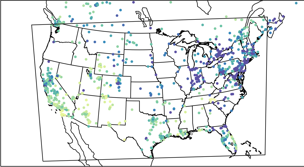
AirNOW (2024-01-12_00:00:00)
