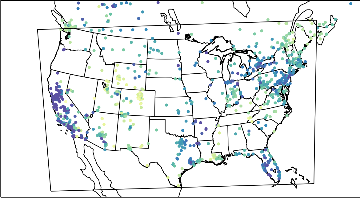
AirNOW (2024-01-12_17:00:00)
