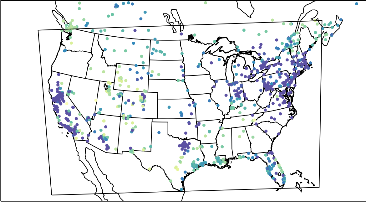
AirNOW (2024-01-12_10:00:00)
