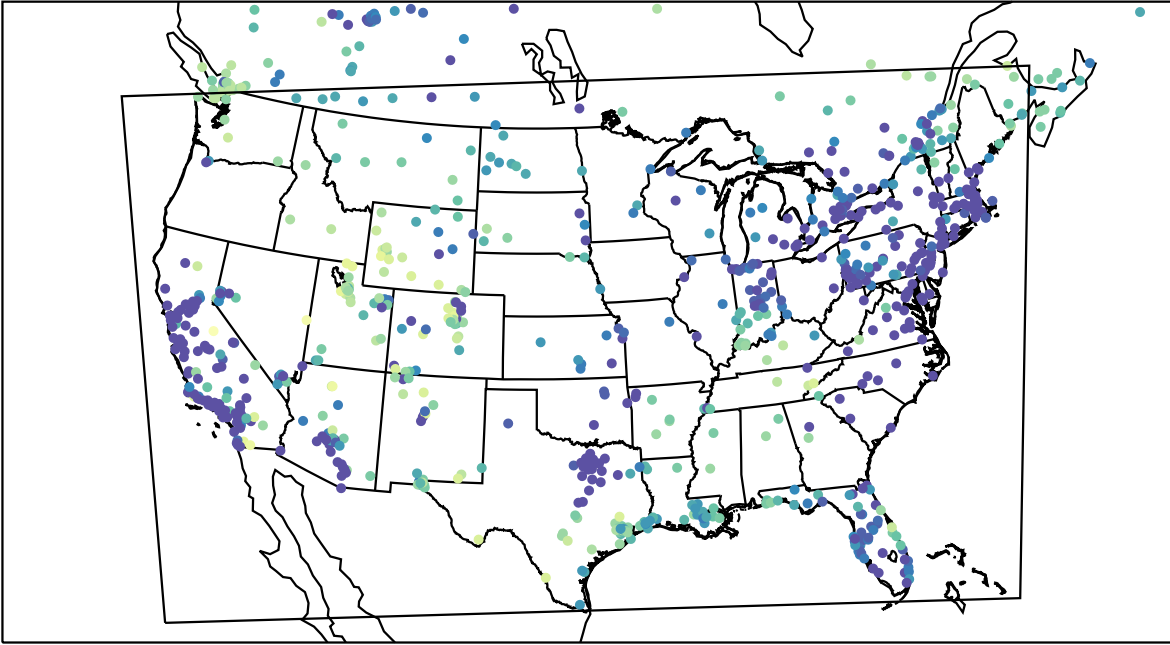
AirNOW (2024-01-12_12:00:00)
