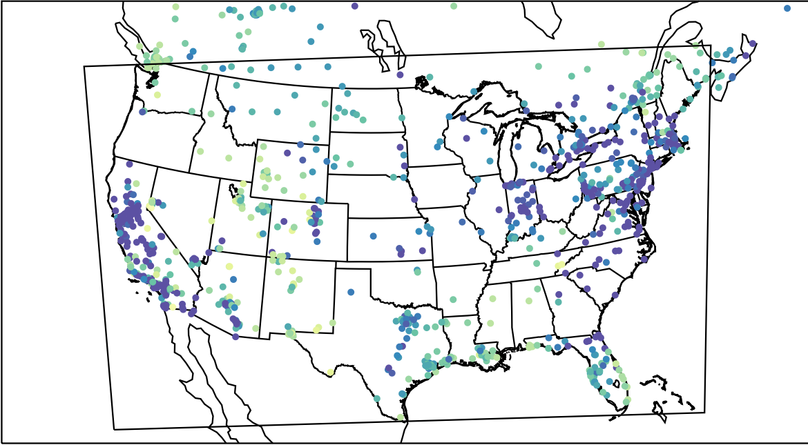
AirNOW (2024-01-12_05:00:00)
