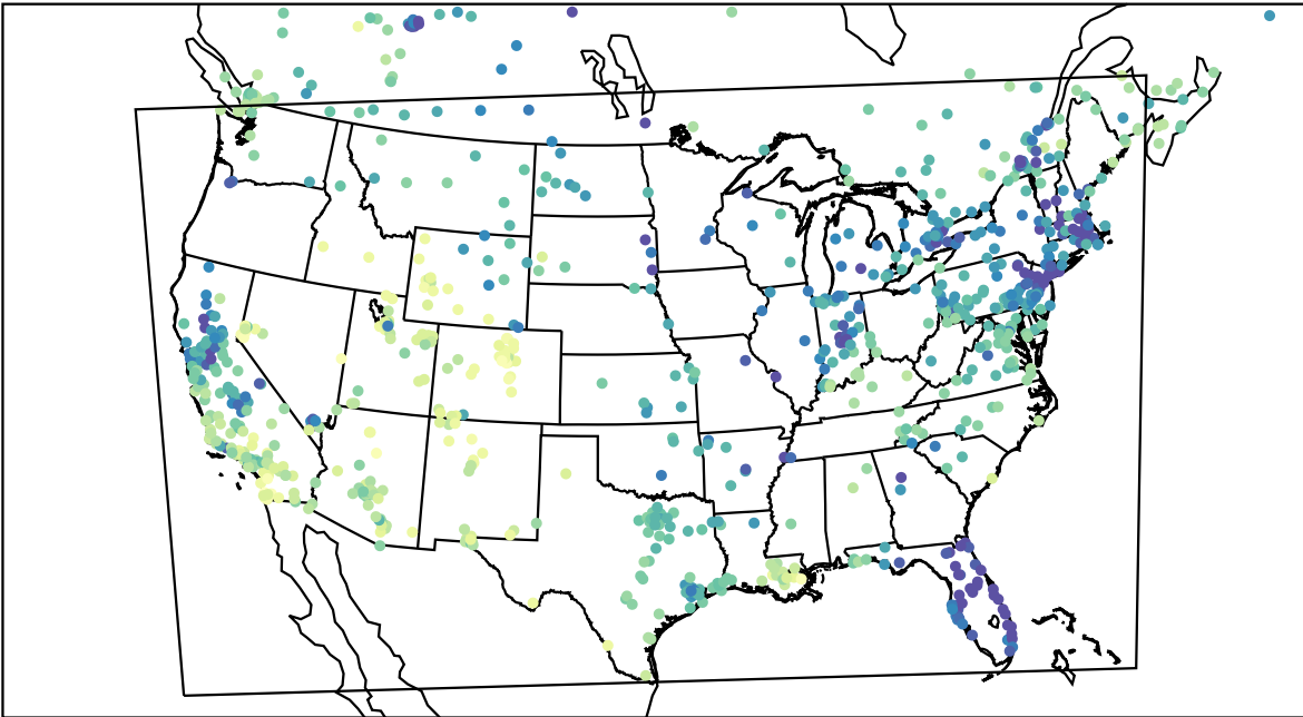
AirNOW (2024-01-12_22:00:00)
