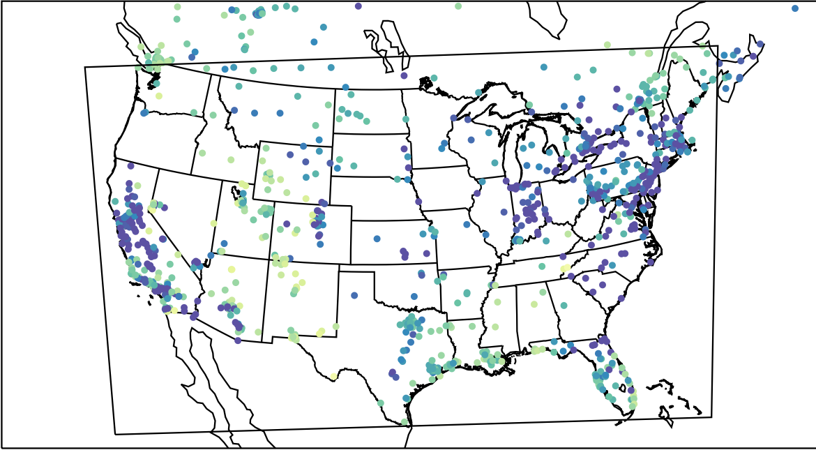
AirNOW (2024-01-12_03:00:00)
