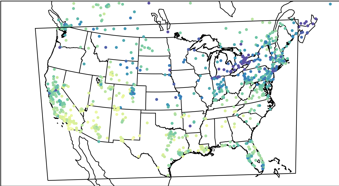
AirNOW (2024-01-11_21:00:00)
