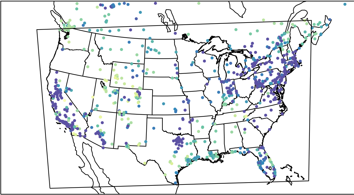
AirNOW (2024-01-12_11:00:00)
