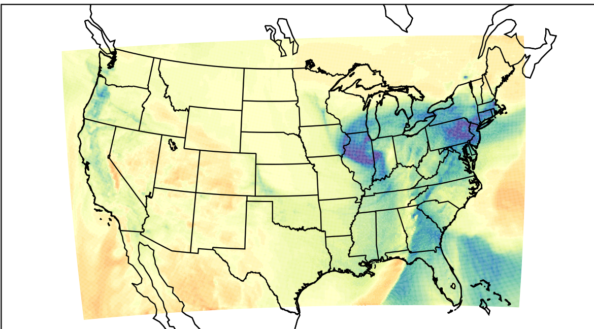
WRF (2024-01-12_22:00:00)
