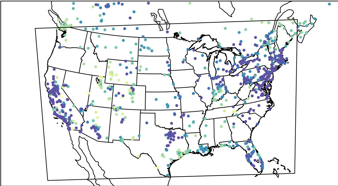
AirNOW (2024-01-12_13:00:00)
