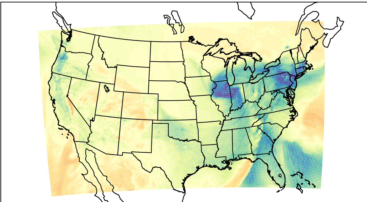
WRF (2024-01-12_23:00:00)
