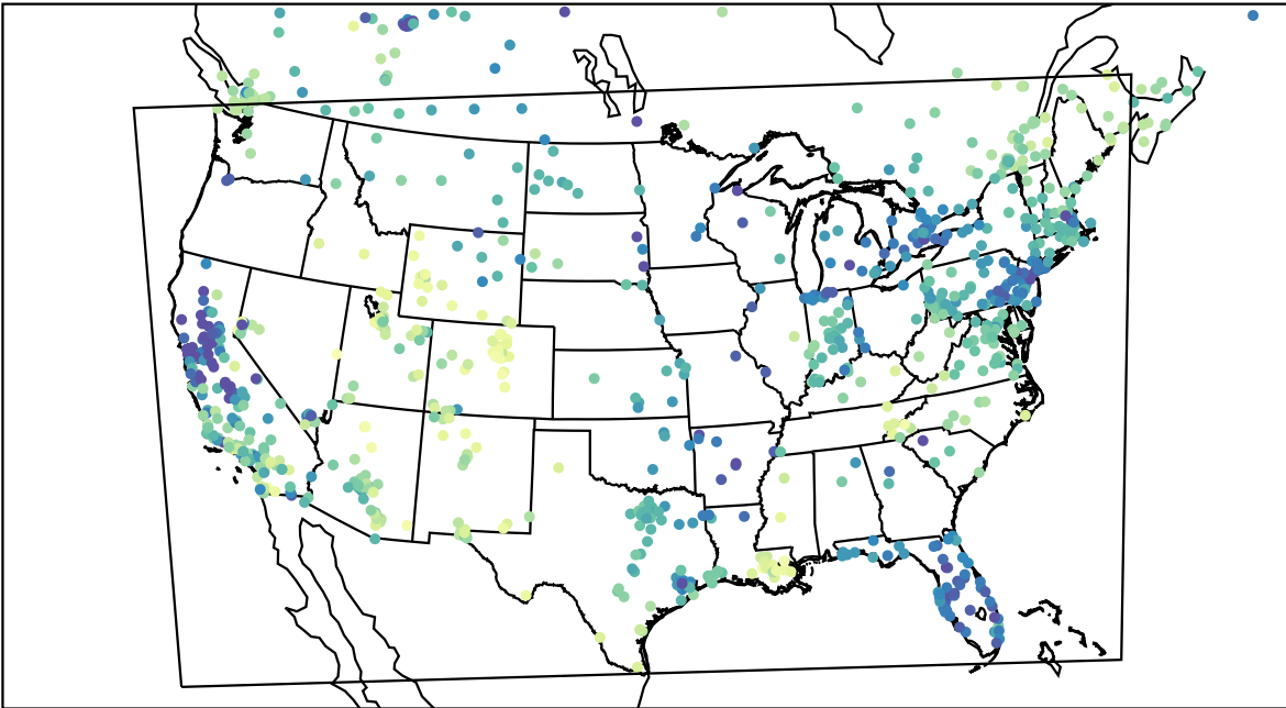
AirNOW (2024-01-12_19:00:00)
