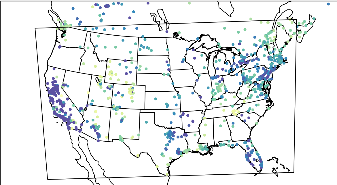
AirNOW (2024-01-12_16:00:00)
