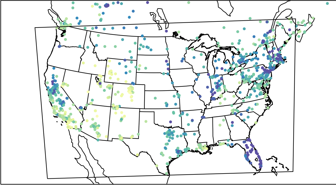
AirNOW (2024-01-12_23:00:00)
