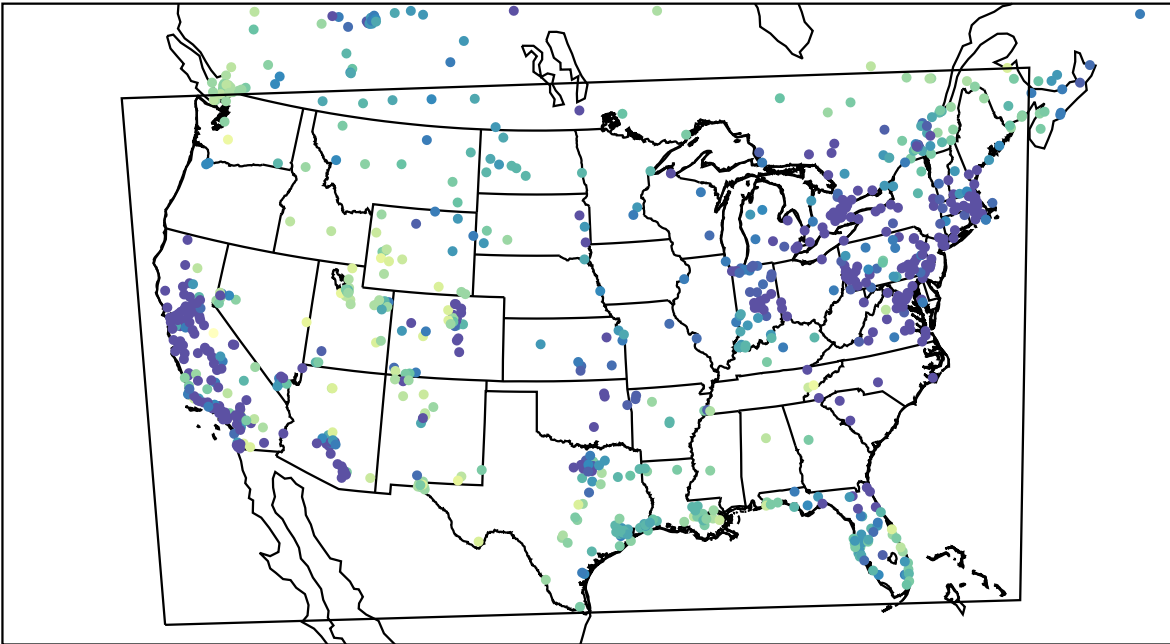
AirNOW (2024-01-12_08:00:00)
