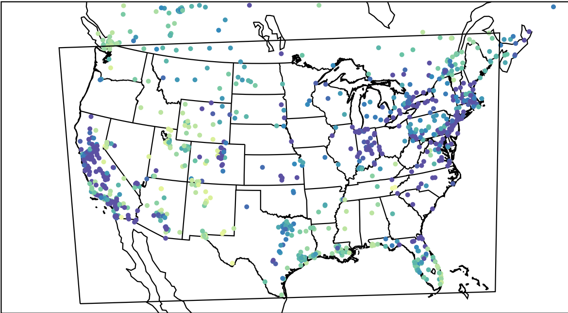
AirNOW (2024-01-12_04:00:00)
