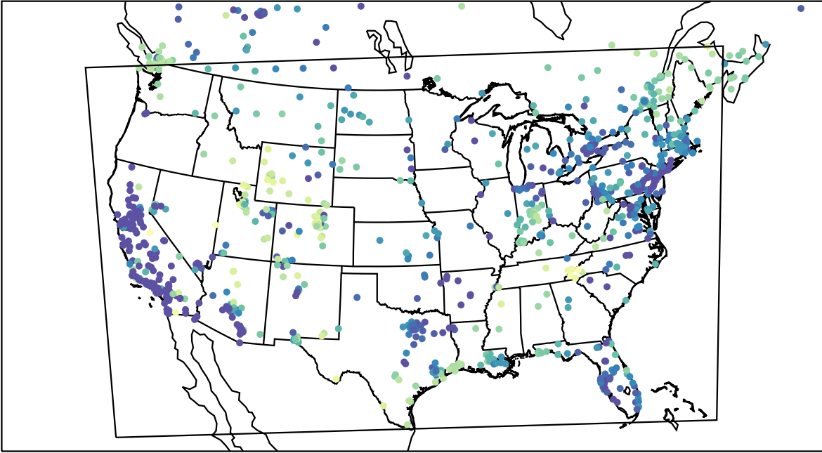
AirNOW (2024-01-12_15:00:00)
