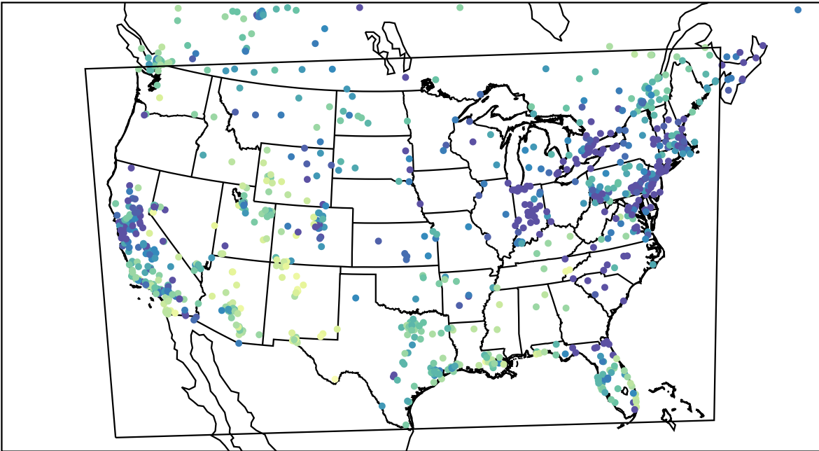
AirNOW (2024-01-12_01:00:00)
