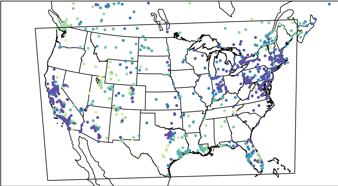
AirNOW (2024-01-12_09:00:00)
