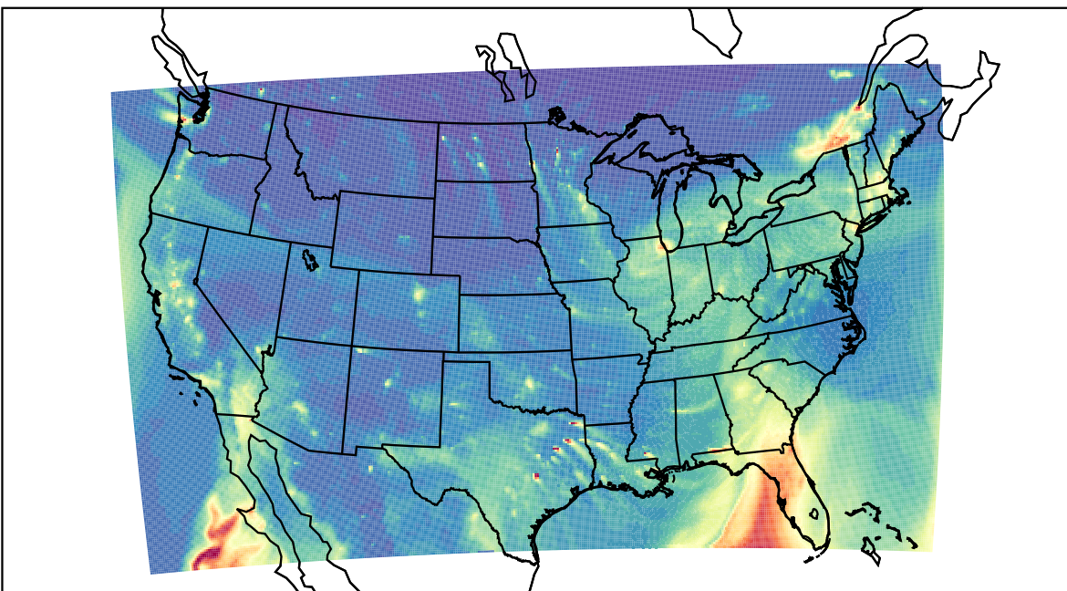
WRF 2024-01-13_02:00:00
