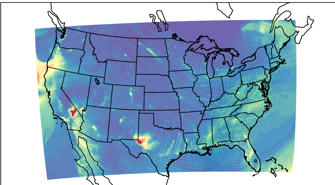
WRF 2024-01-14_06:00:00
