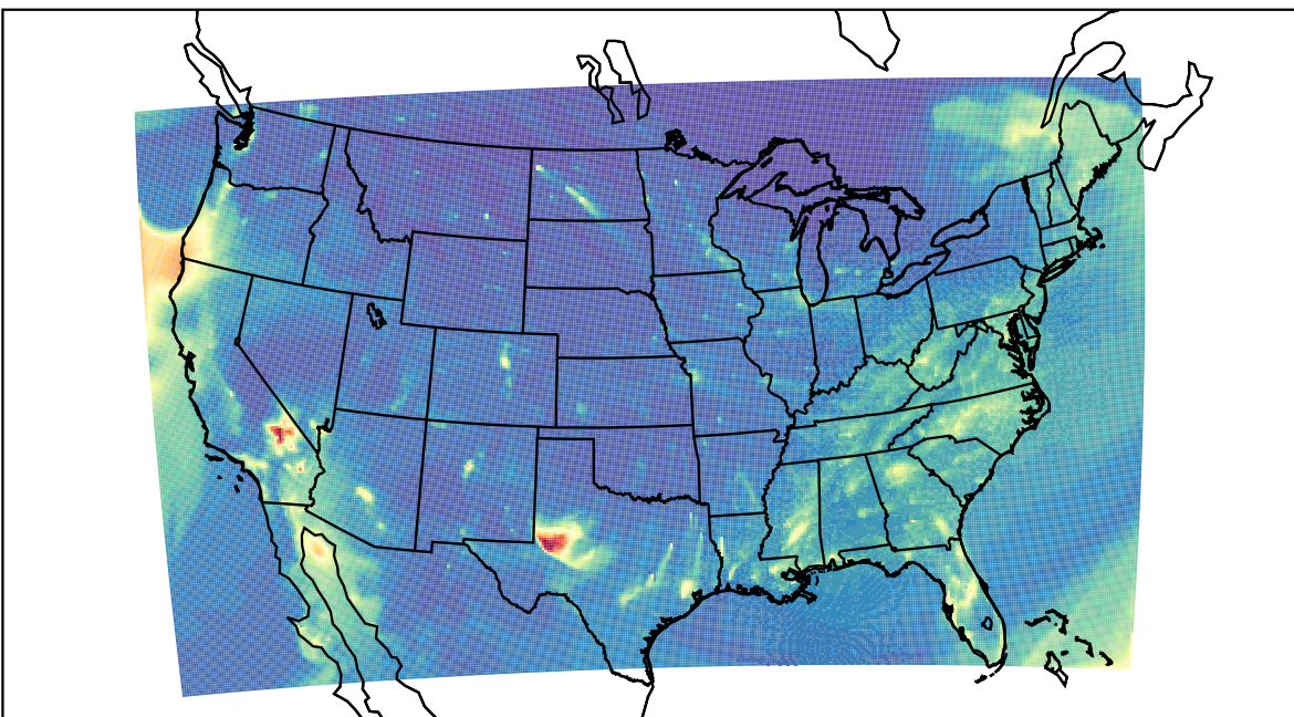
WRF 2024-01-14_04:00:00
