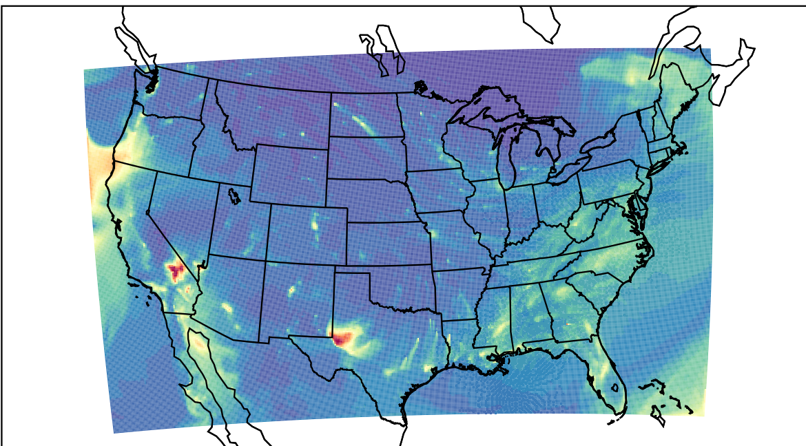
WRF 2024-01-14_05:00:00
