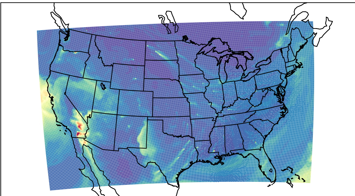
WRF 2024-01-14_20:00:00
