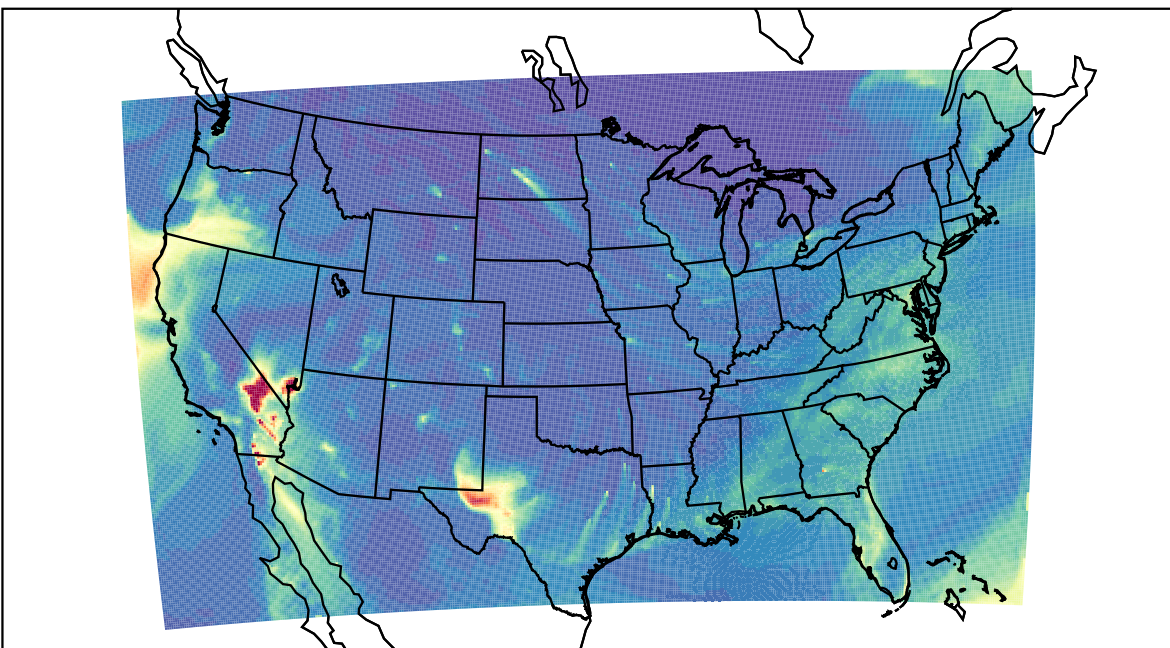
WRF 2024-01-14_09:00:00
