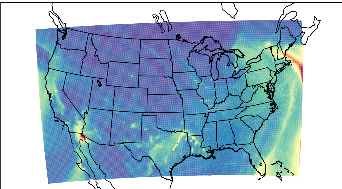
WRF 2024-01-13_16:00:00
