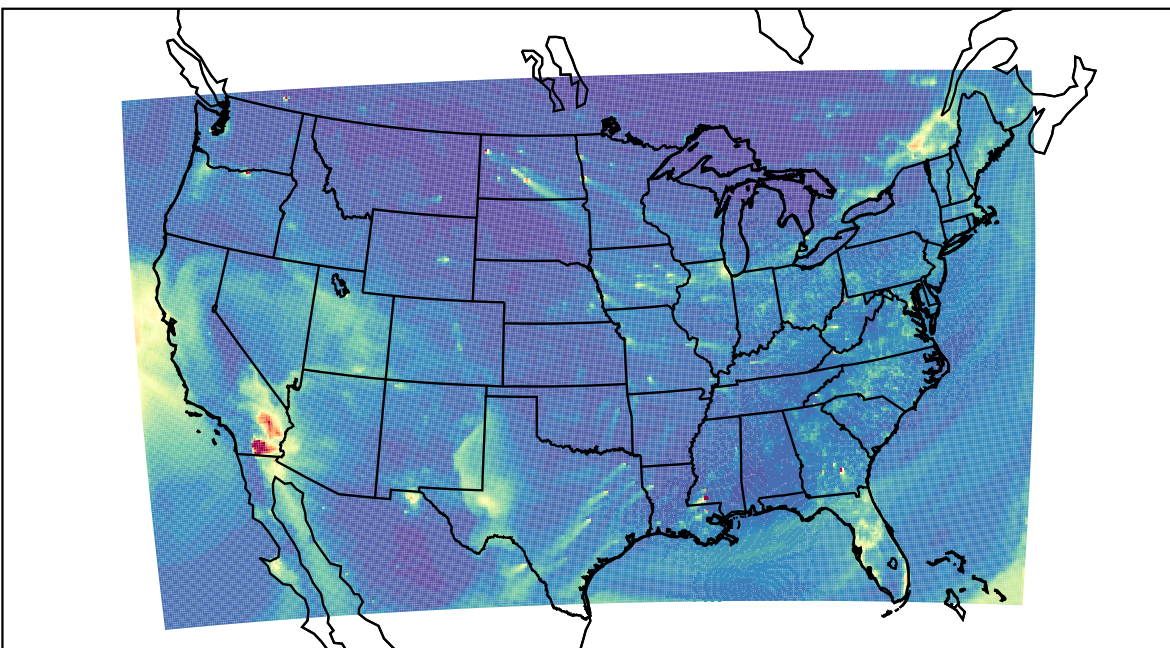
WRF 2024-01-14_23:00:00
