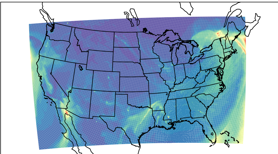
WRF 2024-01-13_20:00:00
