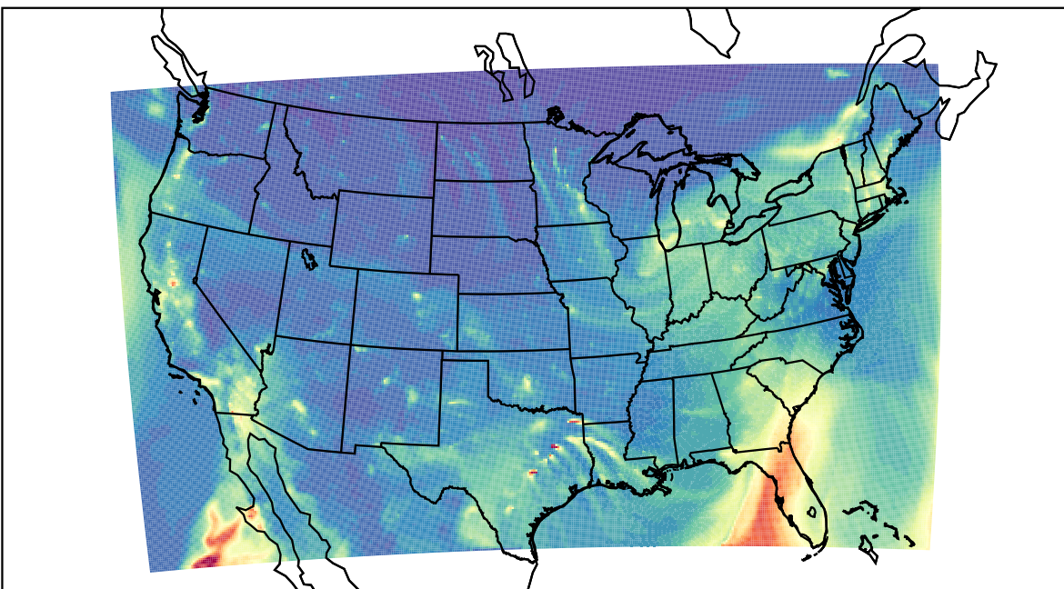
WRF 2024-01-13_04:00:00
