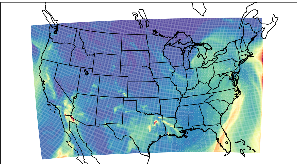
WRF 2024-01-13_10:00:00
