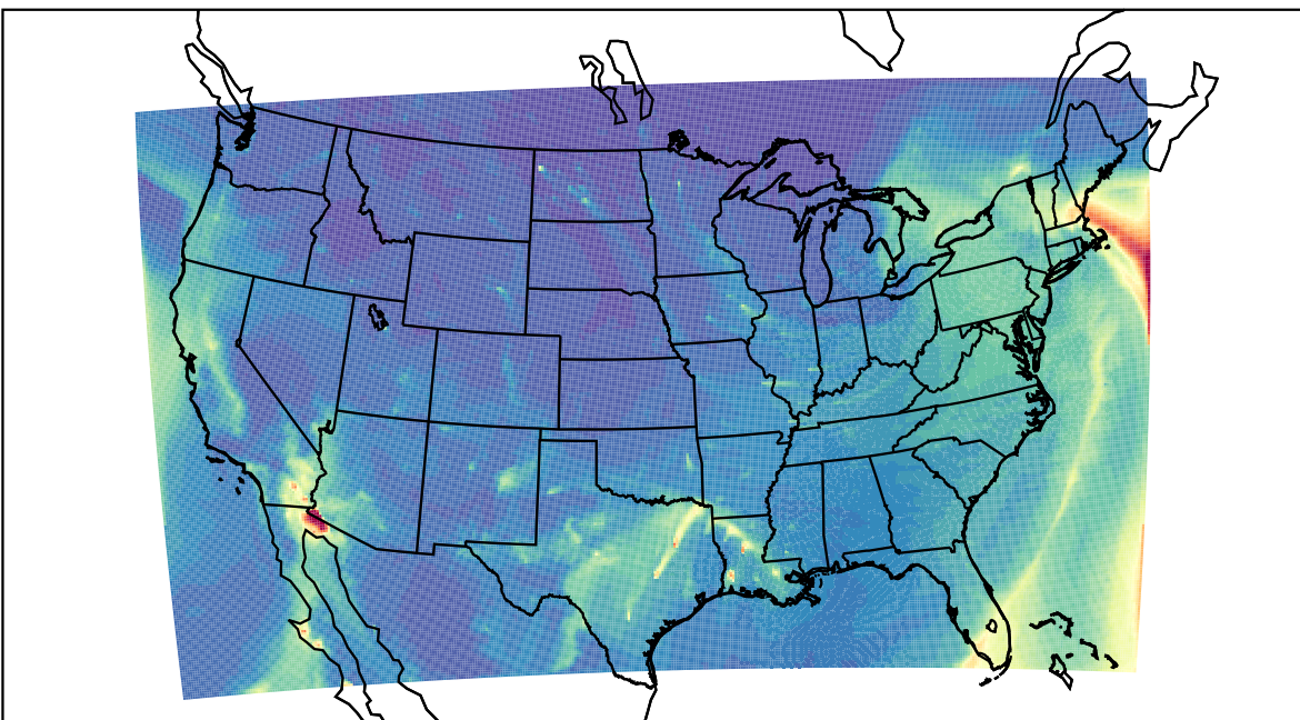
WRF 2024-01-13_15:00:00
