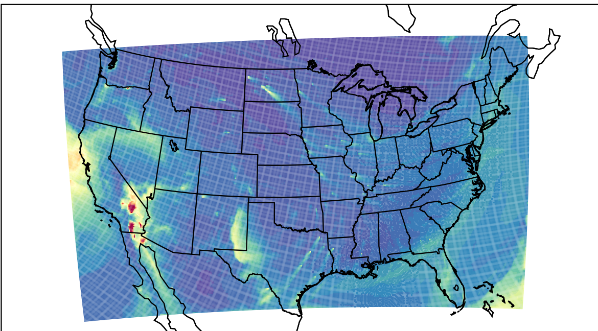
WRF 2024-01-14_17:00:00
