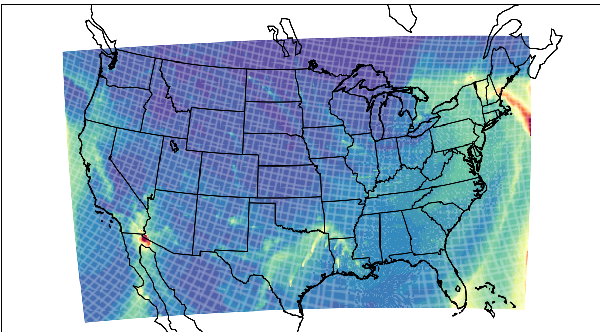
WRF 2024-01-13_17:00:00
