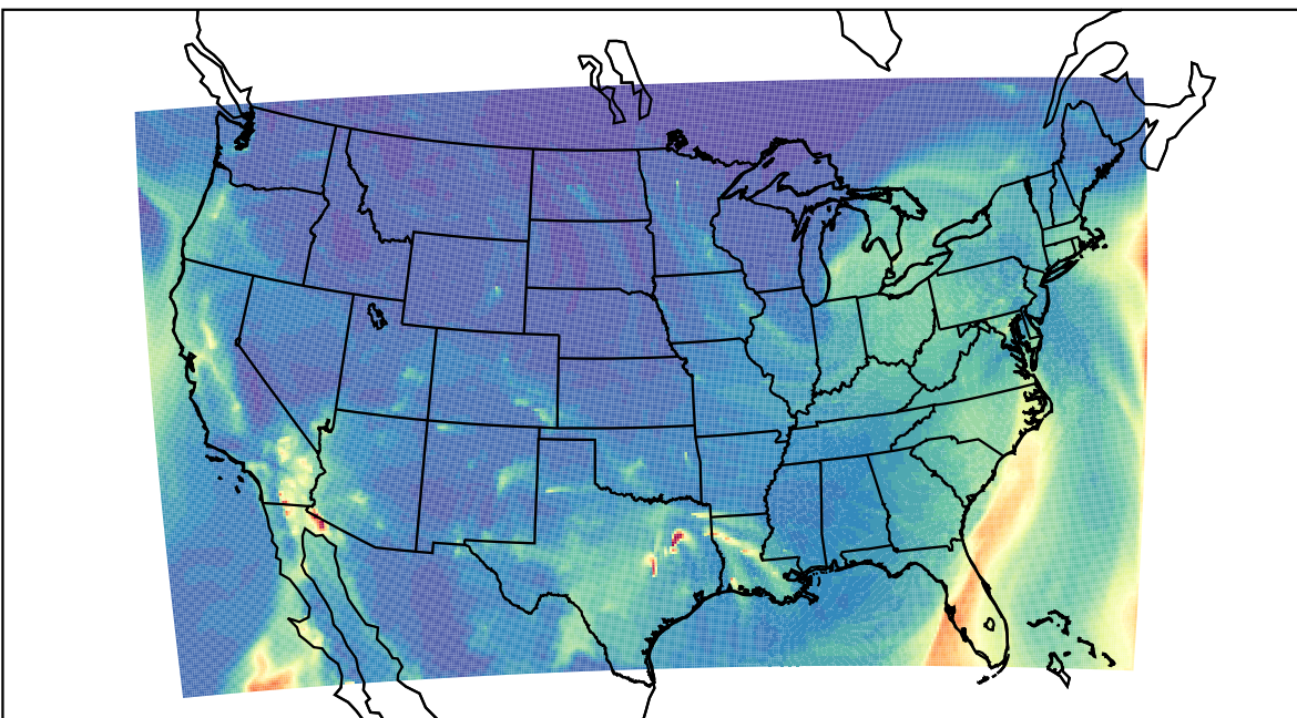
WRF 2024-01-13_09:00:00
