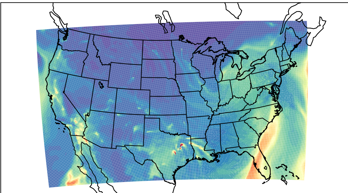
WRF 2024-01-13_08:00:00
