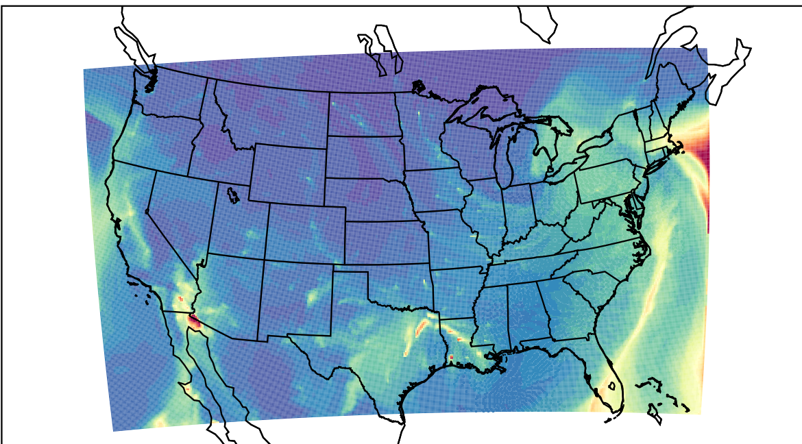
WRF 2024-01-13_13:00:00
