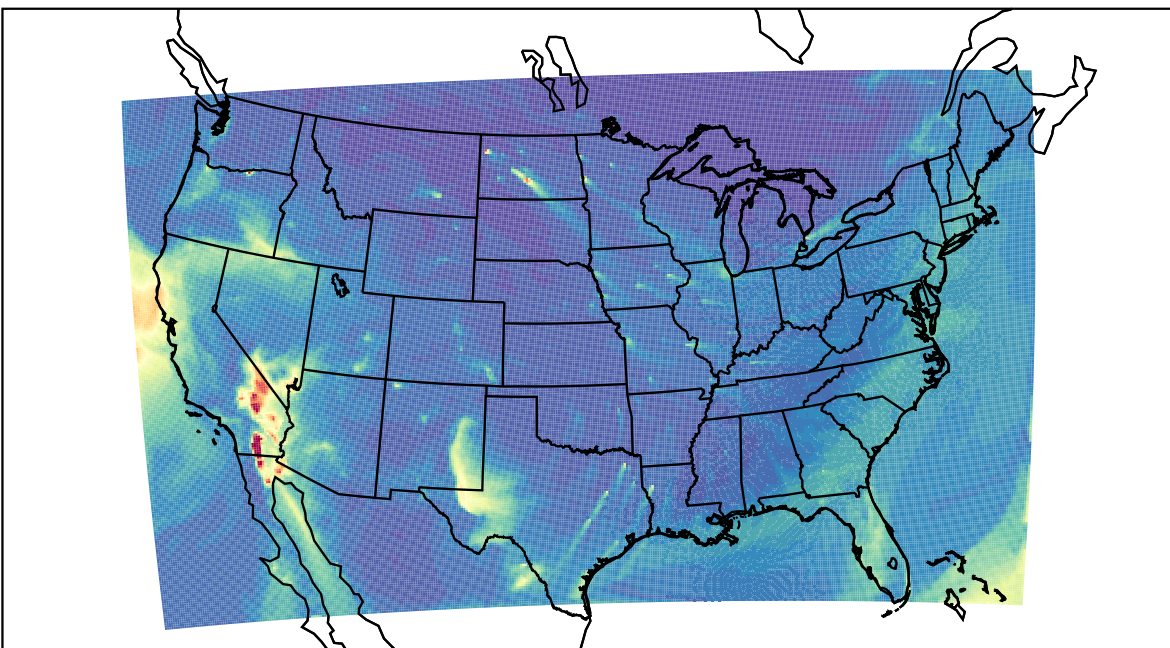
WRF 2024-01-14_15:00:00
