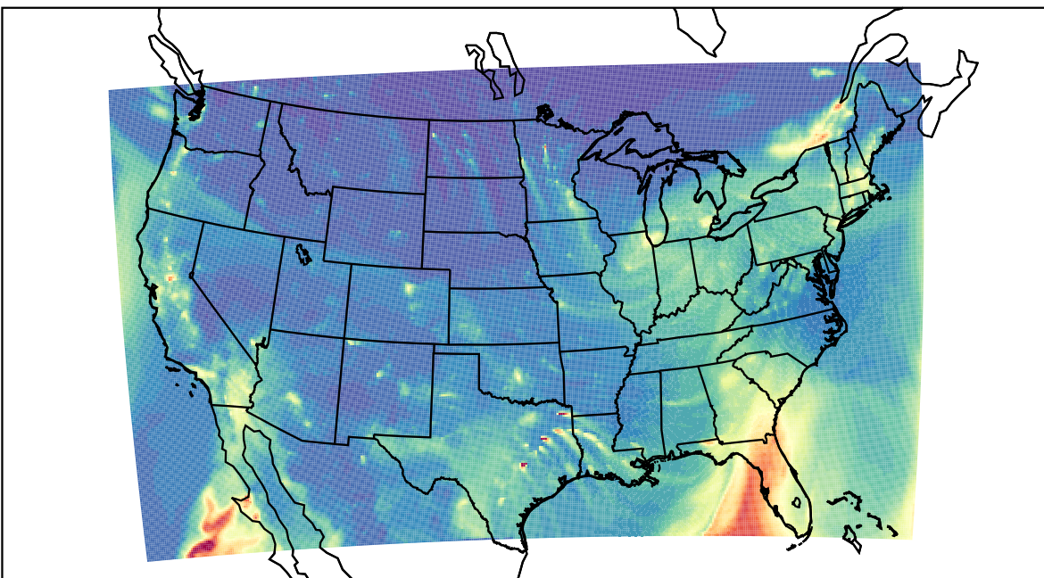
WRF 2024-01-13_03:00:00
