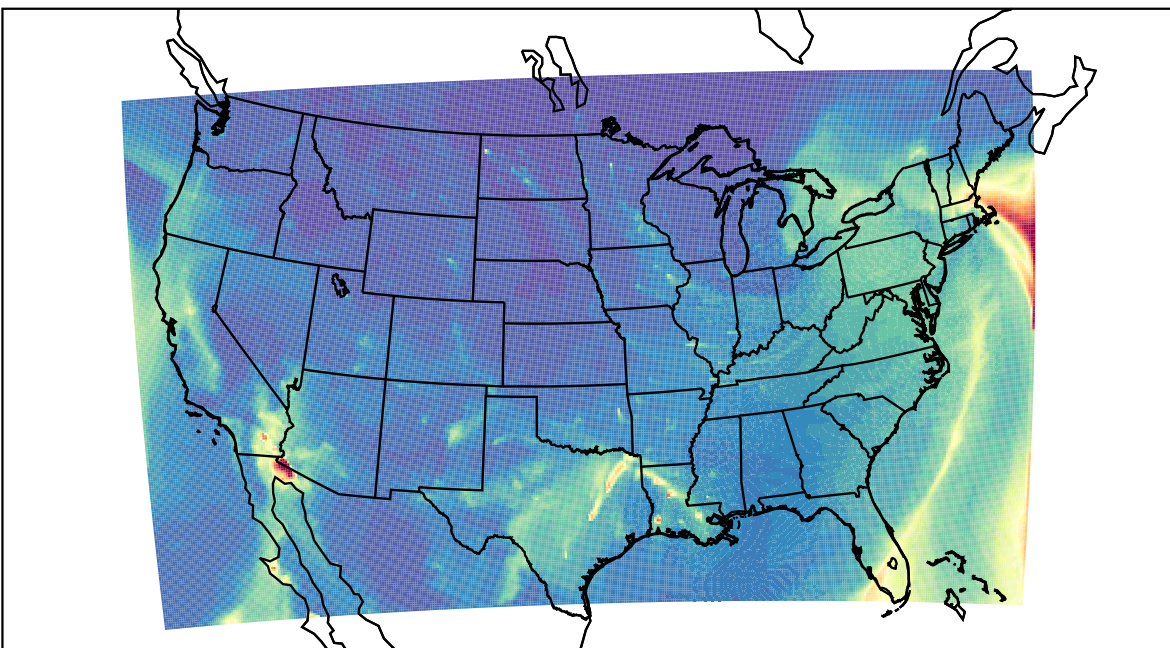
WRF 2024-01-13_14:00:00
