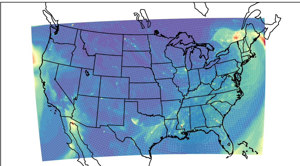
WRF 2024-01-13_23:00:00
