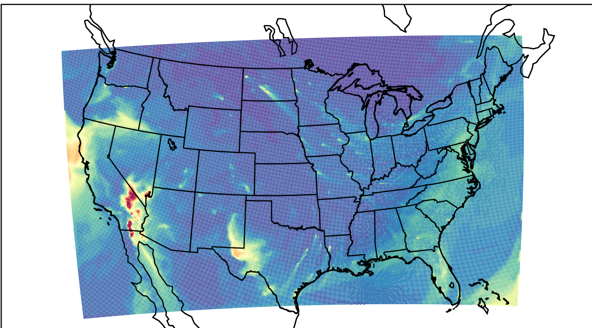
WRF 2024-01-14_13:00:00
