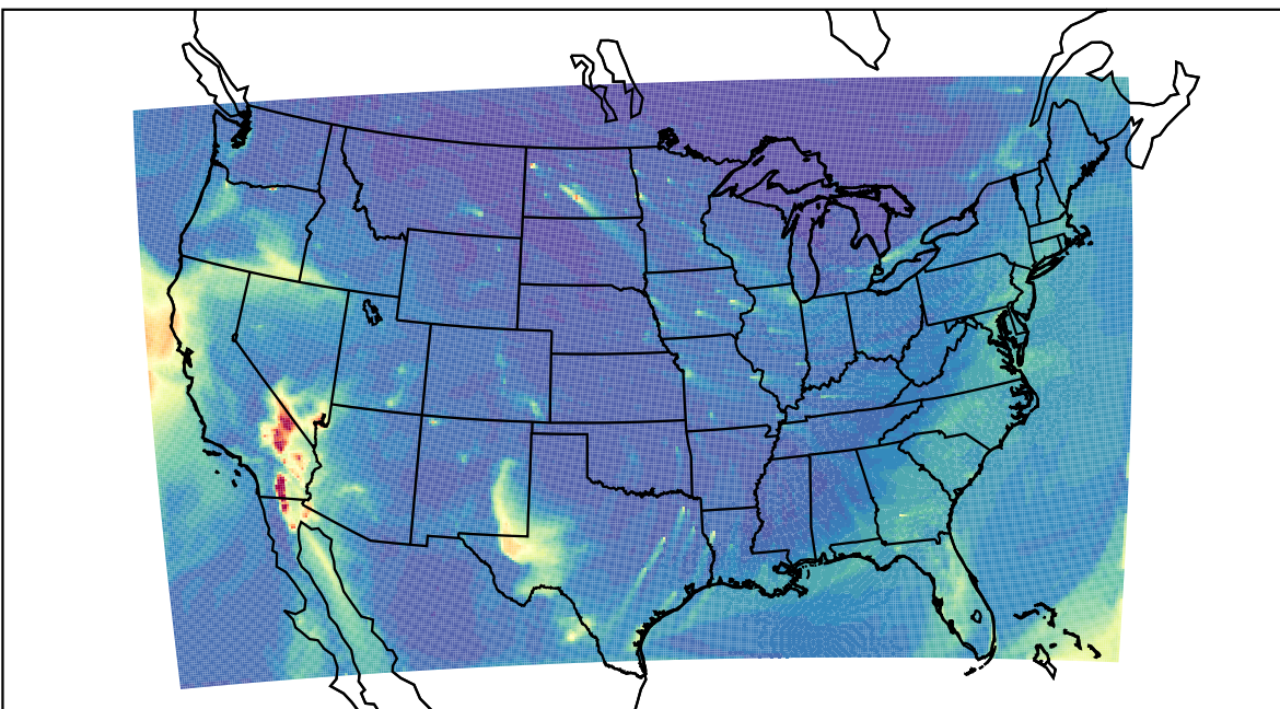
WRF 2024-01-14_14:00:00
