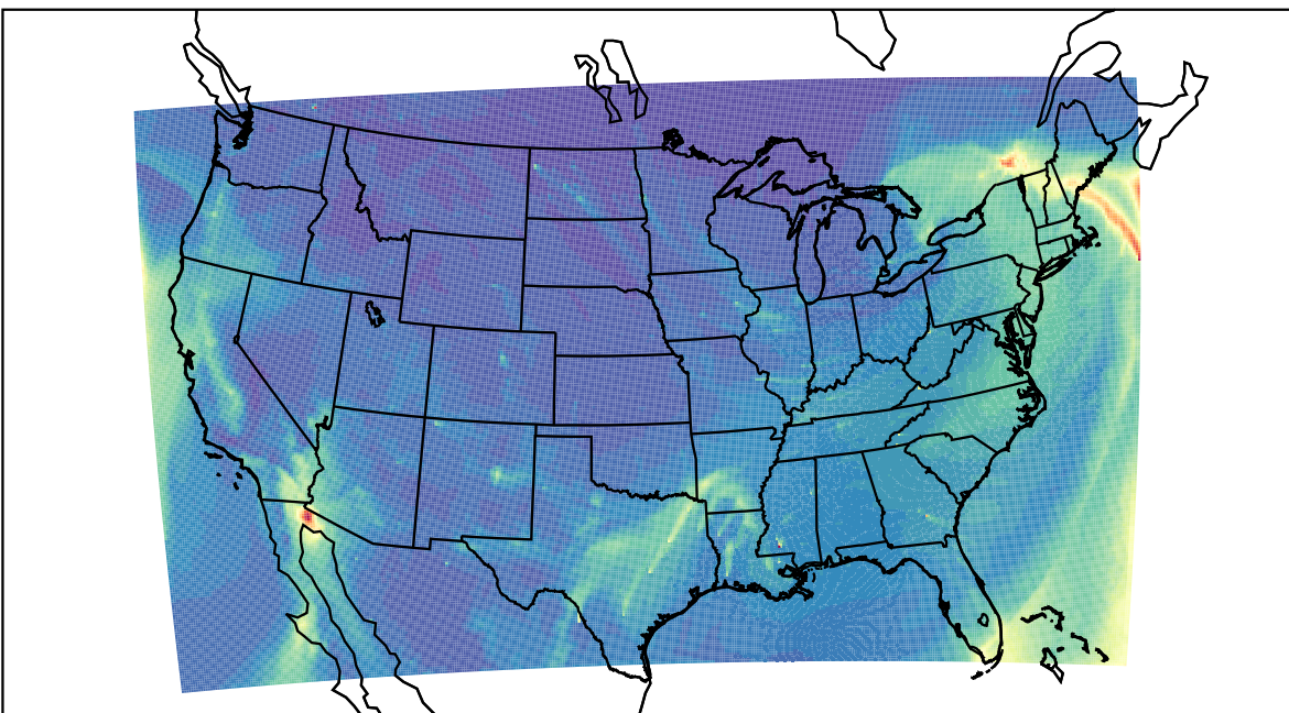
WRF 2024-01-13_19:00:00
