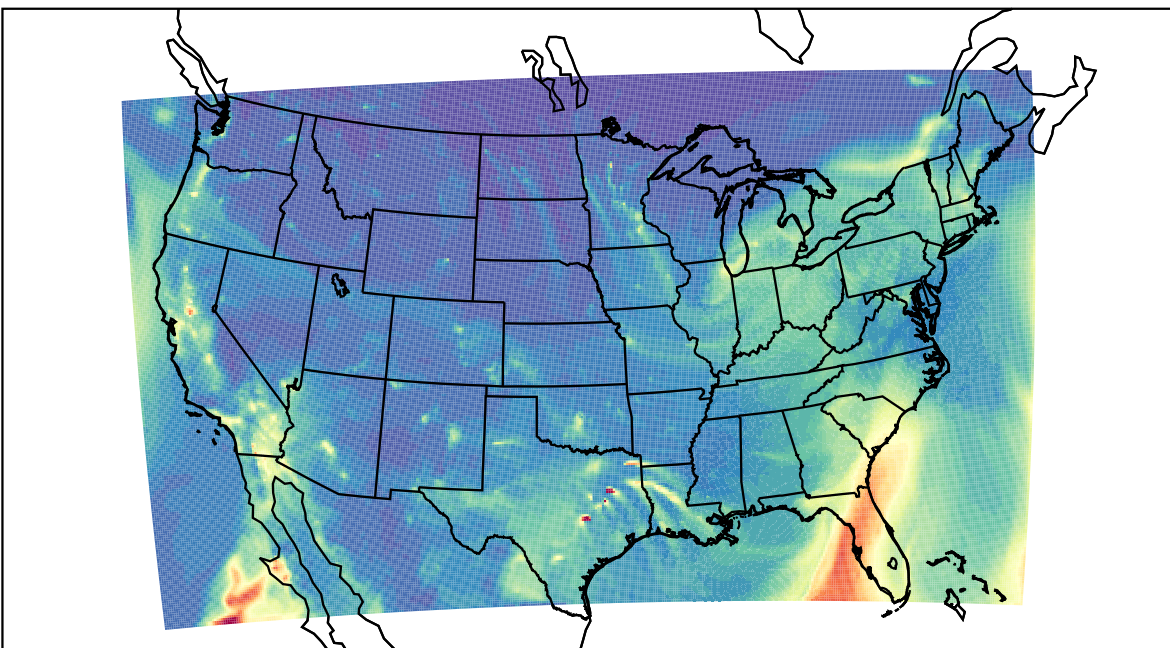
WRF 2024-01-13_05:00:00
