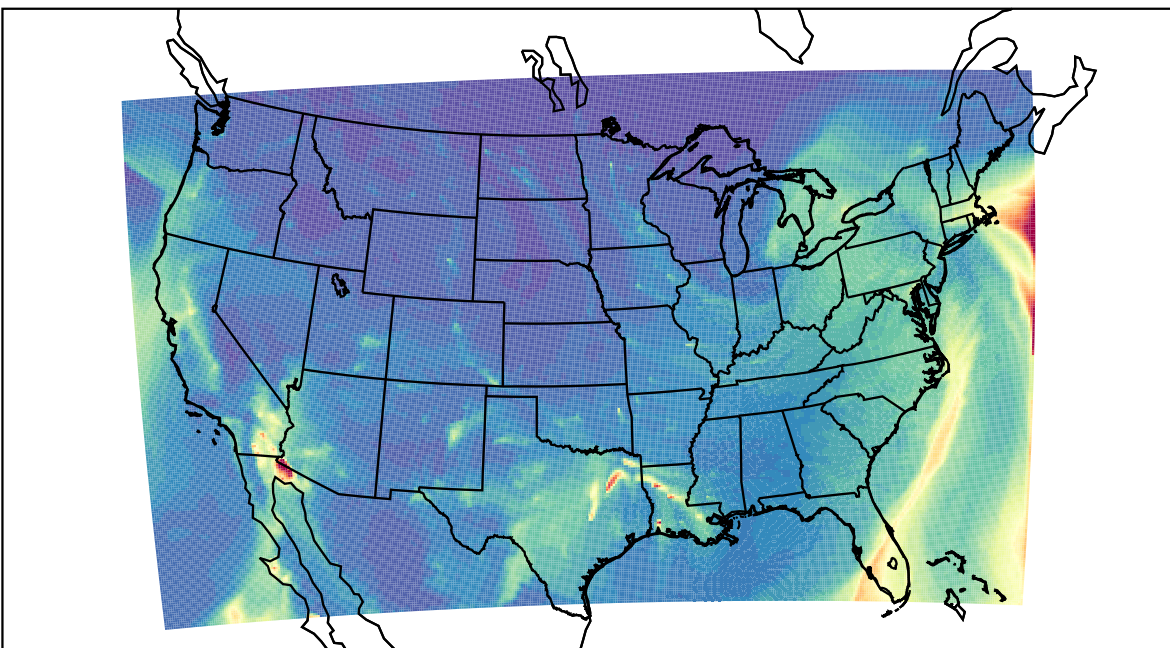
WRF 2024-01-13_12:00:00
