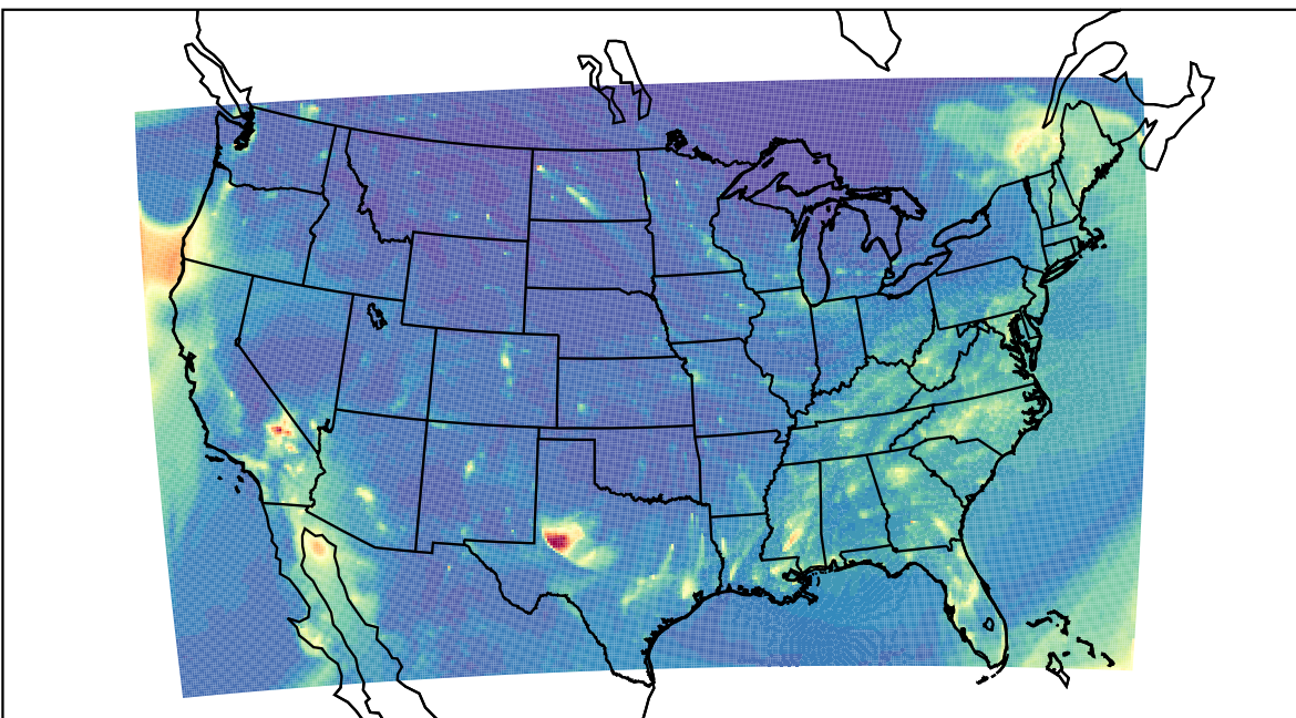
WRF 2024-01-14_03:00:00
