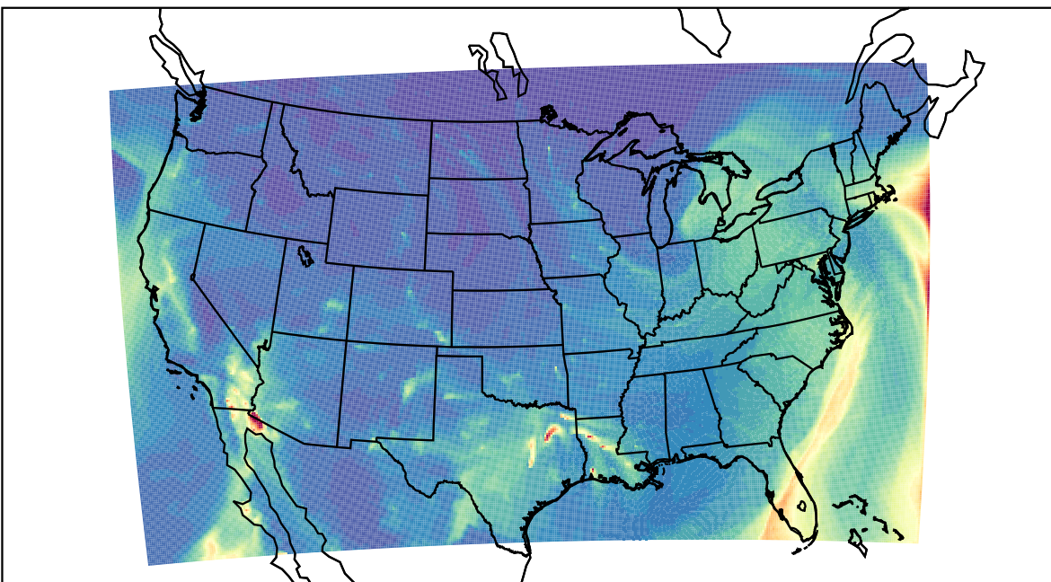
WRF 2024-01-13_11:00:00
