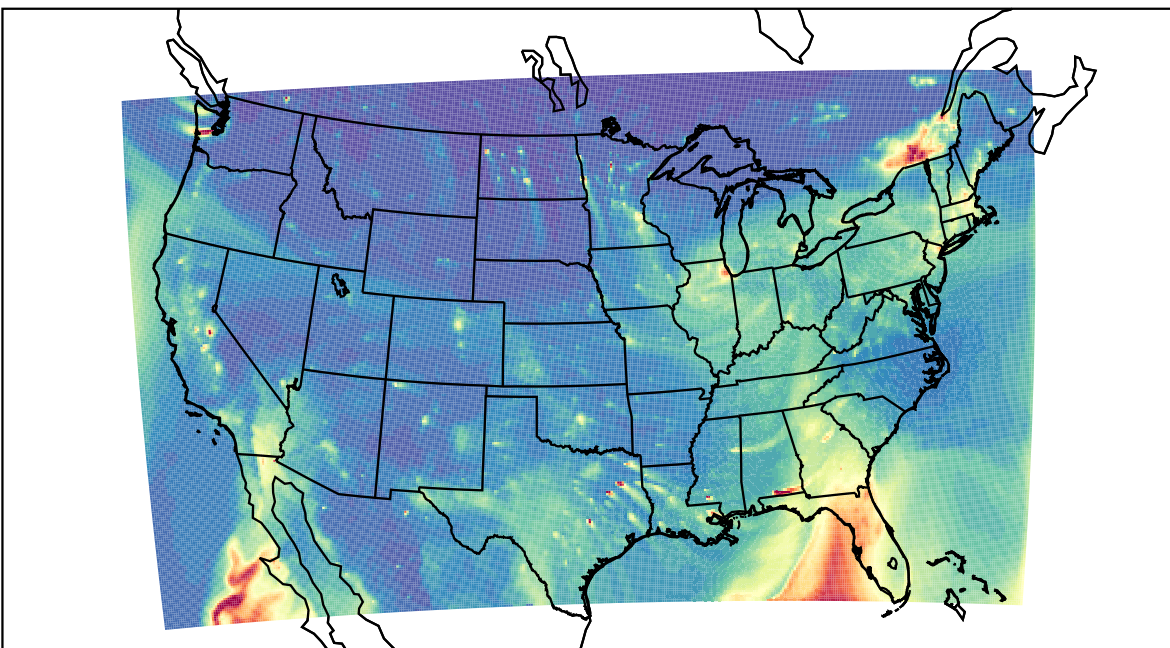
WRF 2024-01-13_01:00:00
