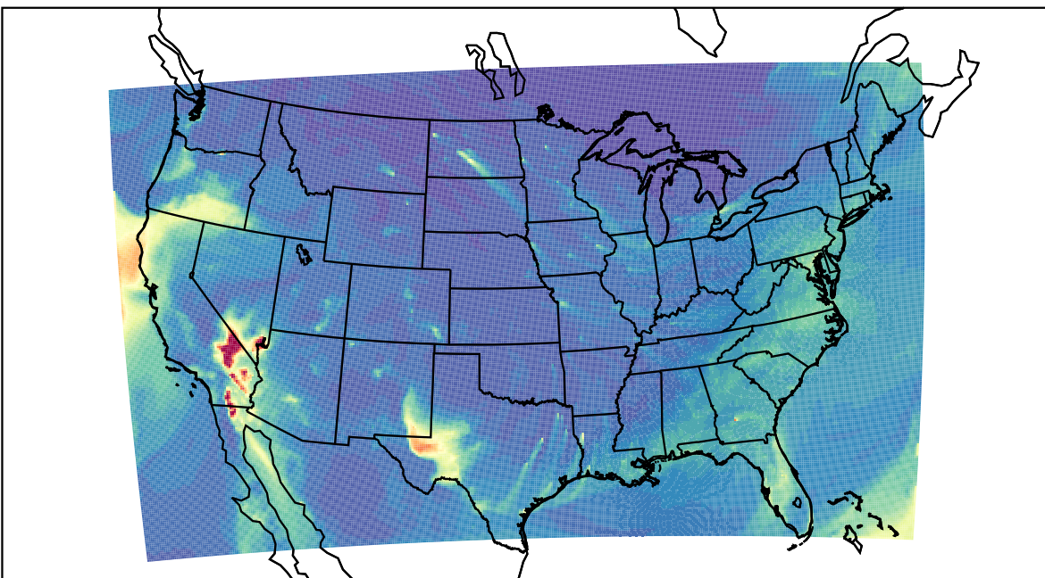
WRF 2024-01-14_11:00:00
