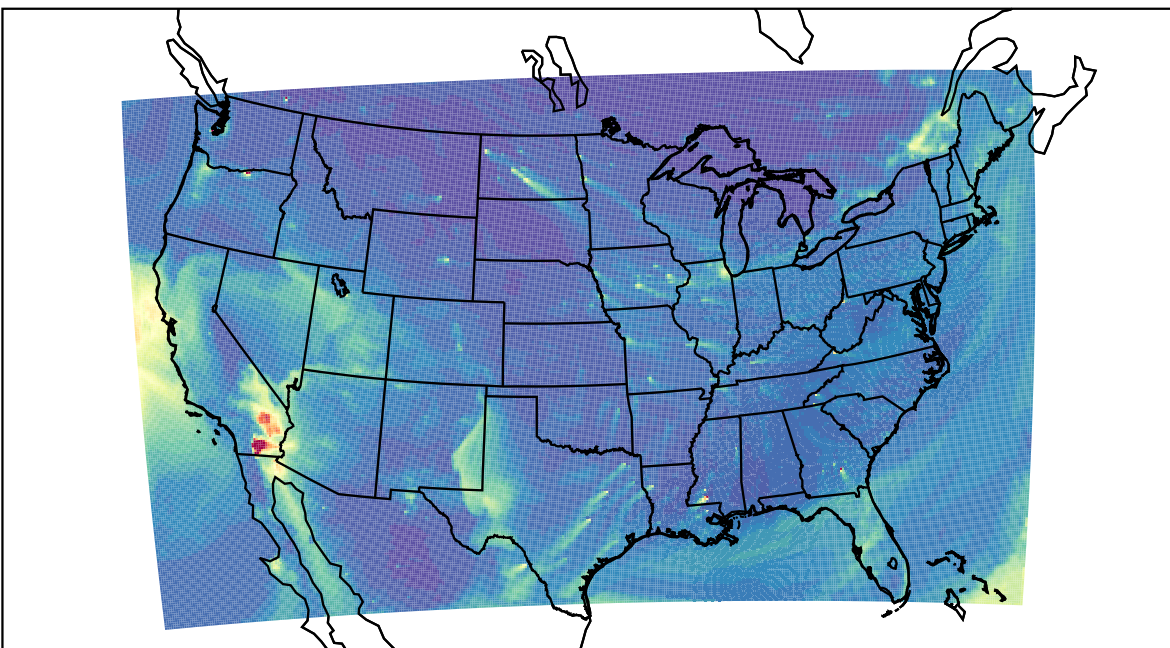
WRF 2024-01-14_22:00:00
