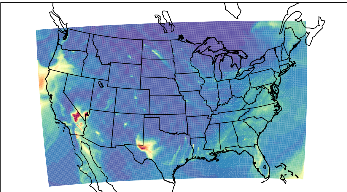
WRF 2024-01-14_08:00:00
