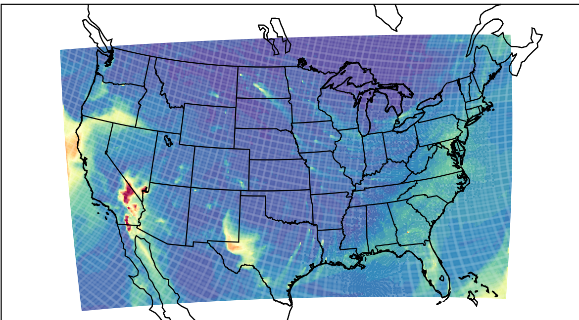
WRF 2024-01-14_12:00:00
