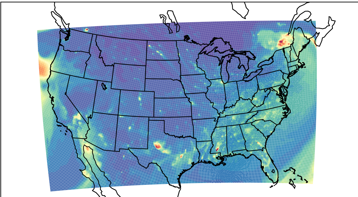
WRF 2024-01-14_01:00:00
