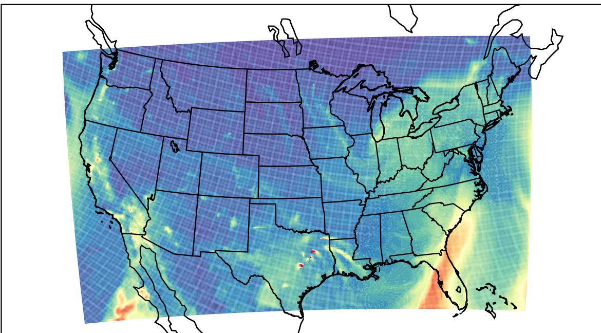
WRF 2024-01-13_06:00:00
