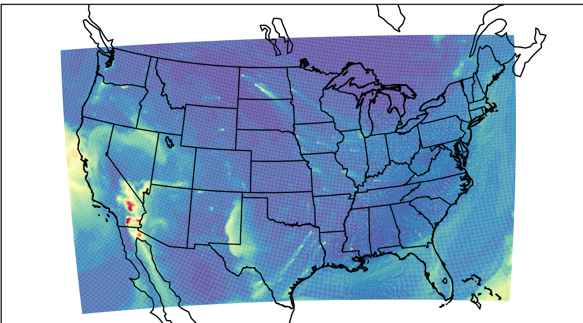
WRF 2024-01-14_19:00:00
