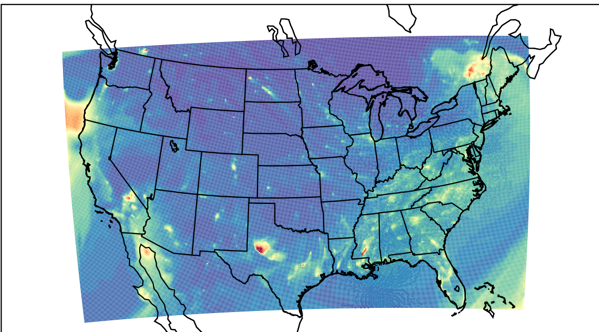
WRF 2024-01-14_02:00:00
