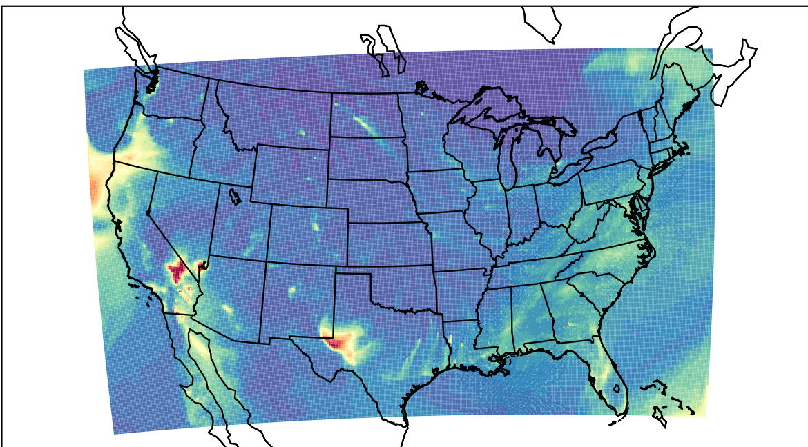
WRF 2024-01-14_07:00:00
