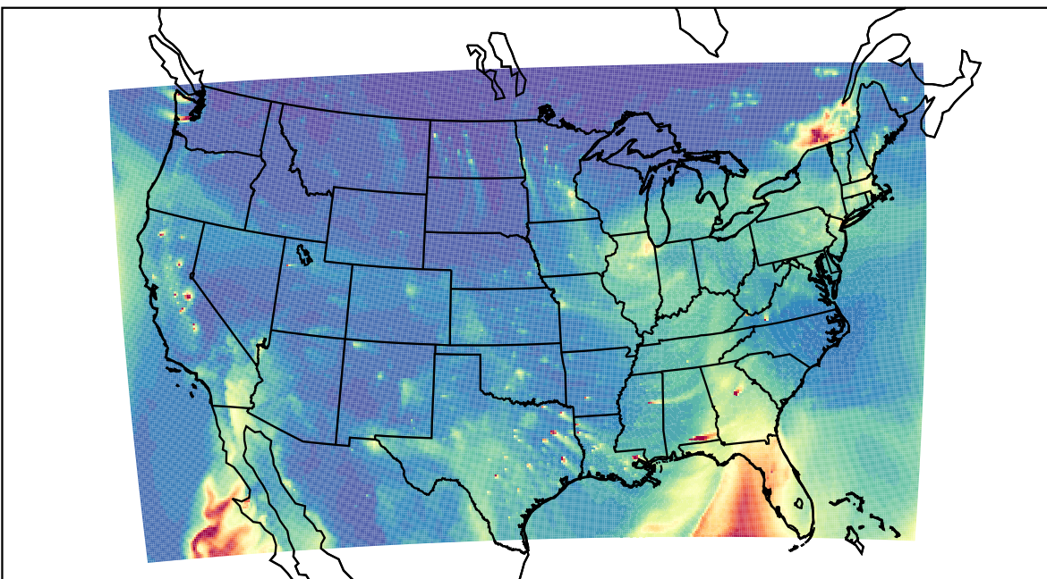
WRF 2024-01-13_00:00:00
