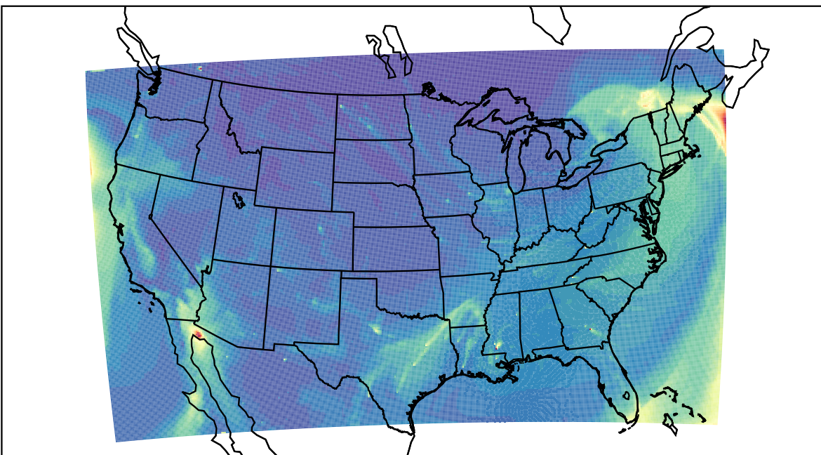
WRF 2024-01-13_21:00:00
