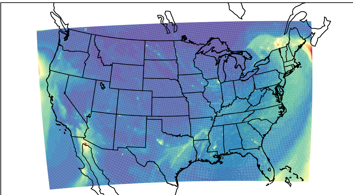
WRF 2024-01-13_22:00:00
