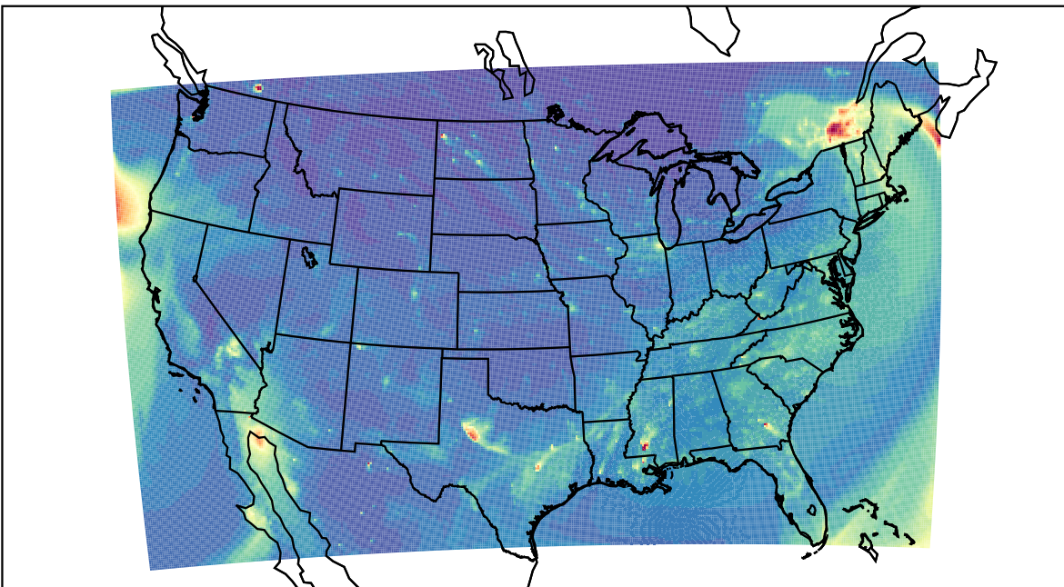
WRF 2024-01-14_00:00:00
