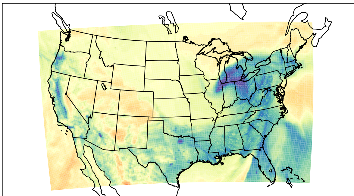
WRF (2024-01-13_05:00:00)
