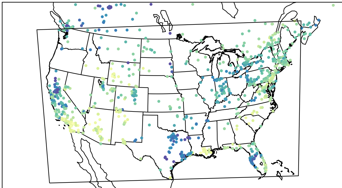
AirNOW (2024-01-14_20:00:00)
