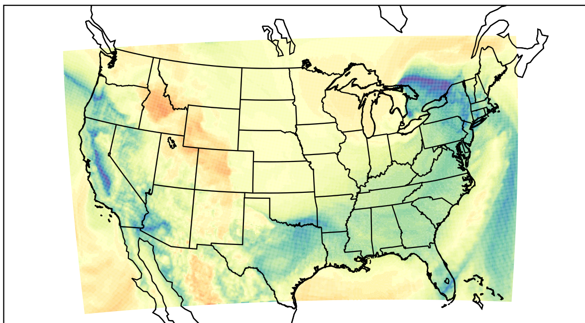
WRF (2024-01-13_17:00:00)
