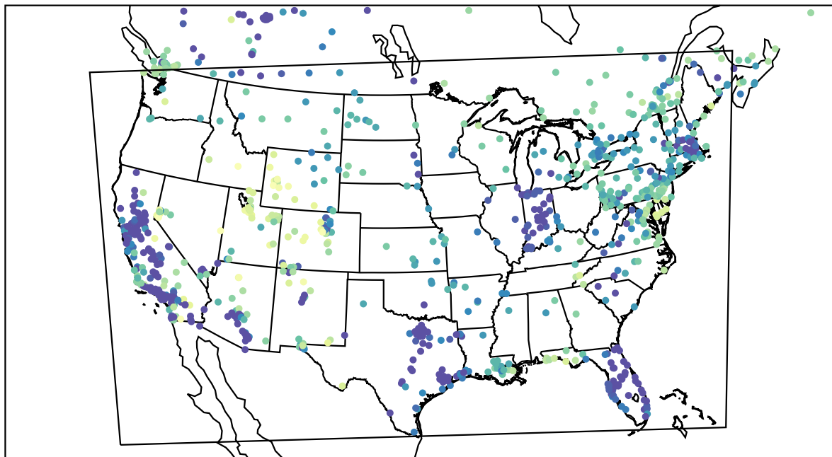
AirNOW (2024-01-13_03:00:00)
