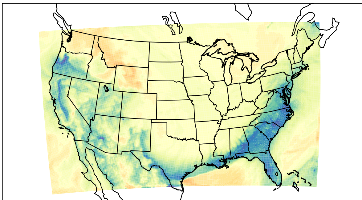
WRF (2024-01-14_12:00:00)
