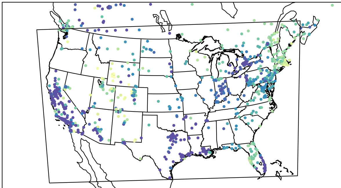
AirNOW (2024-01-13_13:00:00)
