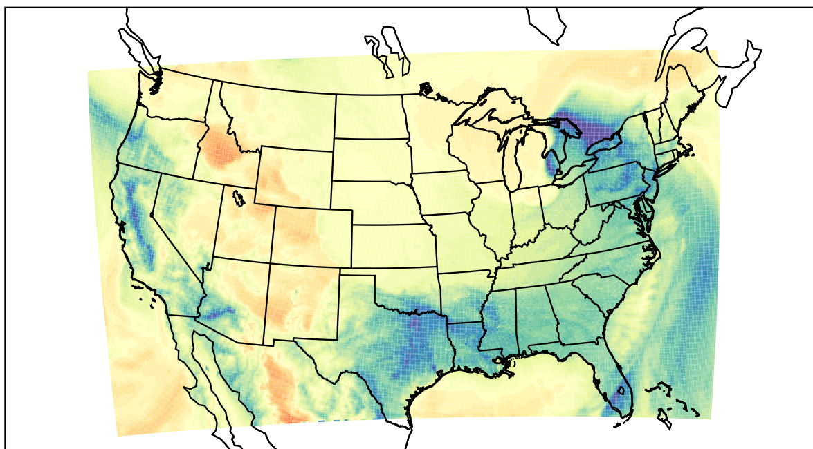
WRF (2024-01-13_14:00:00)
