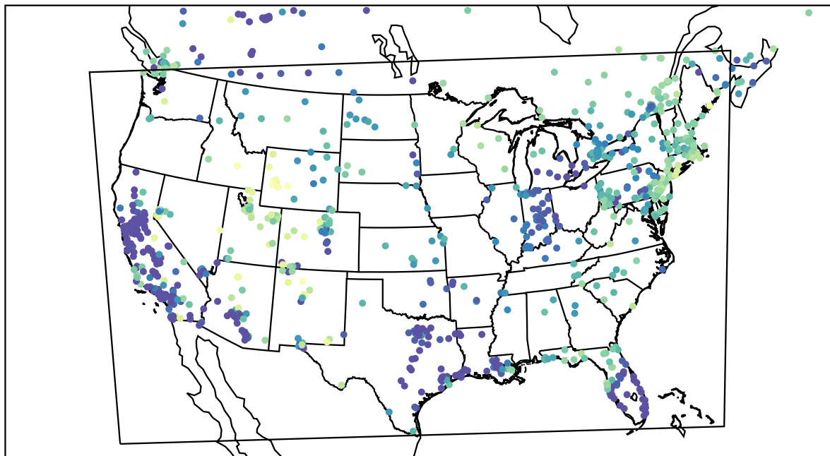
AirNOW (2024-01-13_09:00:00)
