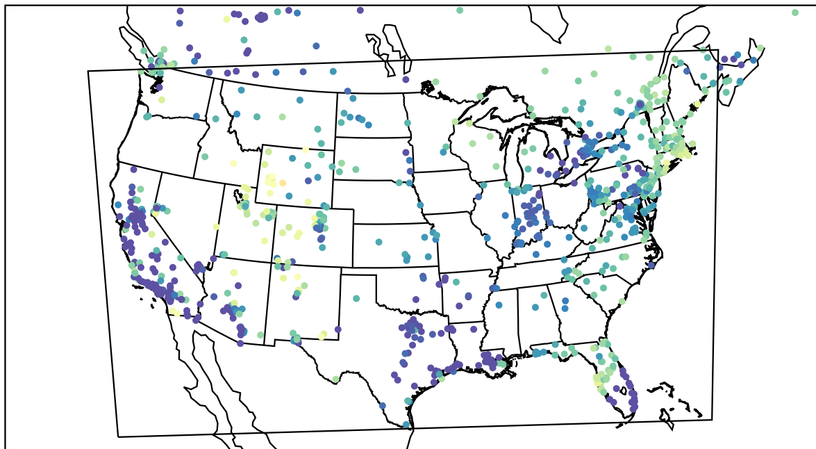
AirNOW (2024-01-13_11:00:00)
