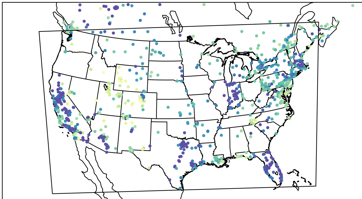
AirNOW (2024-01-13_02:00:00)
