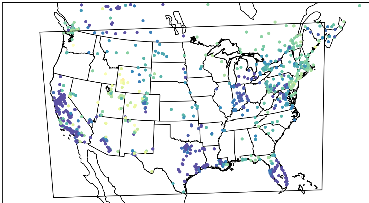
AirNOW (2024-01-13_08:00:00)
