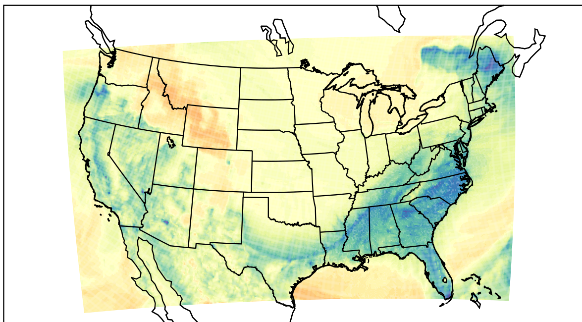
WRF (2024-01-14_03:00:00)
