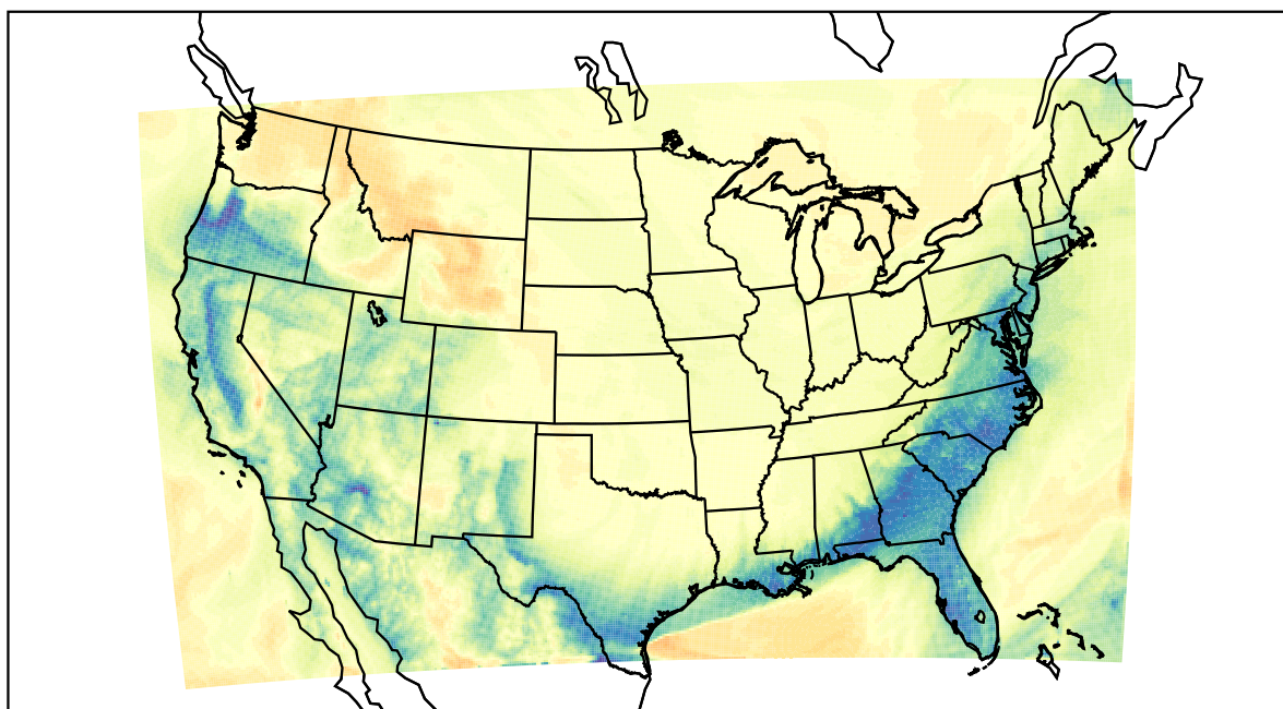
WRF (2024-01-14_13:00:00)
