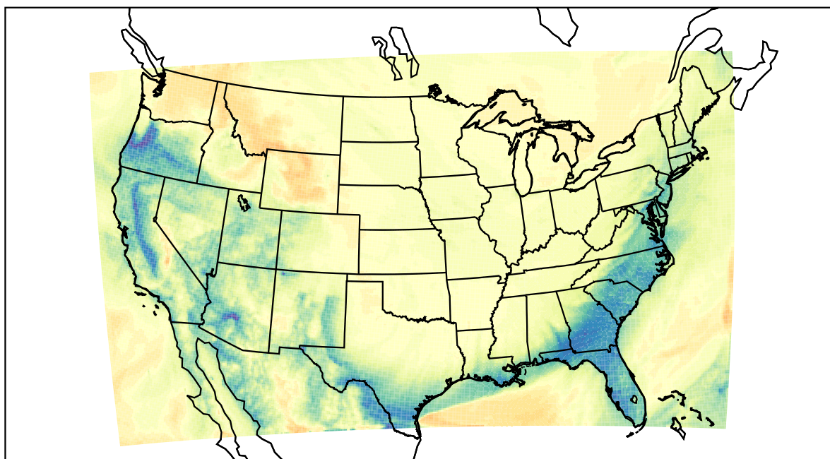
WRF (2024-01-14_14:00:00)
