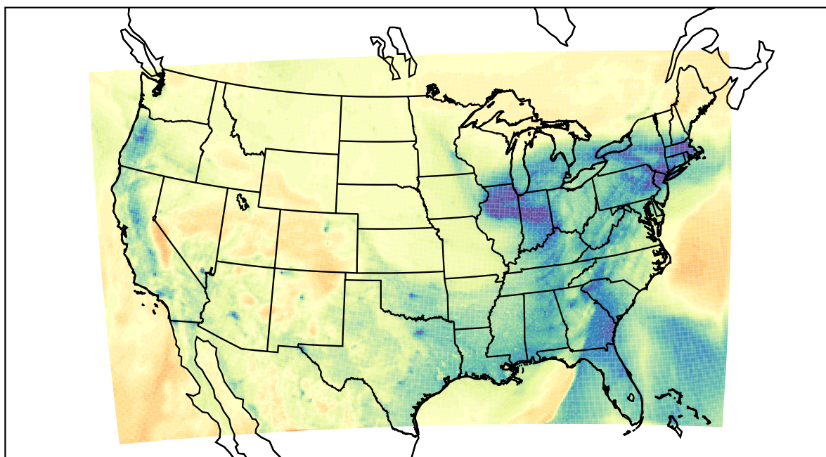
WRF (2024-01-13_01:00:00)
