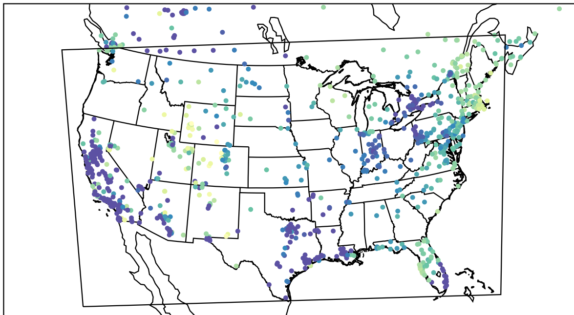
AirNOW (2024-01-13_14:00:00)
