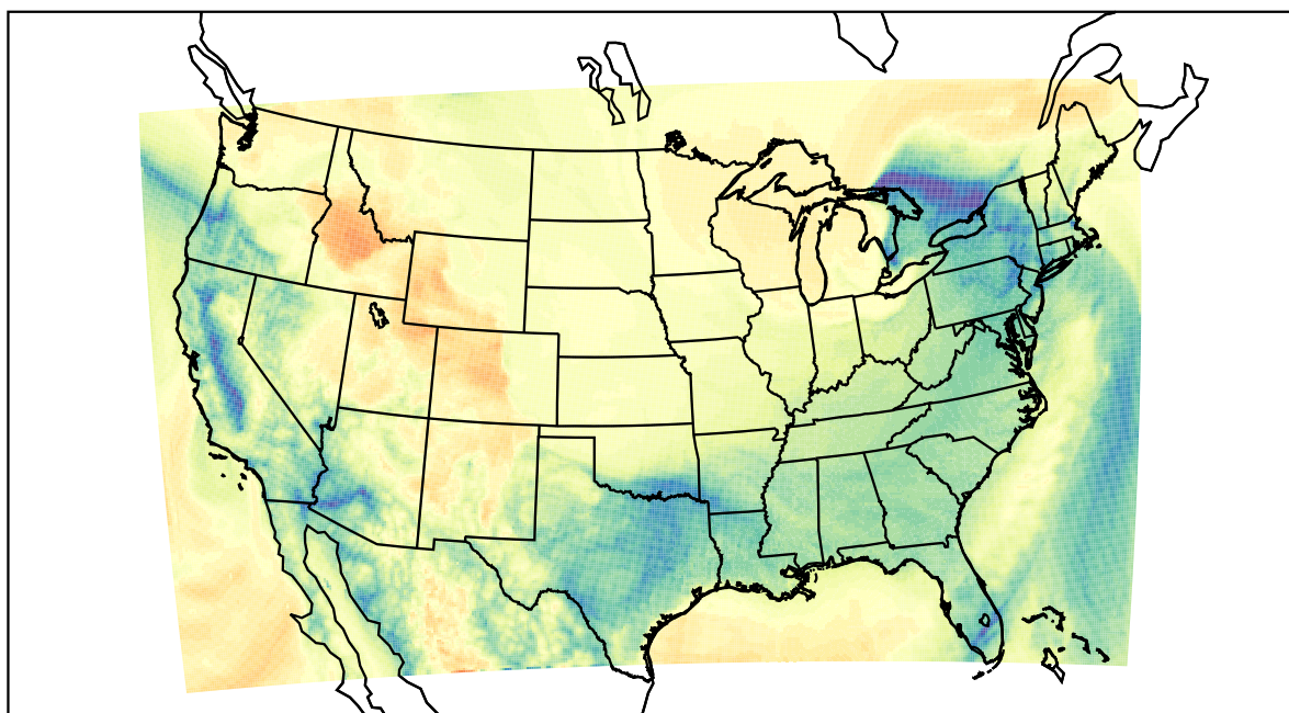
WRF (2024-01-13_16:00:00)
