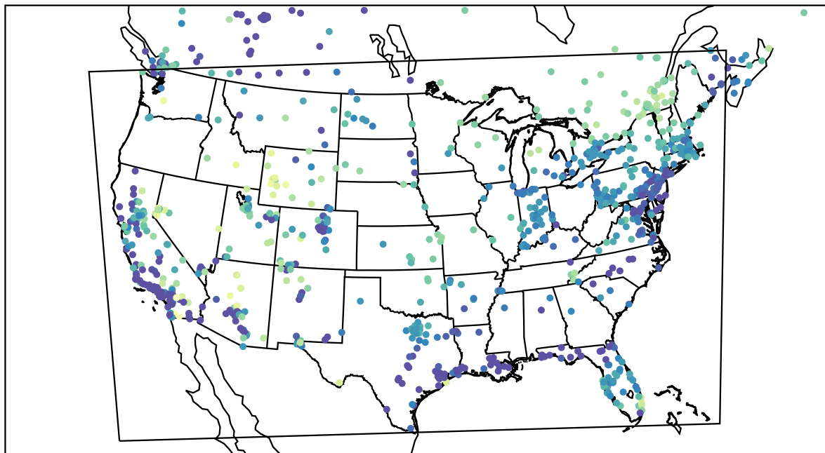
AirNOW (2024-01-14_11:00:00)
