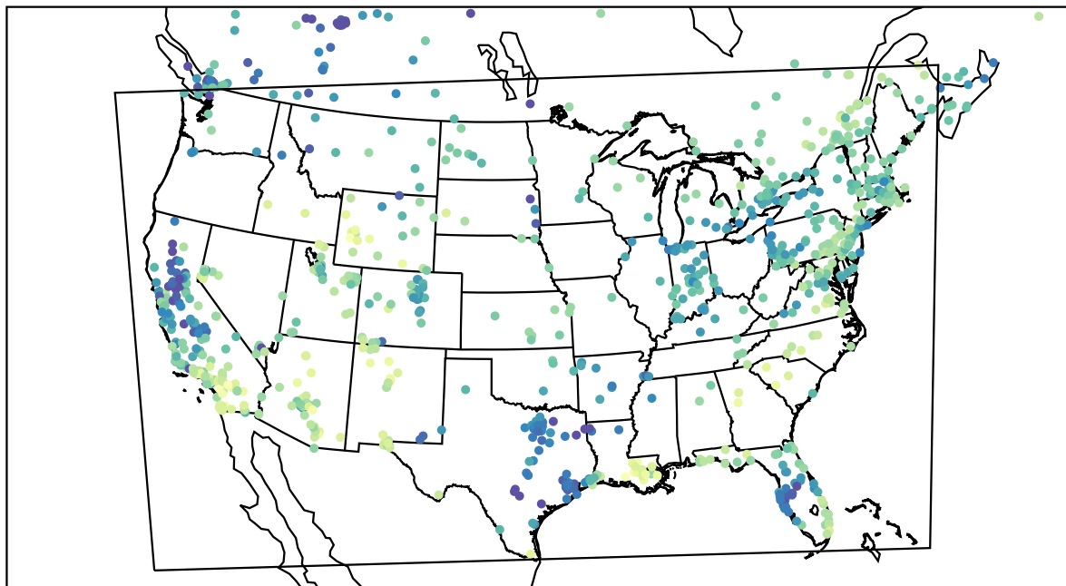
AirNOW (2024-01-14_19:00:00)
