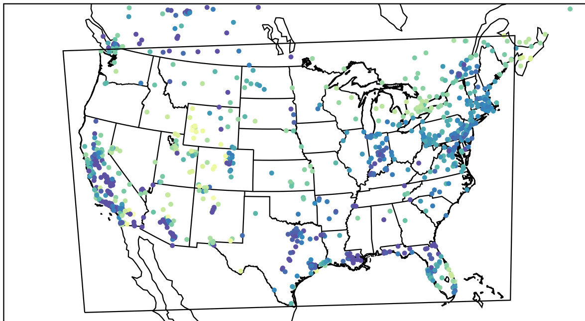
AirNOW (2024-01-14_03:00:00)
