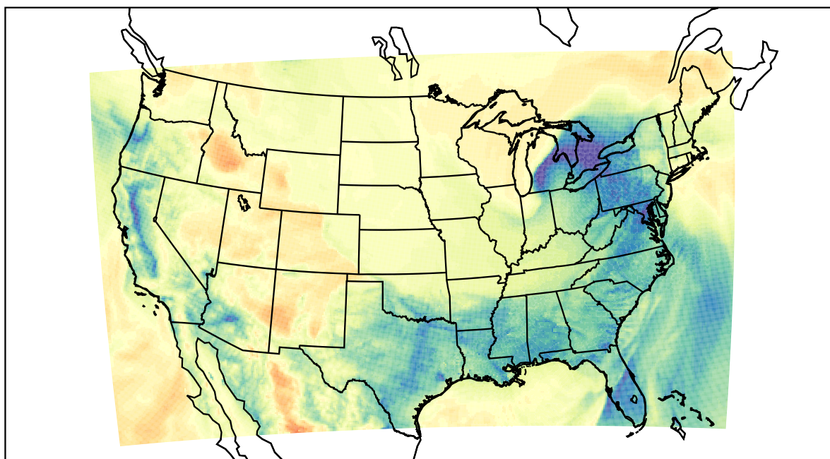
WRF (2024-01-13_10:00:00)
