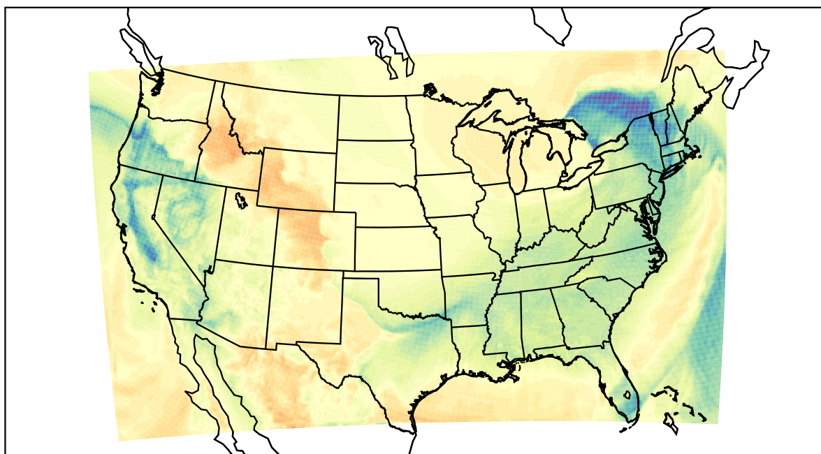
WRF (2024-01-13_20:00:00)
