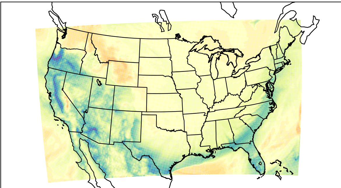
WRF (2024-01-14_16:00:00)
