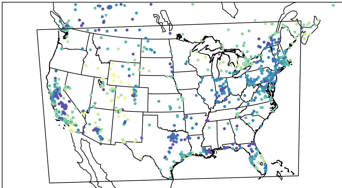
AirNOW (2024-01-14_01:00:00)
