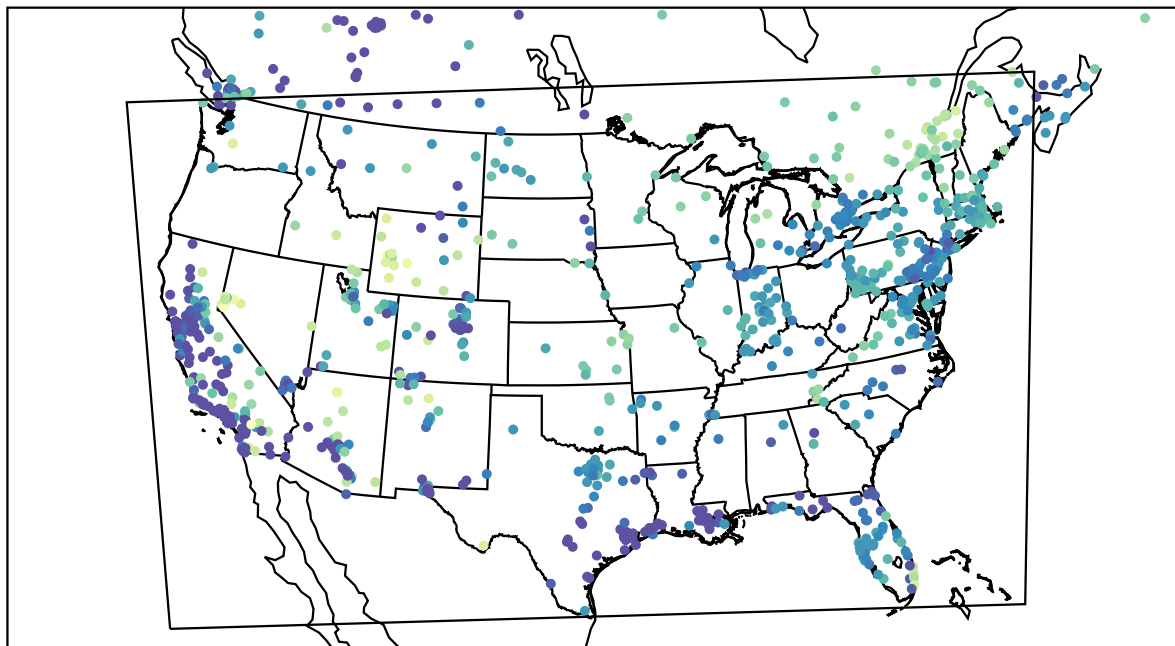
AirNOW (2024-01-14_14:00:00)
