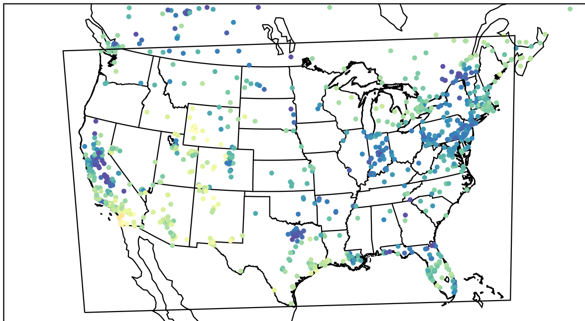
AirNOW (2024-01-13_23:00:00)
