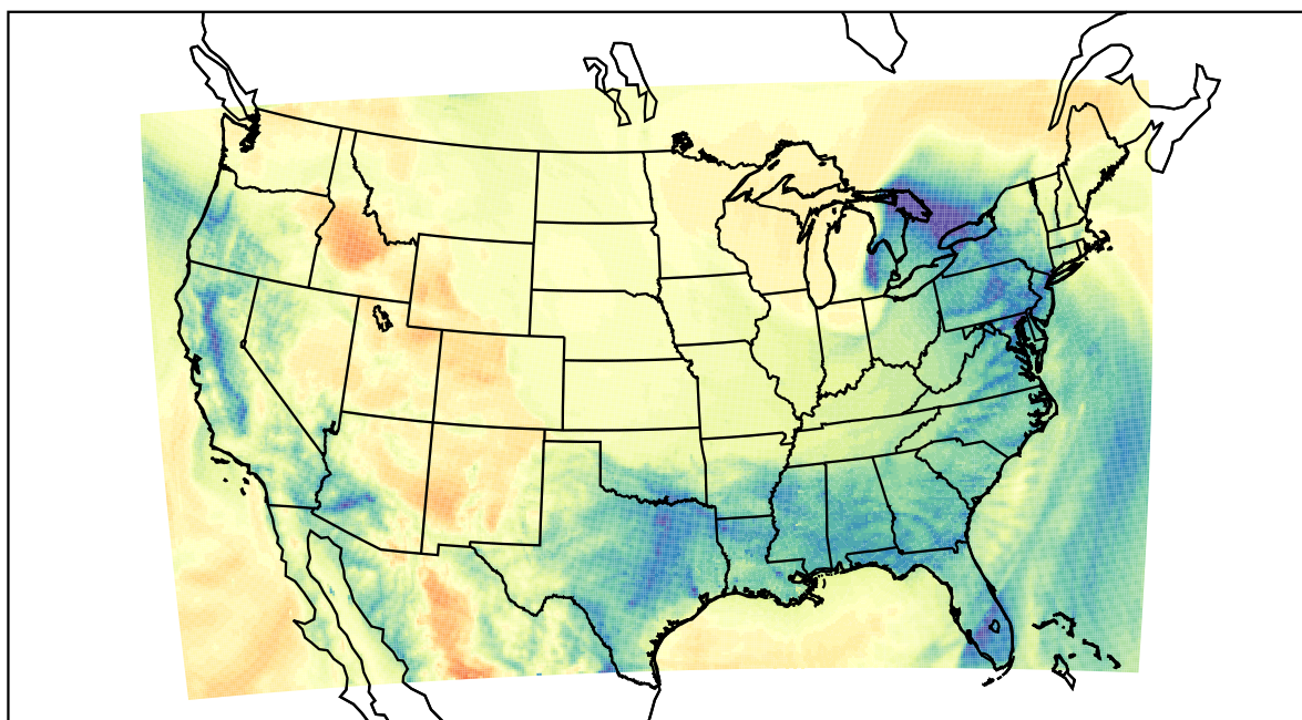
WRF (2024-01-13_13:00:00)
