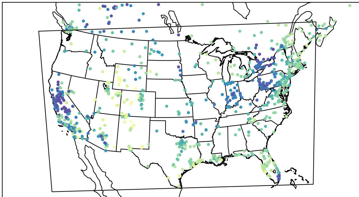
AirNOW (2024-01-13_18:00:00)
