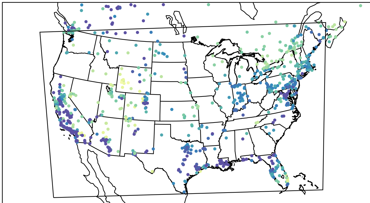
AirNOW (2024-01-14_07:00:00)
