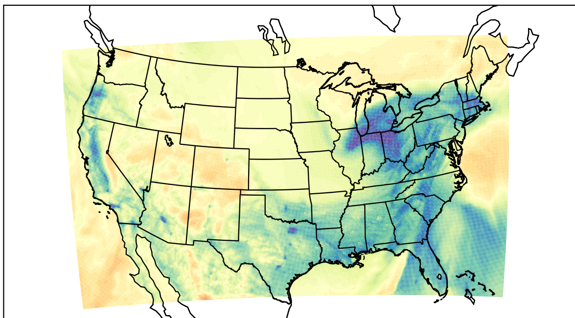
WRF (2024-01-13_04:00:00)
