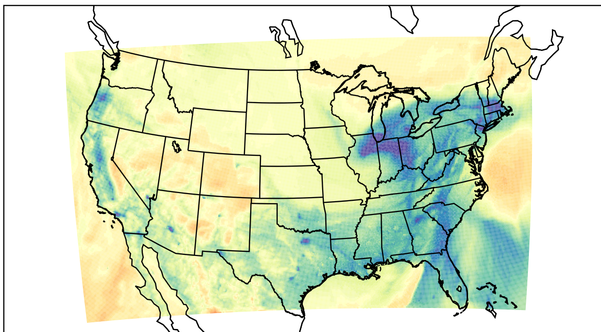
WRF (2024-01-13_03:00:00)
