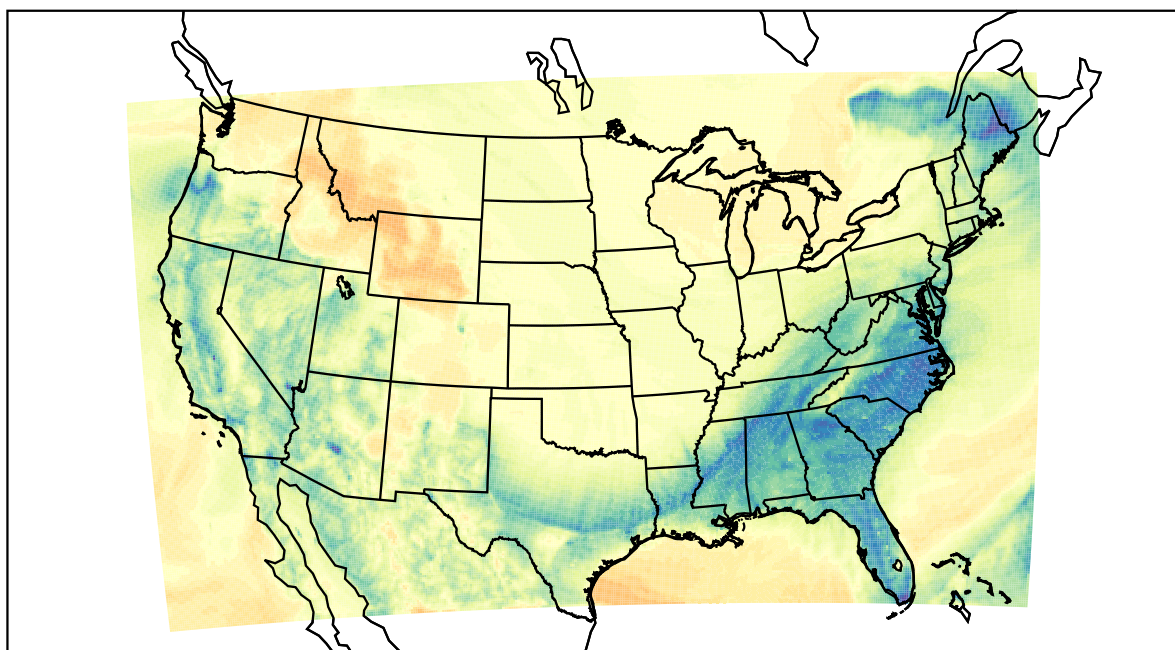
WRF (2024-01-14_04:00:00)
