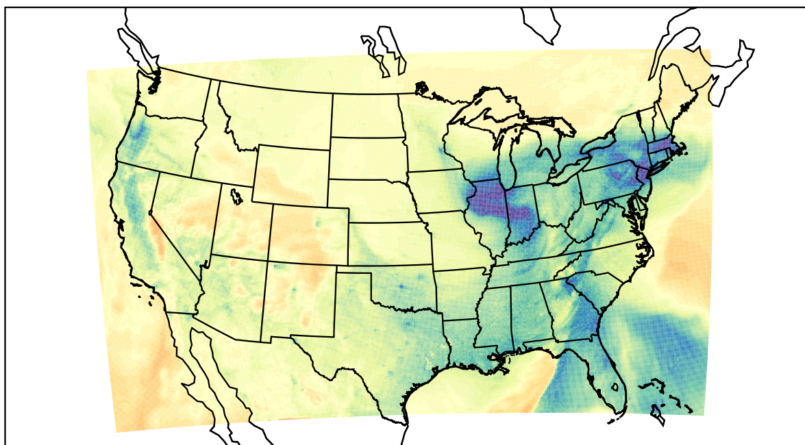
WRF (2024-01-13_00:00:00)
