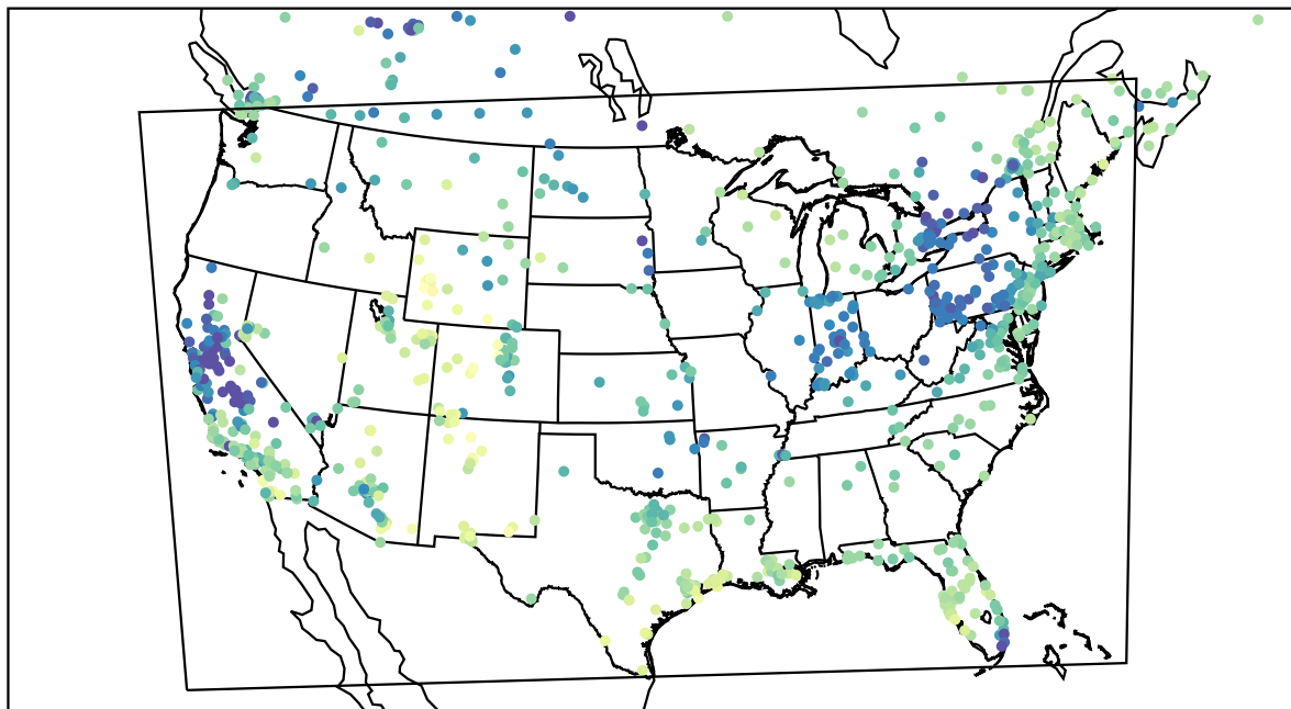
AirNOW (2024-01-13_19:00:00)
