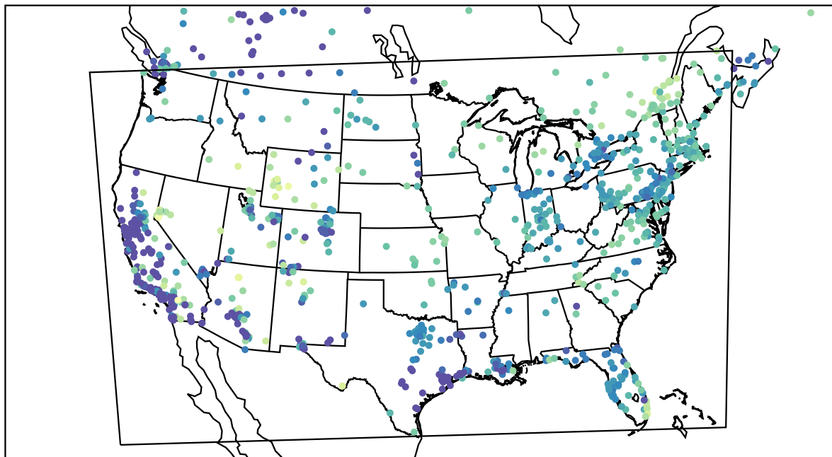
AirNOW (2024-01-14_15:00:00)
