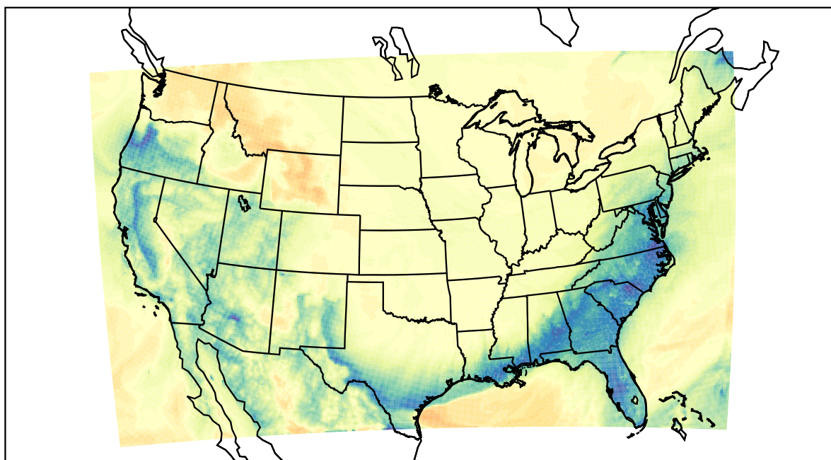
WRF (2024-01-14_11:00:00)
