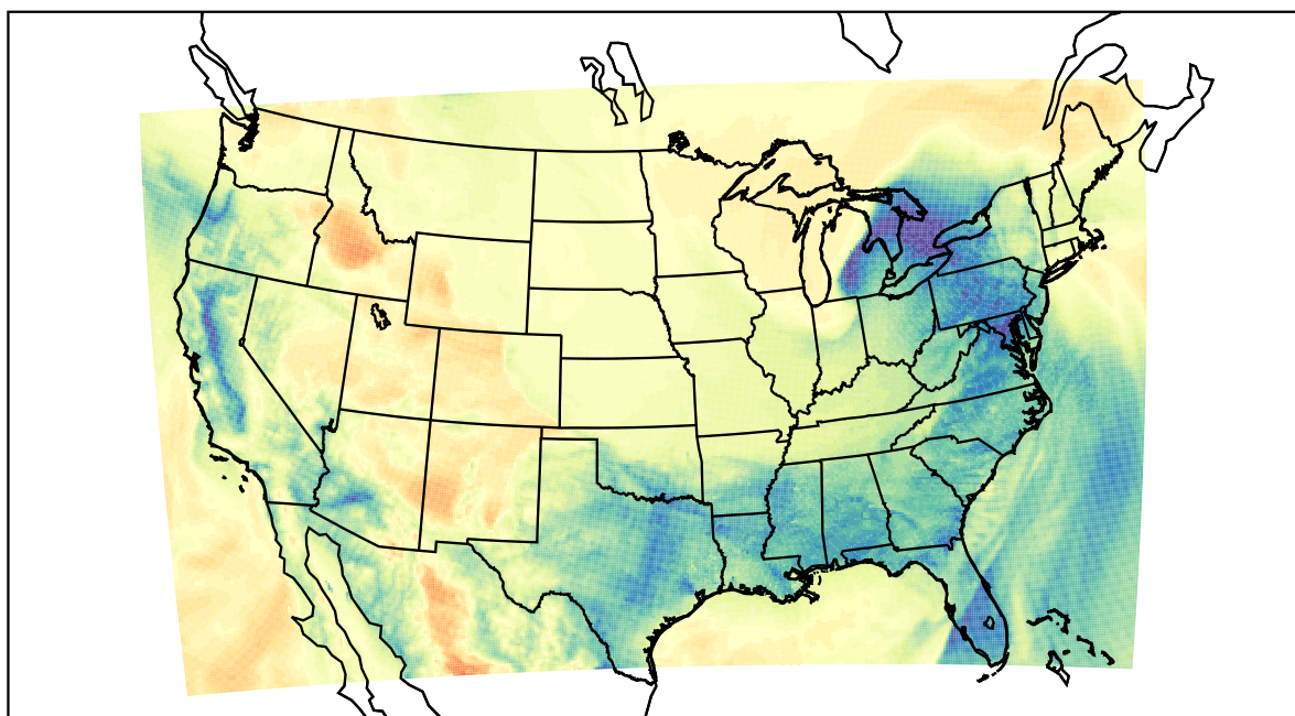
WRF (2024-01-13_11:00:00)
