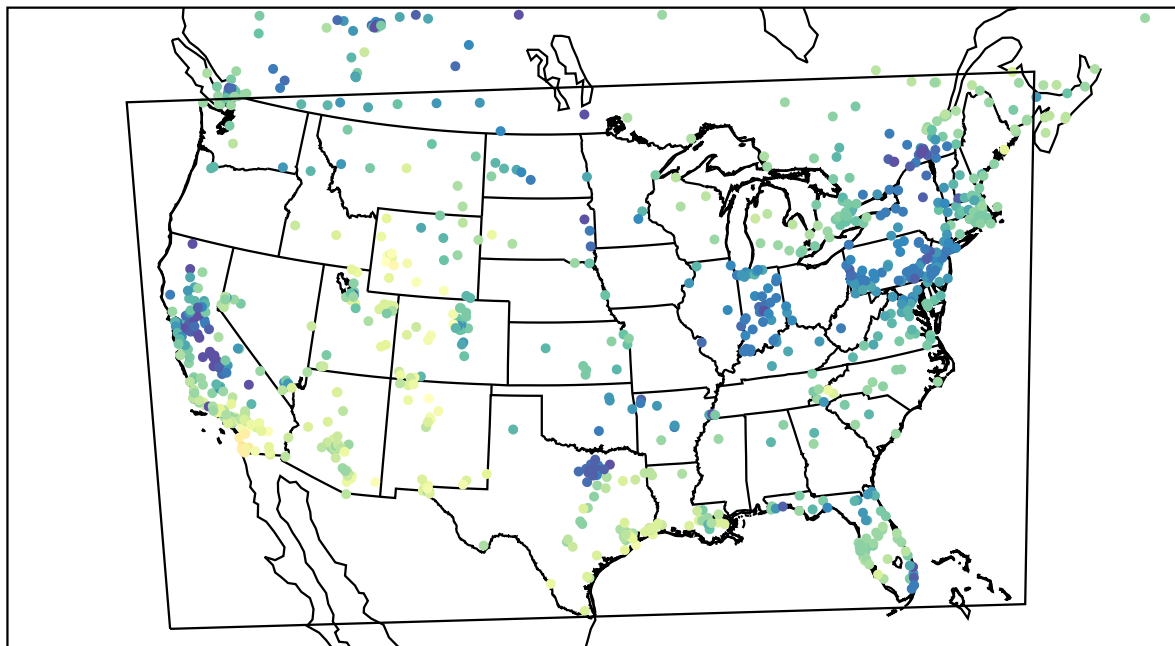
AirNOW (2024-01-13_22:00:00)
