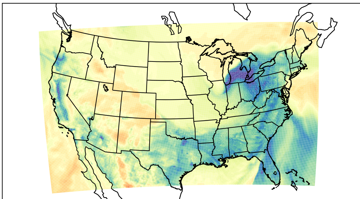
WRF (2024-01-13_07:00:00)
