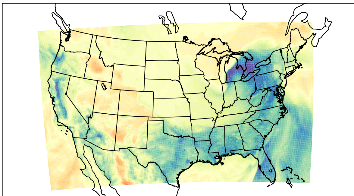
WRF (2024-01-13_09:00:00)
