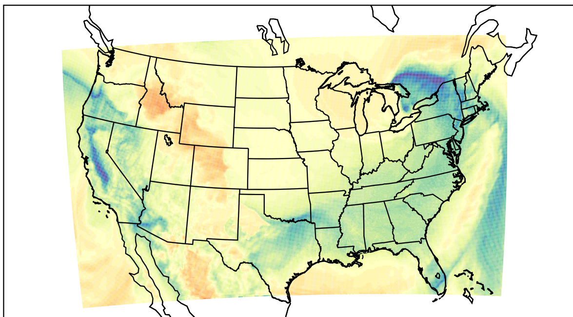
WRF (2024-01-13_18:00:00)
