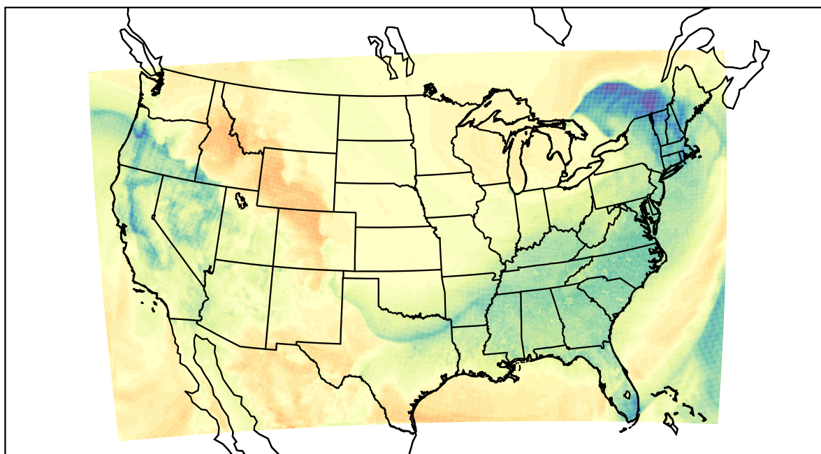
WRF (2024-01-13_22:00:00)
