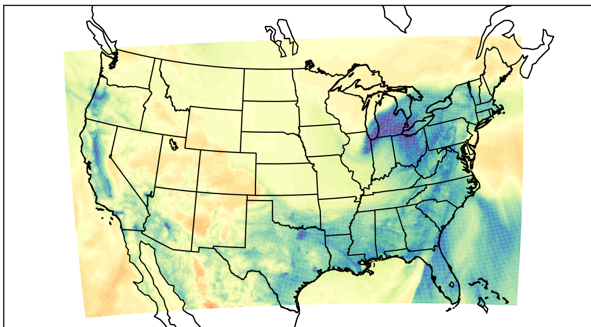
WRF (2024-01-13_06:00:00)
