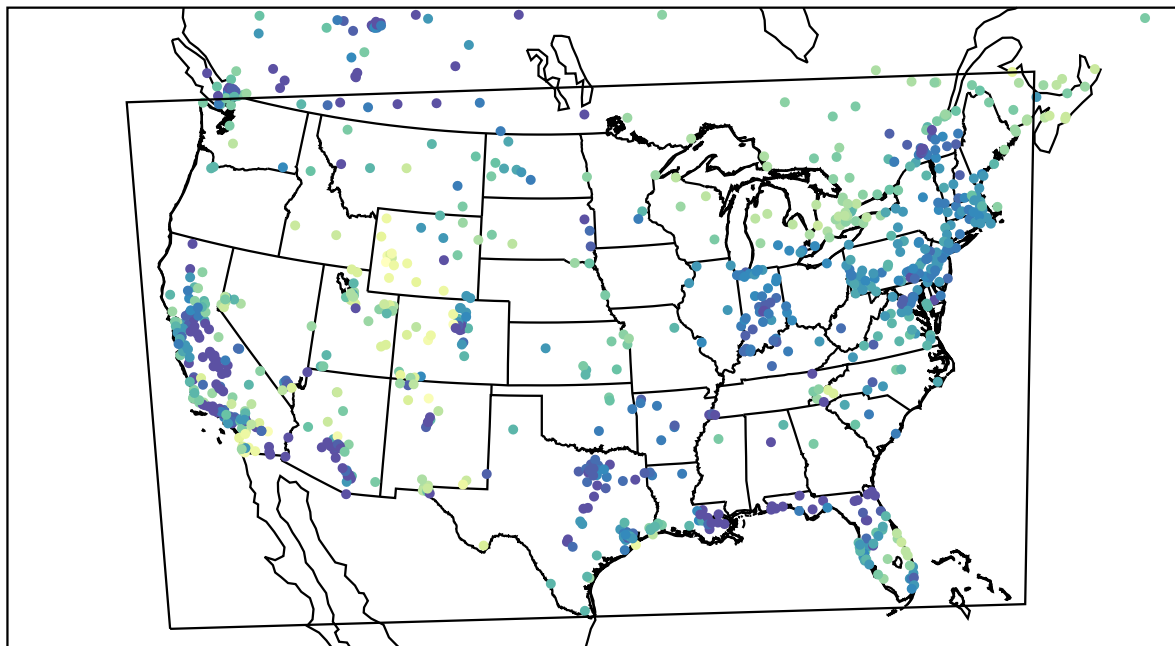
AirNOW (2024-01-14_02:00:00)
