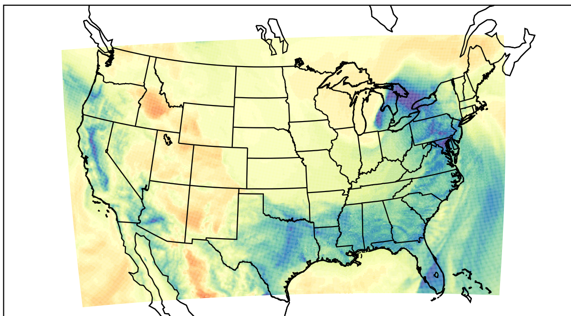
WRF (2024-01-13_12:00:00)
