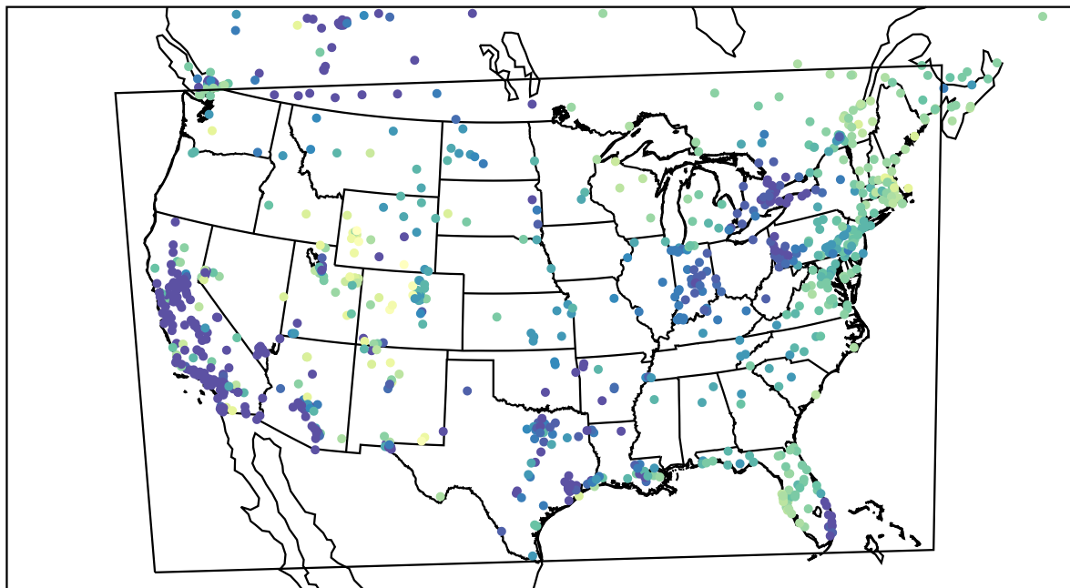
AirNOW (2024-01-13_15:00:00)
