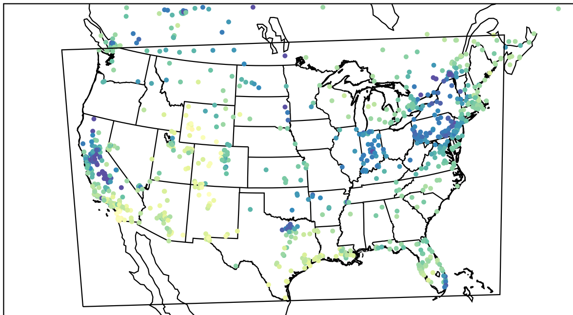
AirNOW (2024-01-13_21:00:00)
