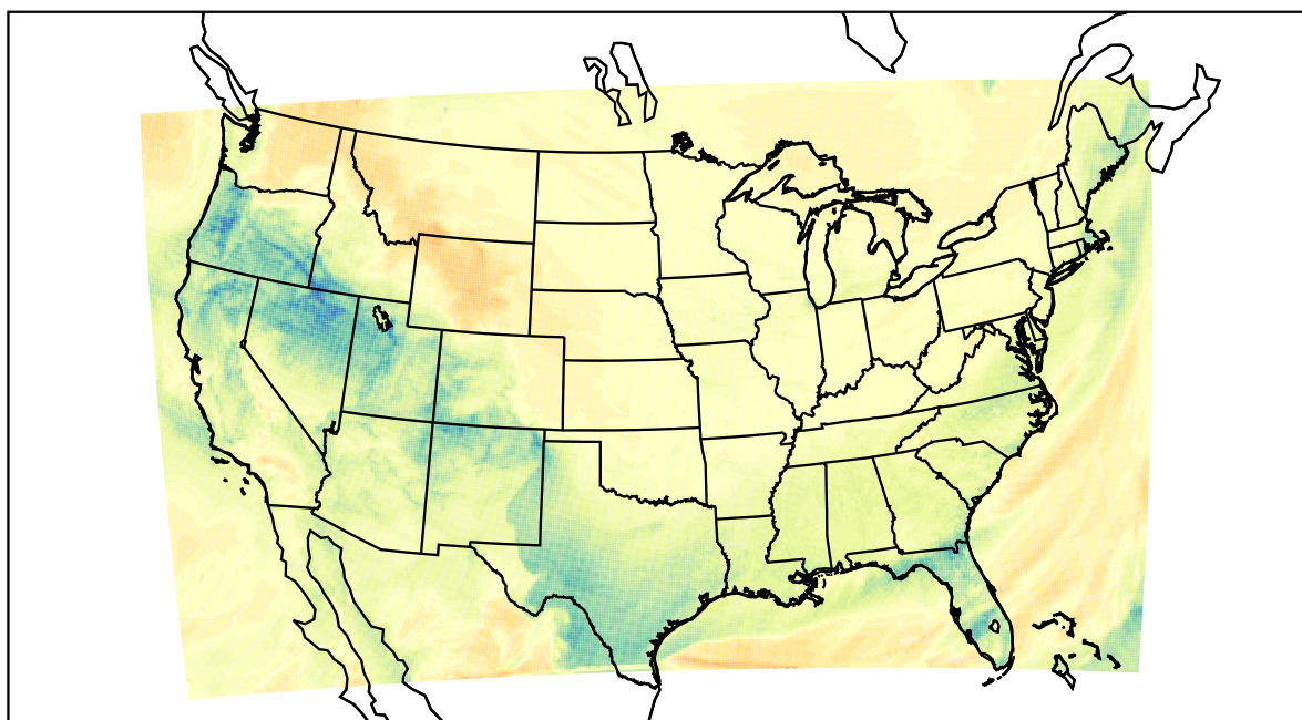
WRF (2024-01-14_22:00:00)
