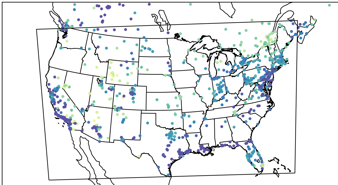
AirNOW (2024-01-14_12:00:00)
