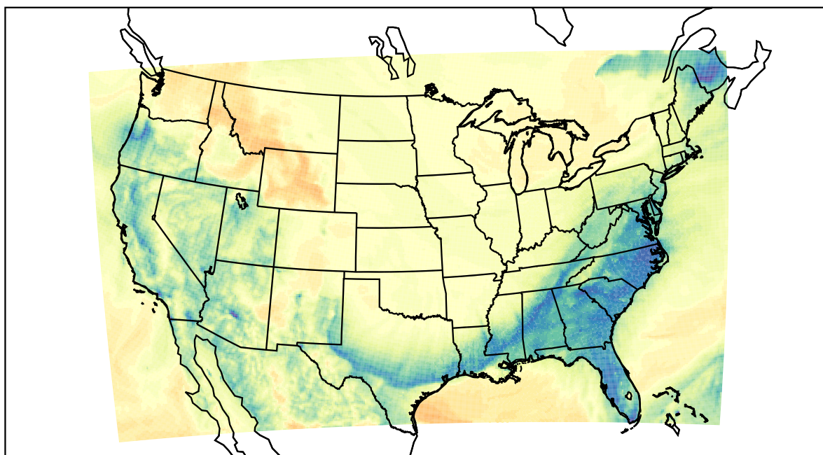
WRF (2024-01-14_07:00:00)
