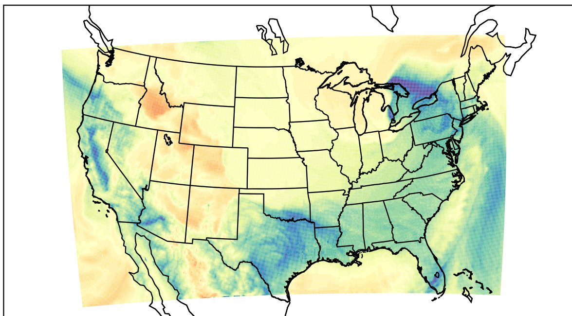
WRF (2024-01-13_15:00:00)
