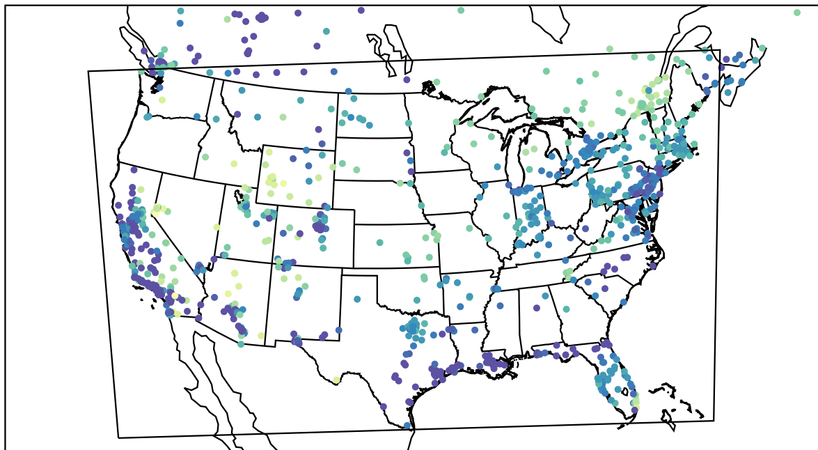
AirNOW (2024-01-14_13:00:00)
