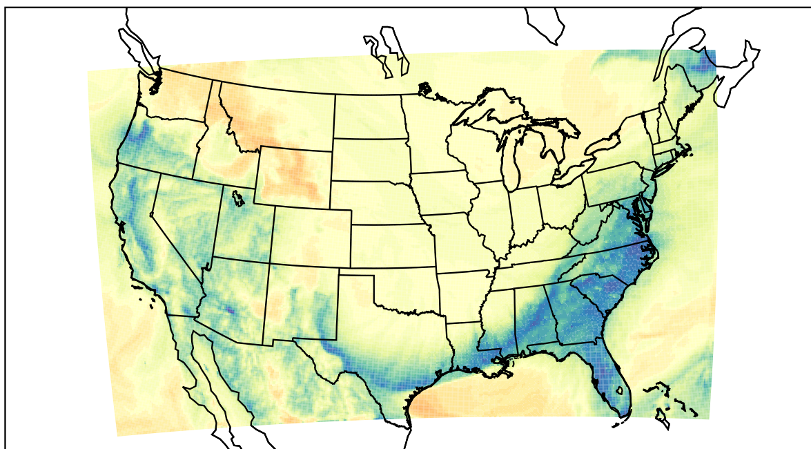
WRF (2024-01-14_09:00:00)
