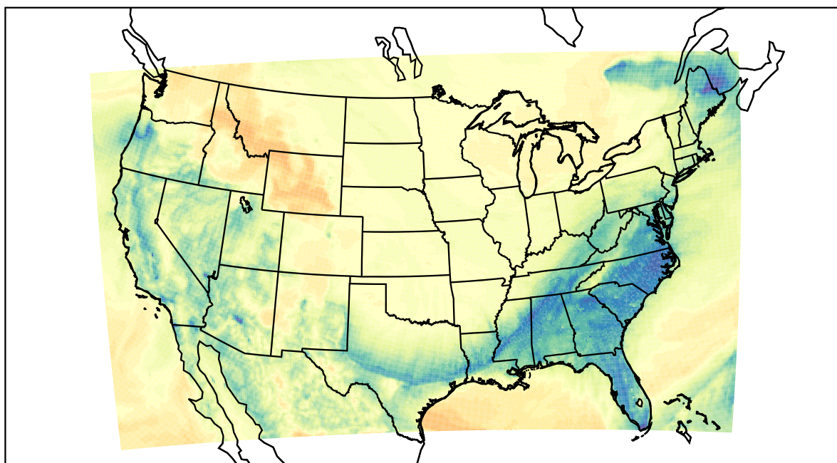
WRF (2024-01-14_05:00:00)
