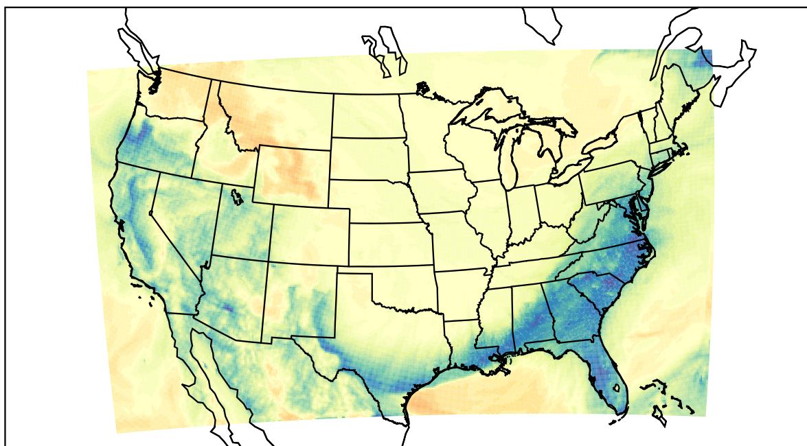
WRF (2024-01-14_10:00:00)
