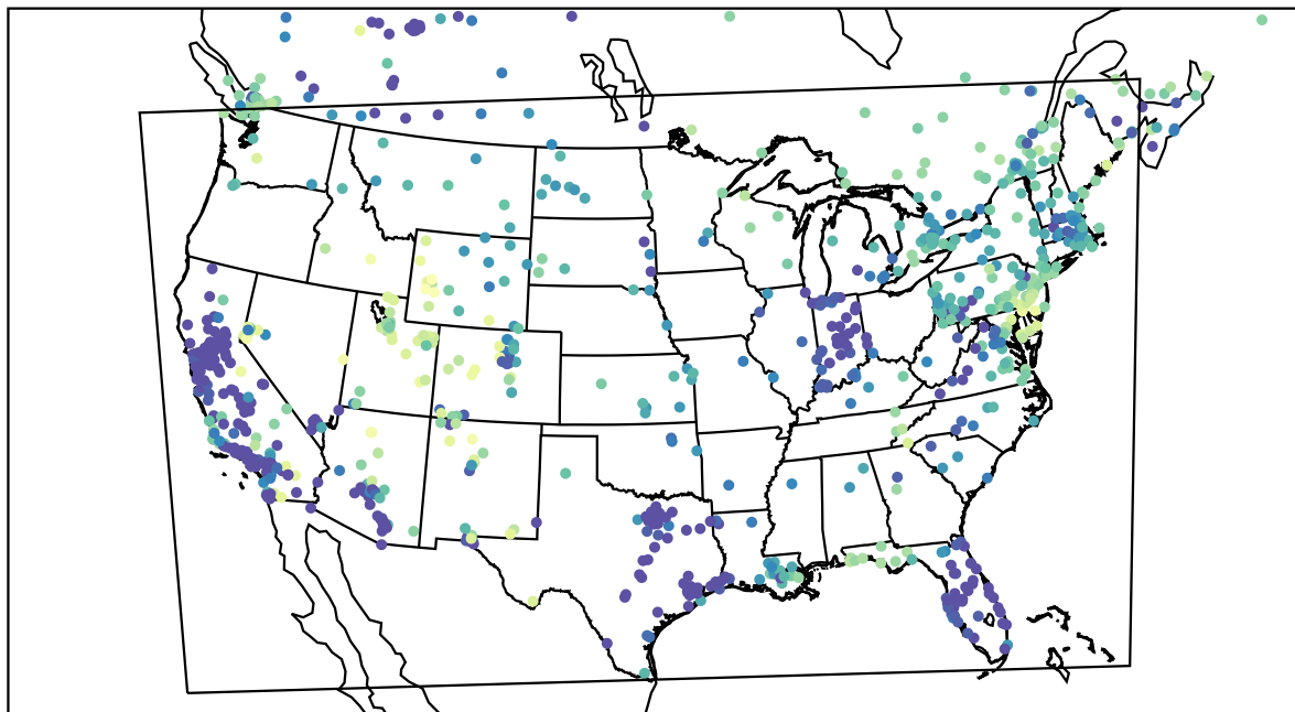
AirNOW (2024-01-13_05:00:00)
