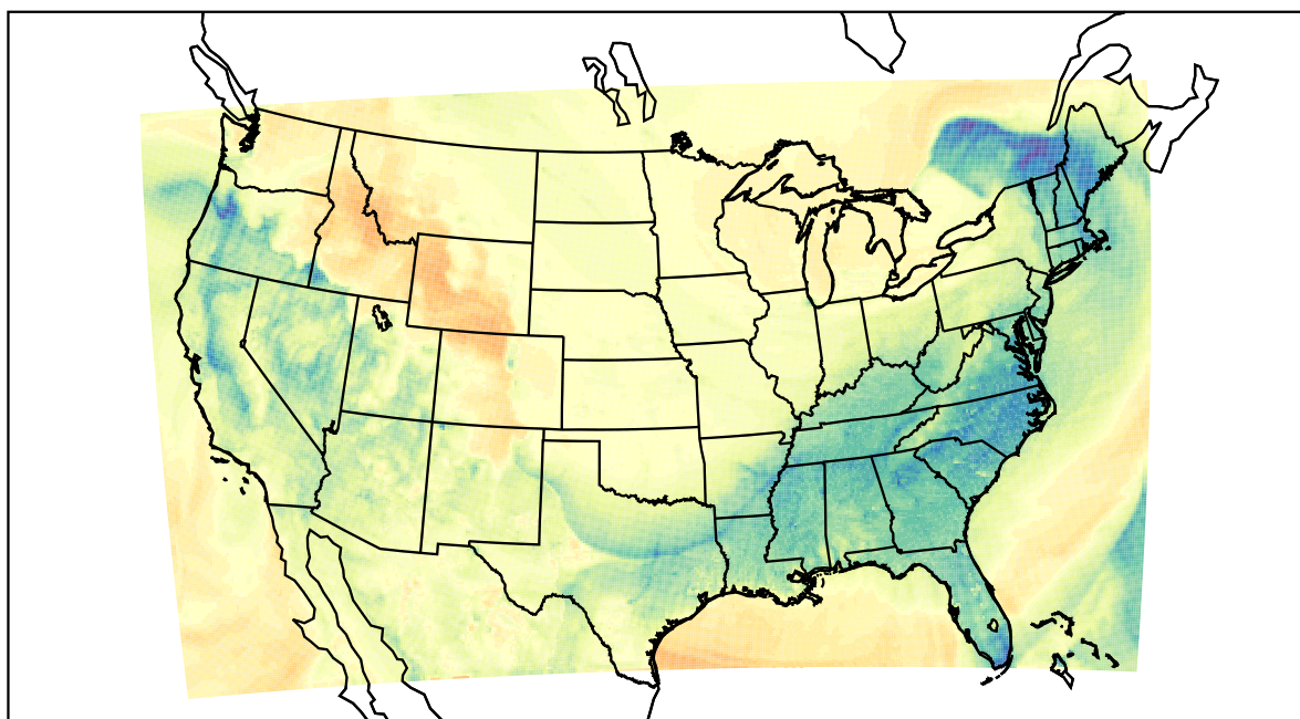
WRF (2024-01-14_00:00:00)
