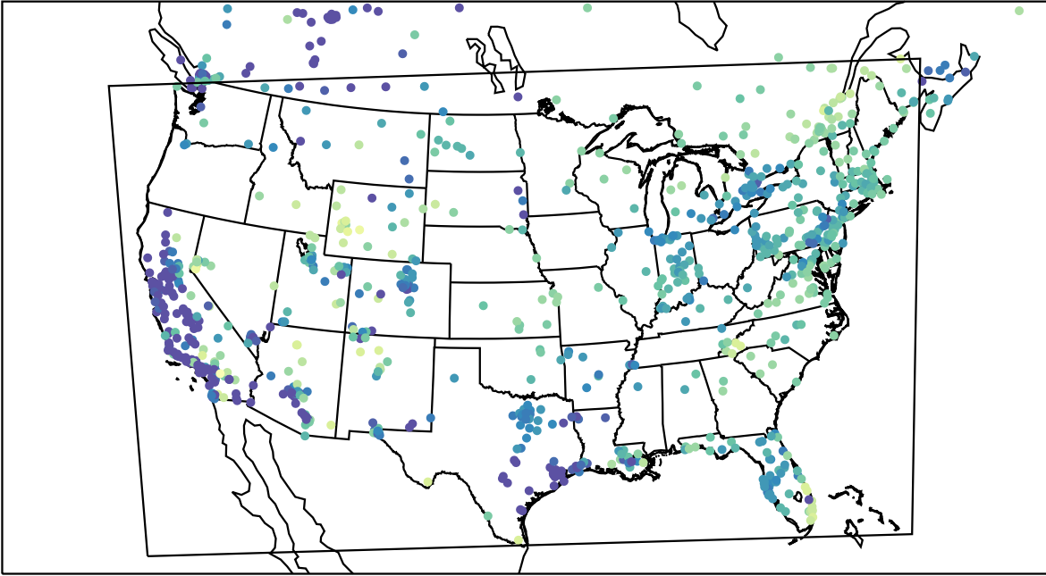
AirNOW (2024-01-14_16:00:00)
