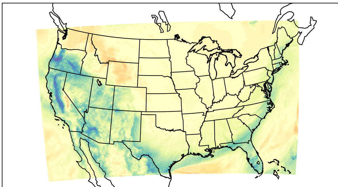
WRF (2024-01-14_17:00:00)
