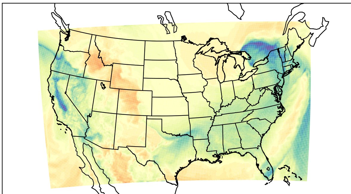
WRF (2024-01-13_19:00:00)
