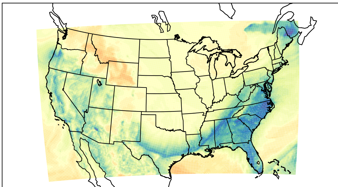
WRF (2024-01-14_06:00:00)
