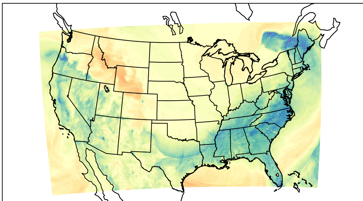
WRF (2024-01-14_01:00:00)
