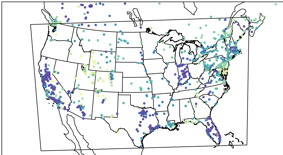
AirNOW (2024-01-13_04:00:00)
