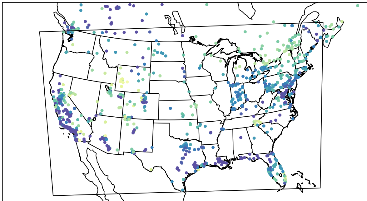
AirNOW (2024-01-14_08:00:00)
