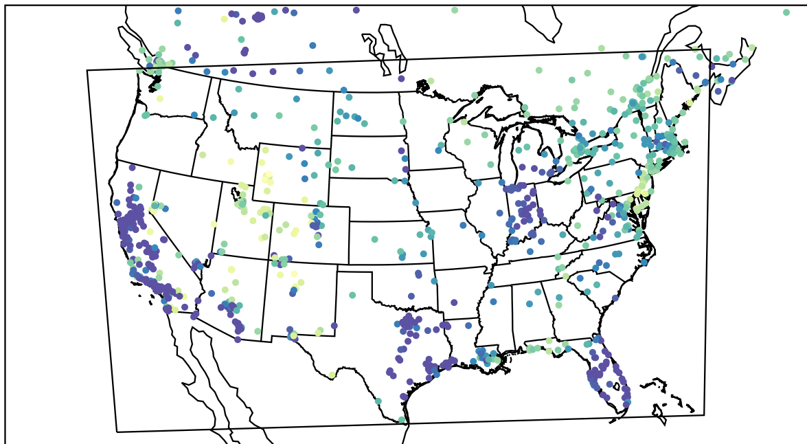
AirNOW (2024-01-13_06:00:00)
