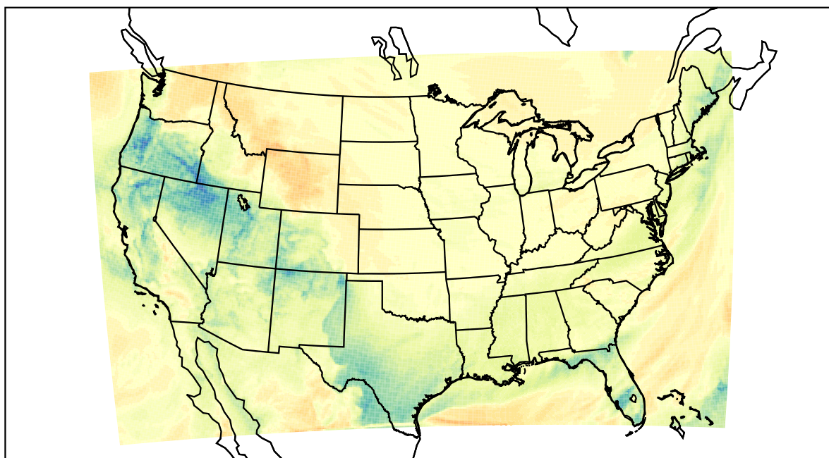
WRF (2024-01-14_21:00:00)
