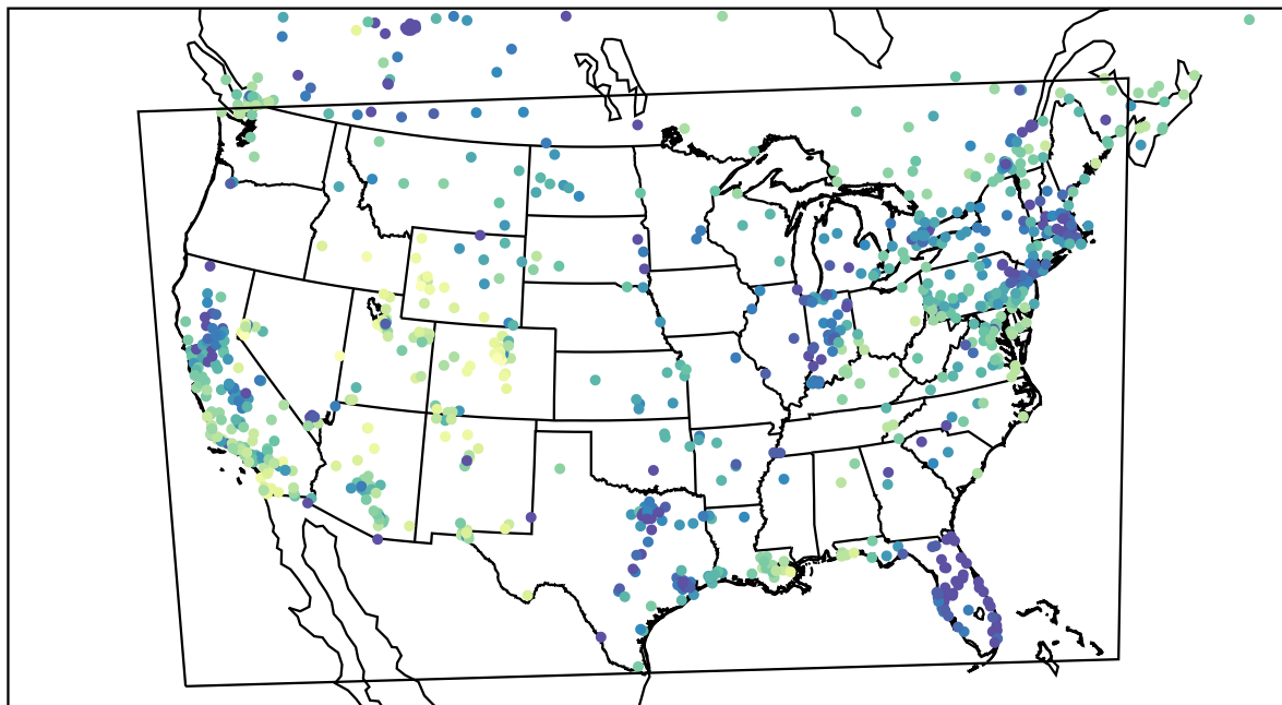
AirNOW (2024-01-13_00:00:00)
