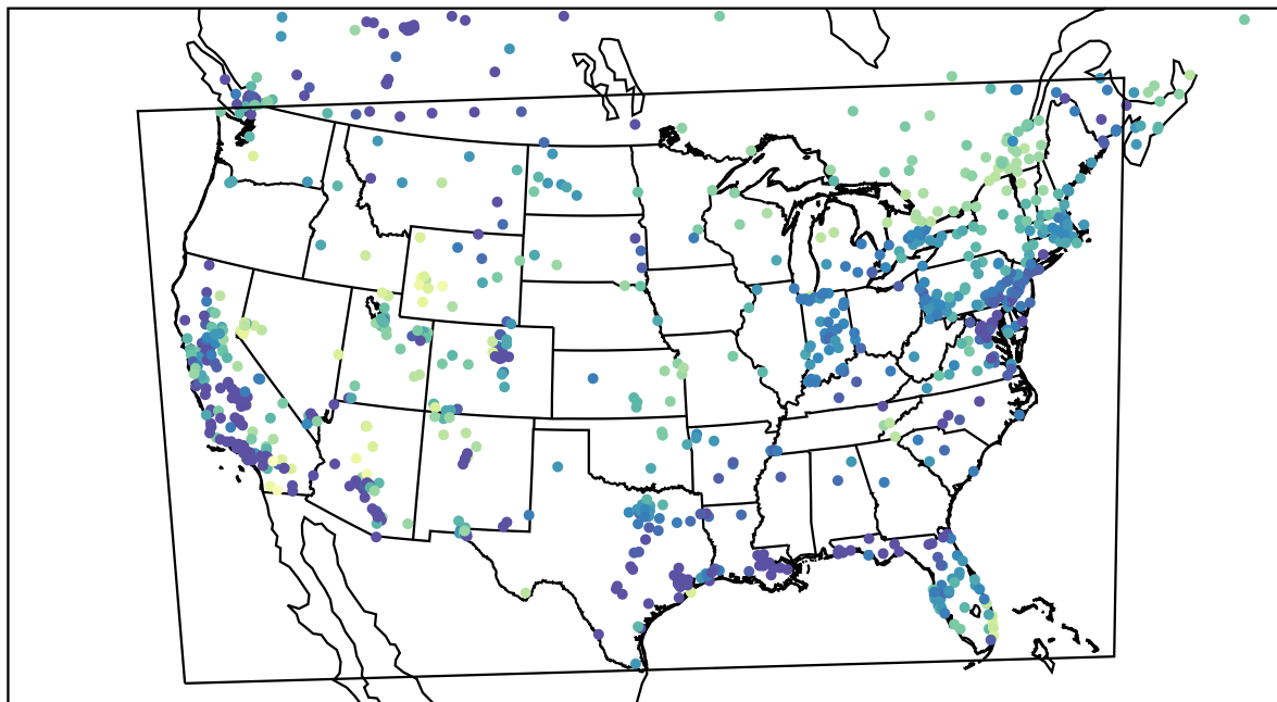
AirNOW (2024-01-14_09:00:00)
