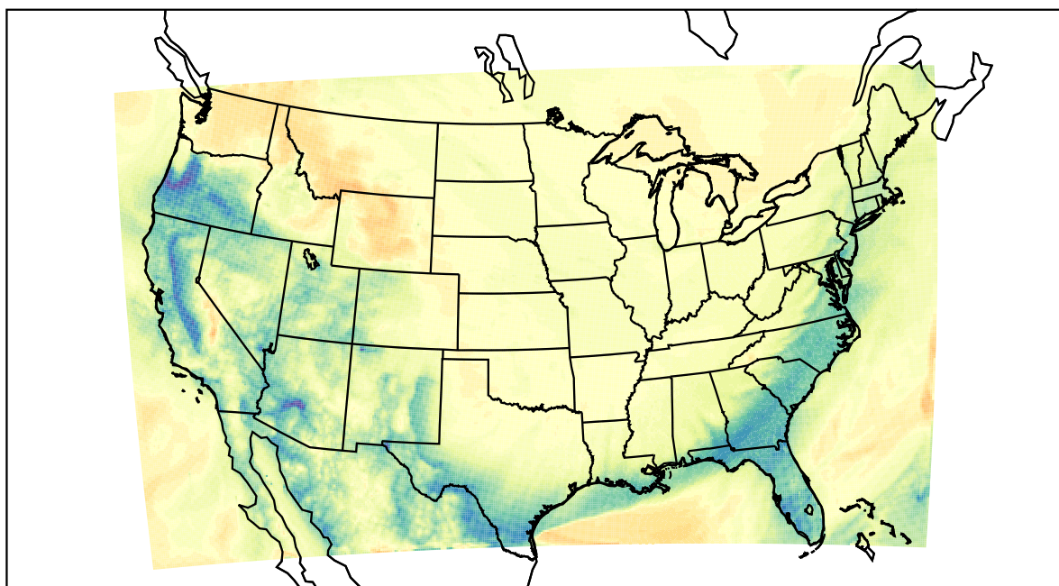
WRF (2024-01-14_15:00:00)
