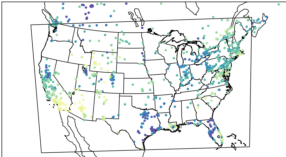
AirNOW (2024-01-14_23:00:00)
