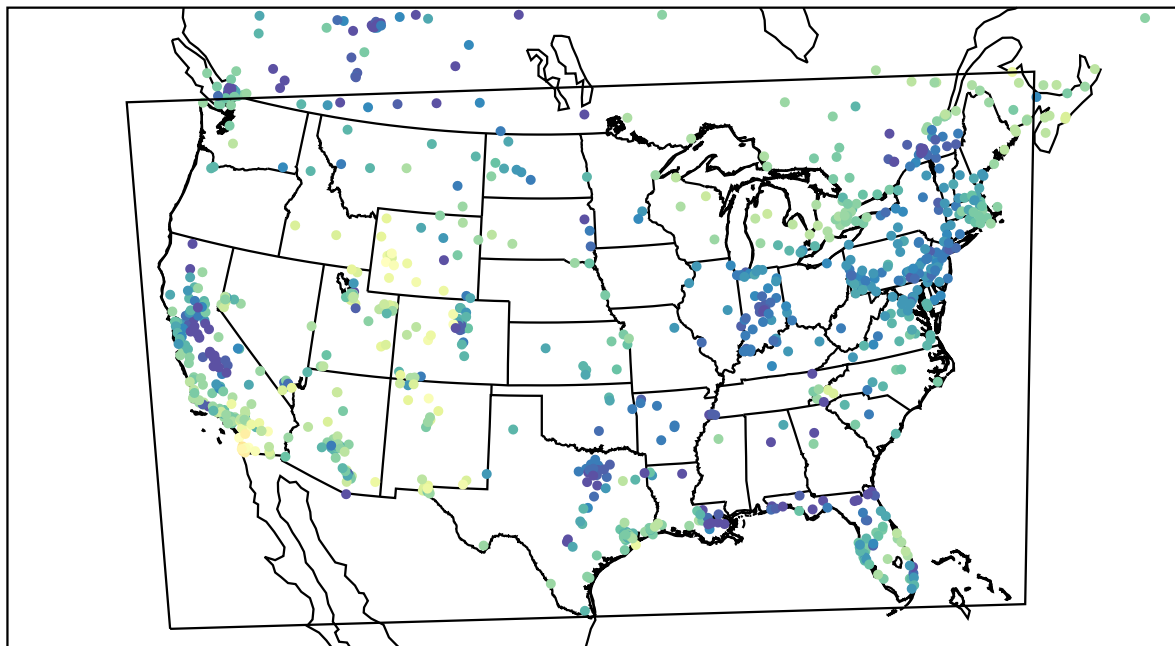
AirNOW (2024-01-14_00:00:00)
