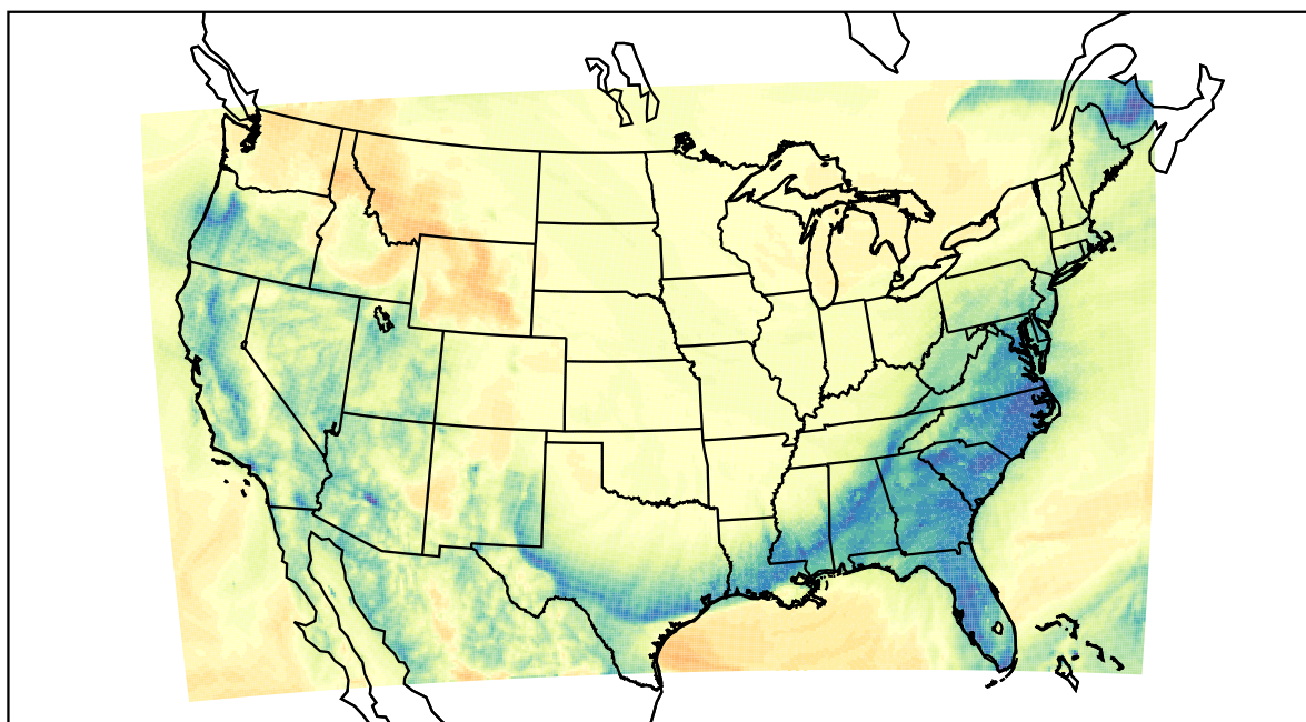
WRF (2024-01-14_08:00:00)
