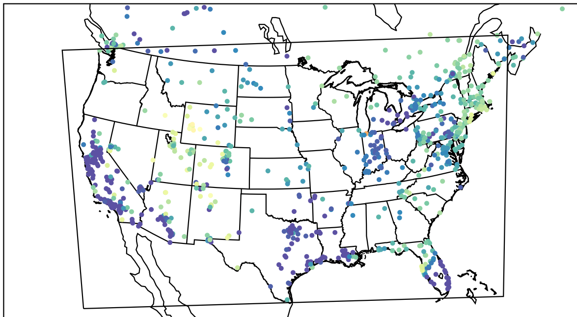
AirNOW (2024-01-13_10:00:00)
