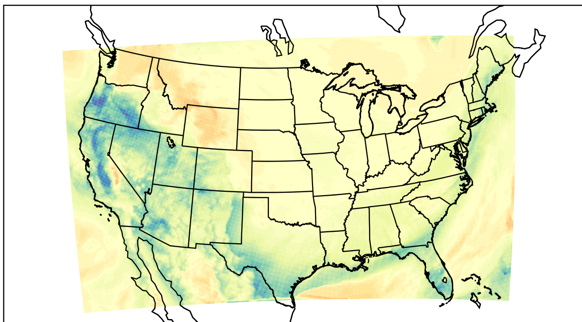
WRF (2024-01-14_18:00:00)
