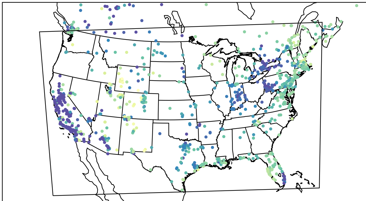
AirNOW (2024-01-13_16:00:00)
