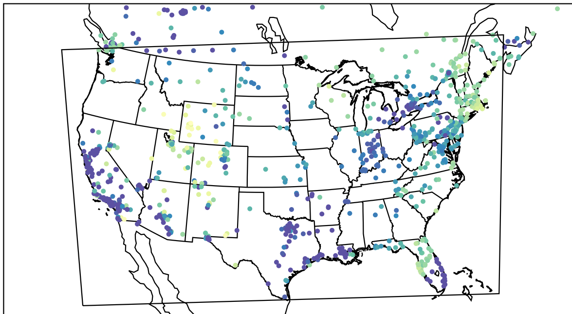
AirNOW (2024-01-13_12:00:00)
