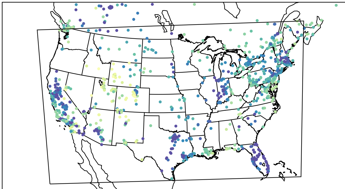
AirNOW (2024-01-13_01:00:00)
