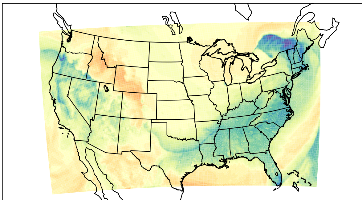
WRF (2024-01-13_23:00:00)
