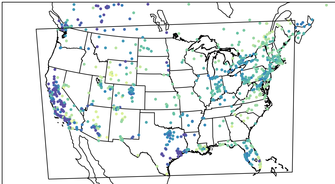
AirNOW (2024-01-14_17:00:00)
