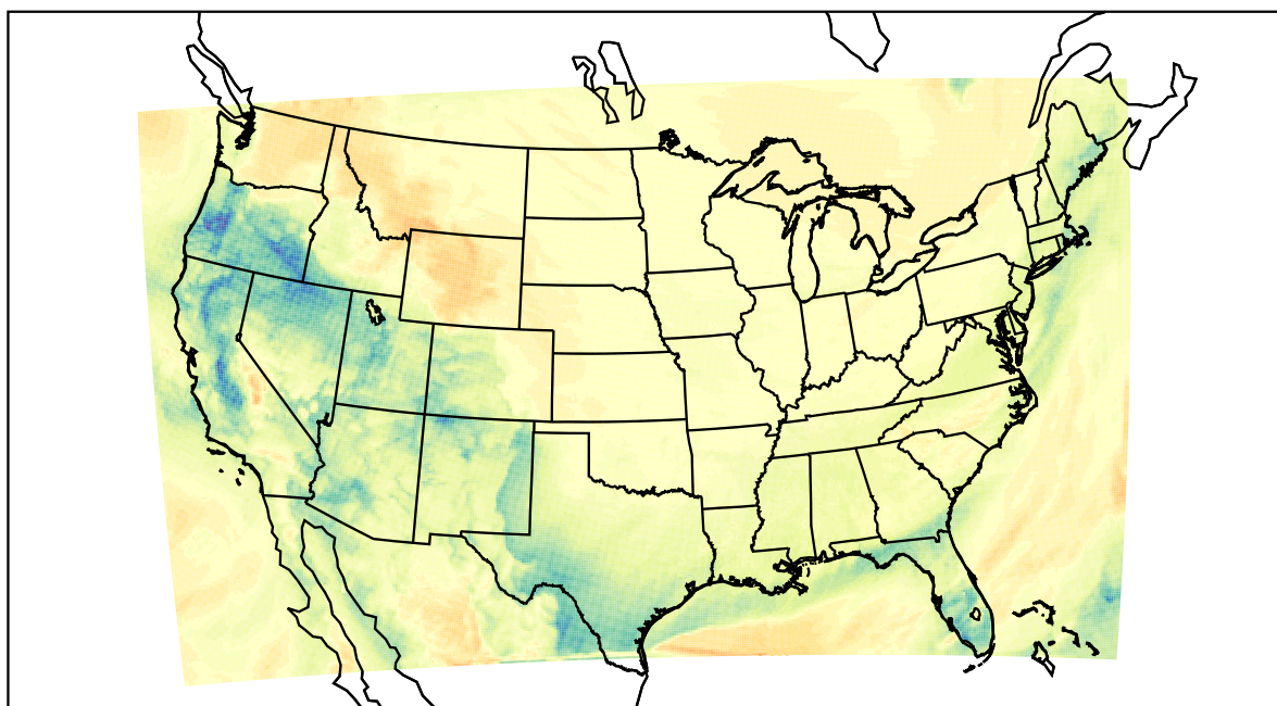
WRF (2024-01-14_19:00:00)
