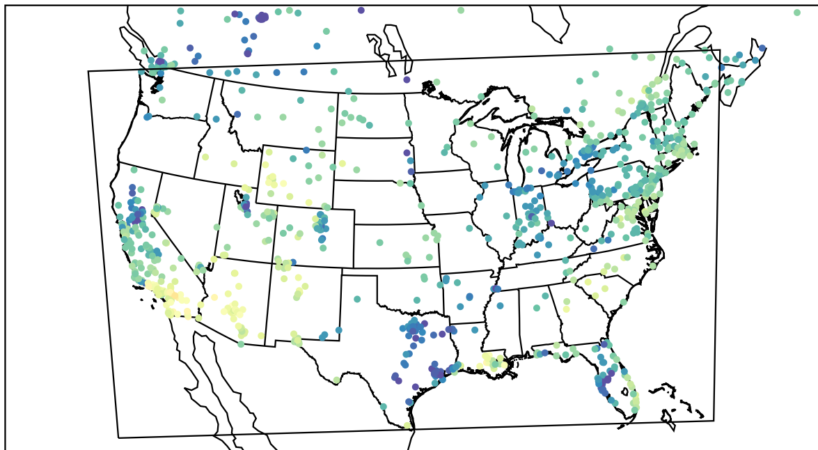
AirNOW (2024-01-14_22:00:00)
