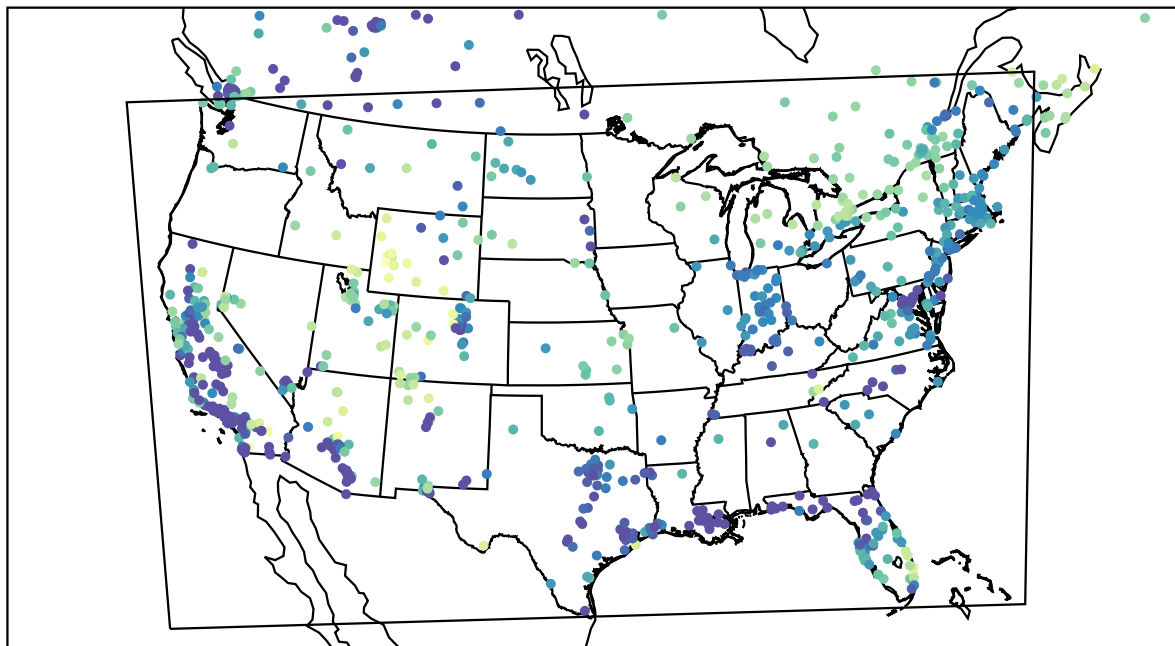
AirNOW (2024-01-14_06:00:00)
