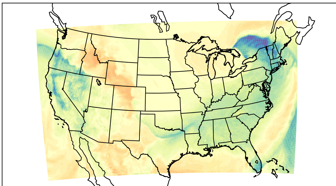
WRF (2024-01-13_21:00:00)
