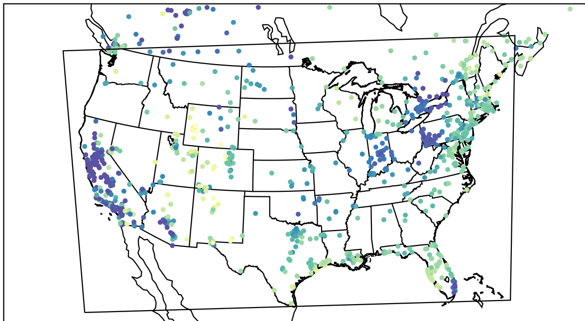
AirNOW (2024-01-13_17:00:00)
