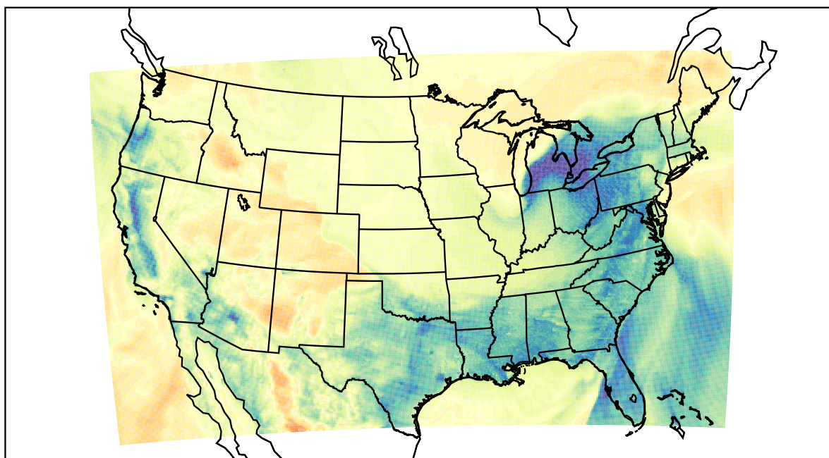
WRF (2024-01-13_08:00:00)
