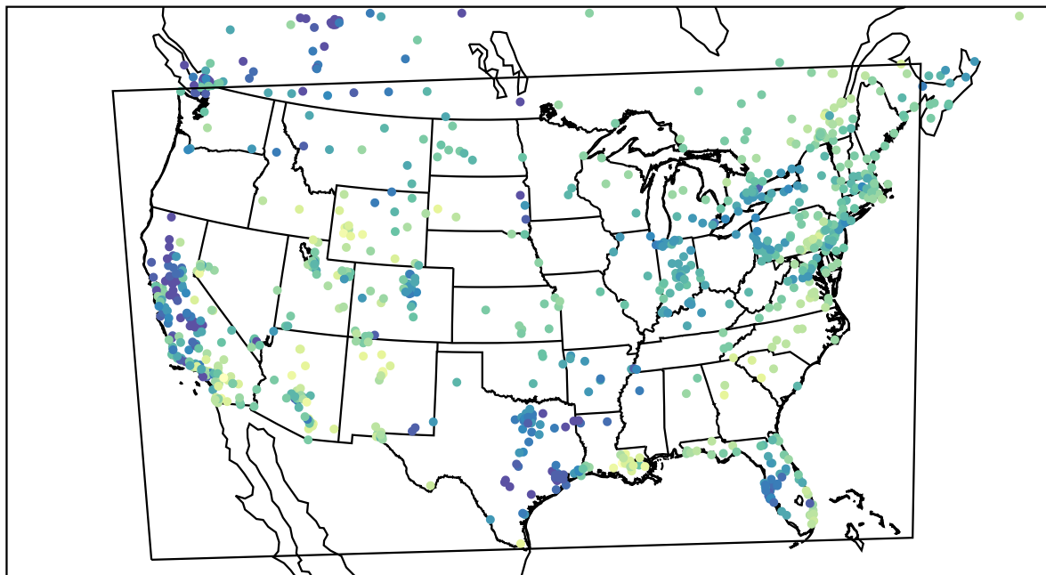
AirNOW (2024-01-14_18:00:00)
