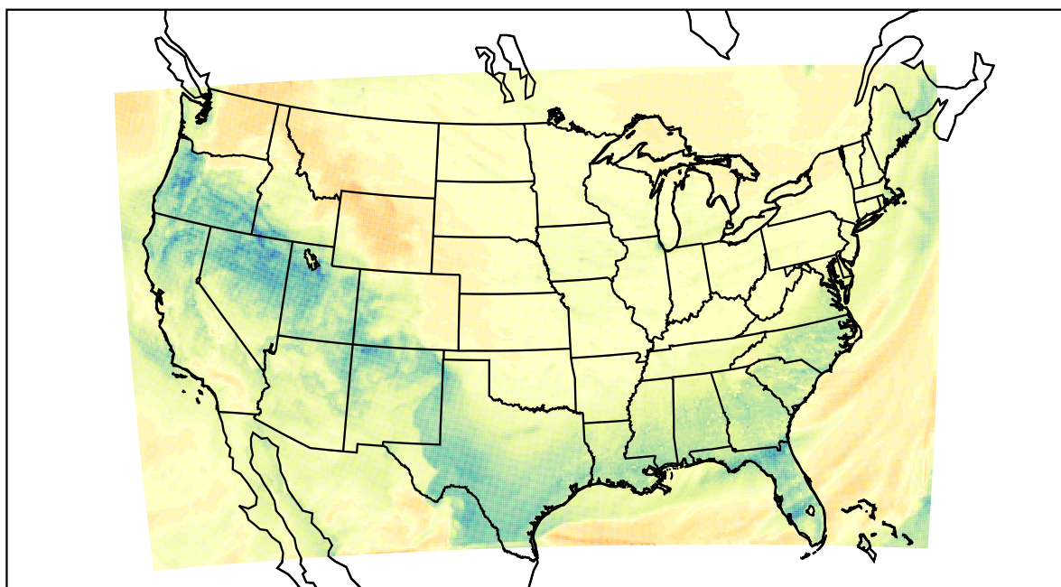
WRF (2024-01-14_23:00:00)
