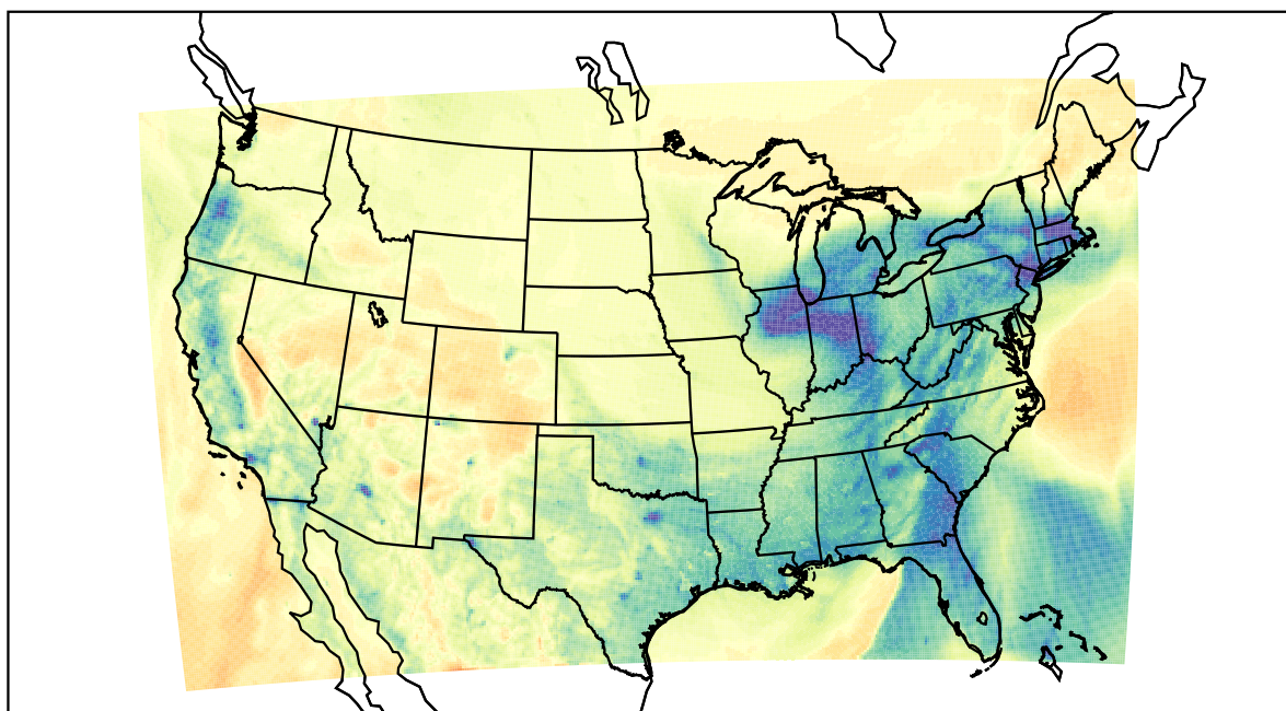
WRF (2024-01-13_02:00:00)
