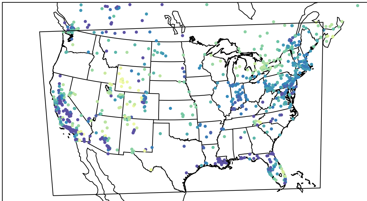
AirNOW (2024-01-14_04:00:00)
