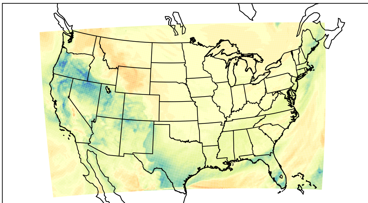
WRF (2024-01-14_20:00:00)
