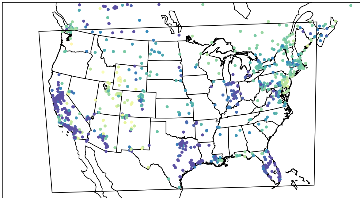
AirNOW (2024-01-13_07:00:00)
