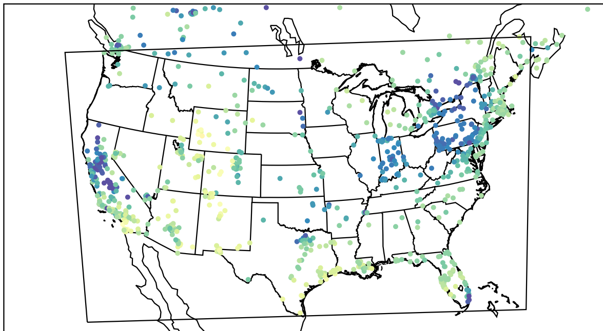
AirNOW (2024-01-13_20:00:00)
