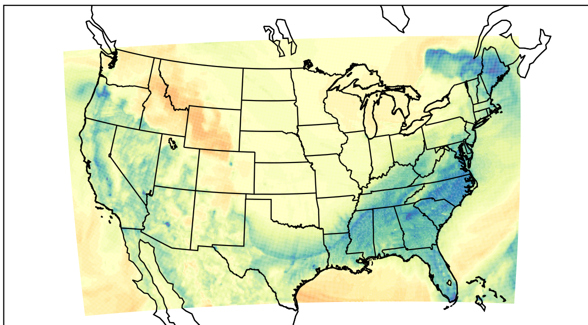
WRF (2024-01-14_02:00:00)
