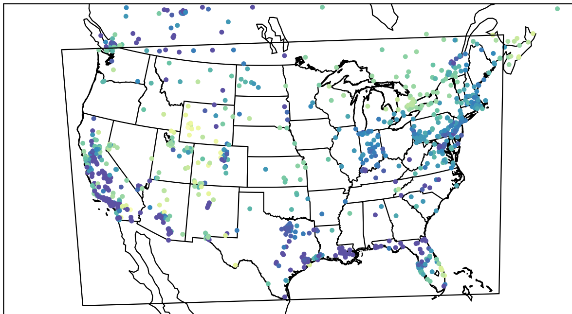
AirNOW (2024-01-14_05:00:00)
