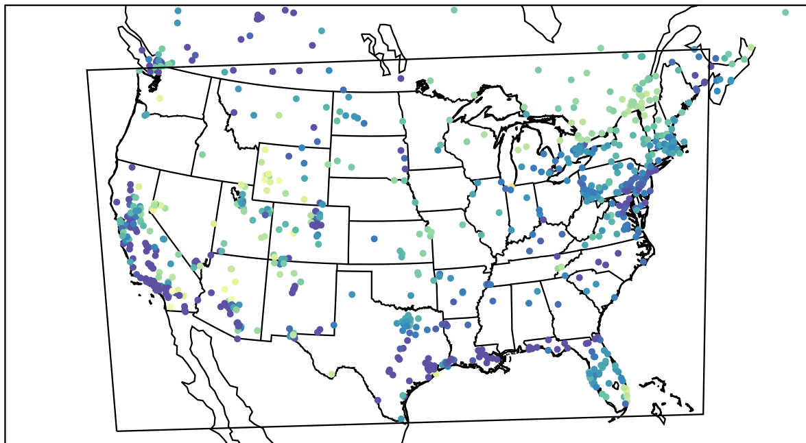
AirNOW (2024-01-14_10:00:00)
