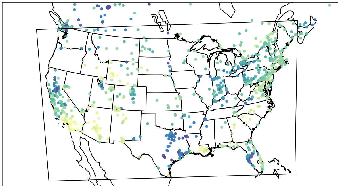
AirNOW (2024-01-14_21:00:00)
