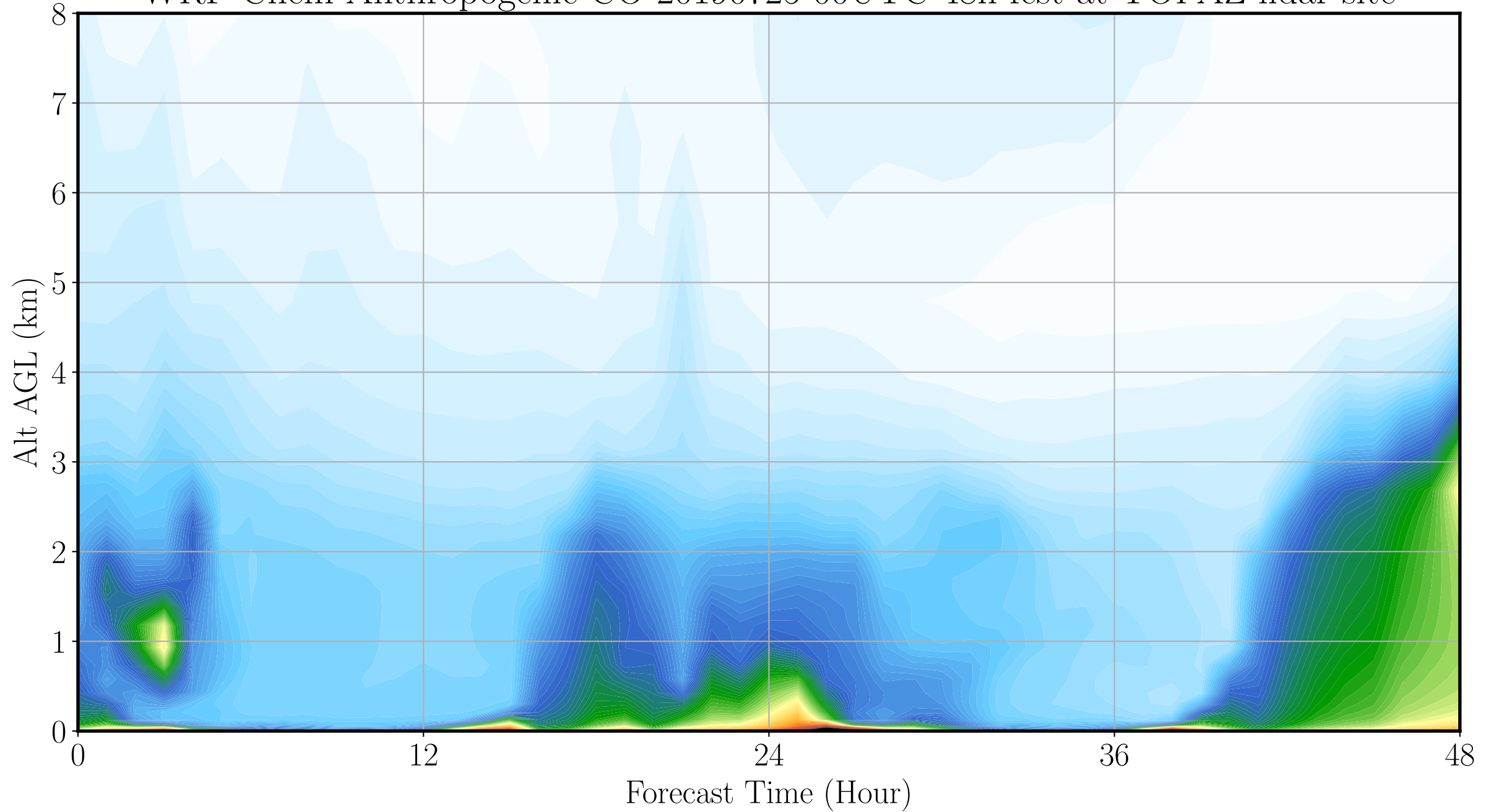
WRF-Chem Anthropogenic CO 20190725 00UTC 48h fcst at TOPAZ lidar site
