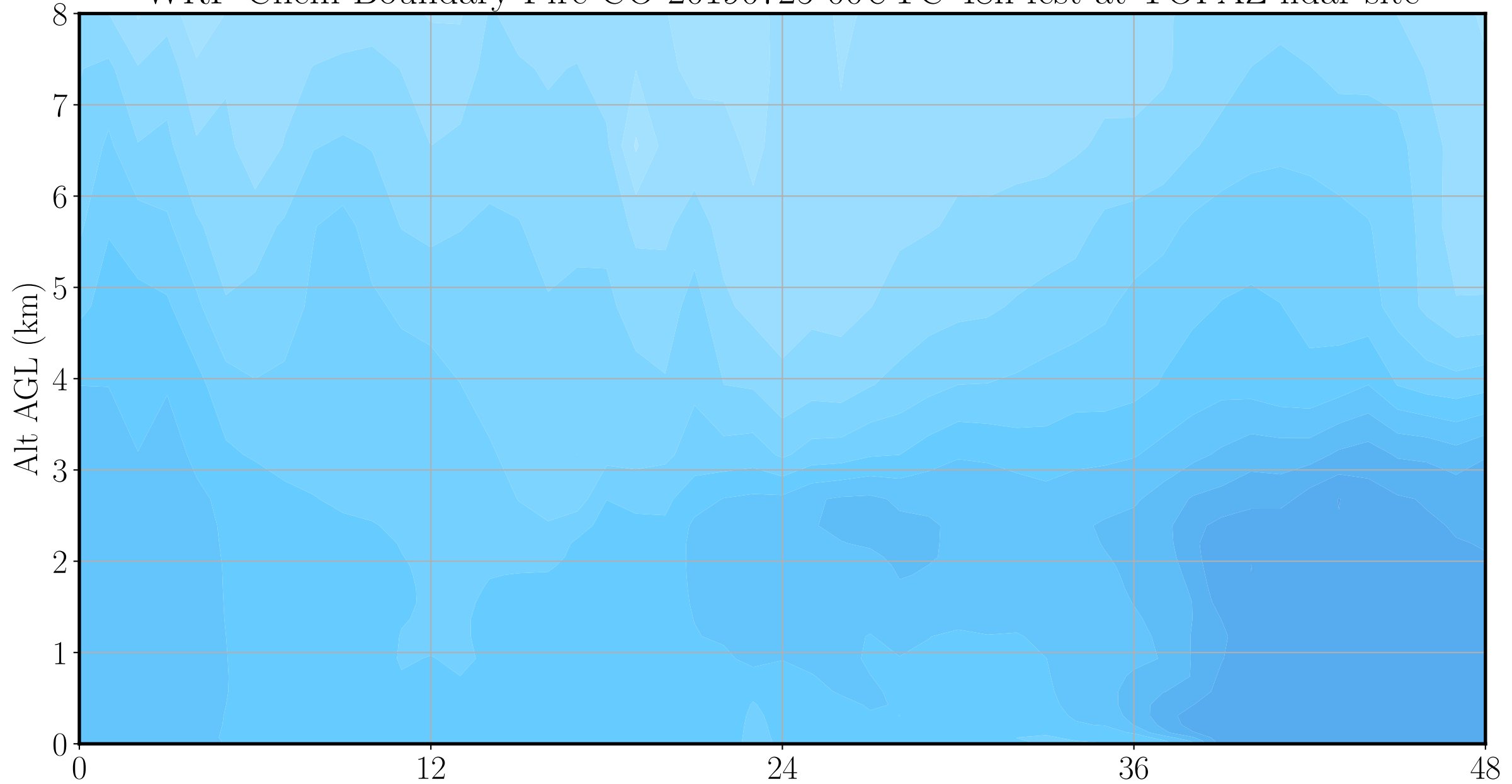
WRF-Chem Boundary Fire CO 20190725 00UTC 48h fcst at TOPAZ lidar site
