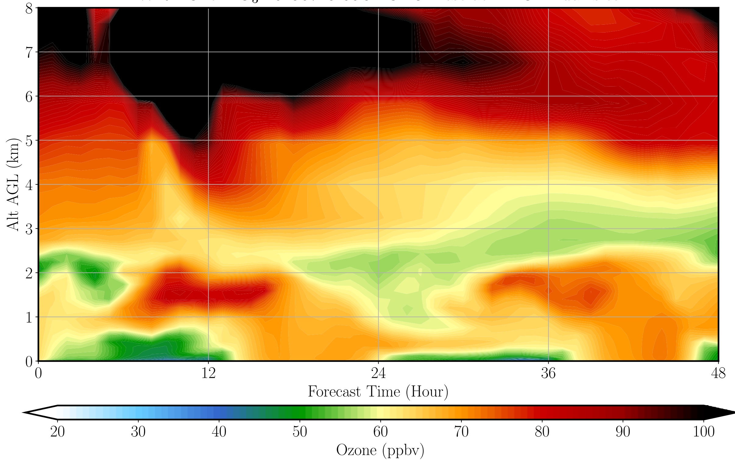
WRF-Chem O 3 20190725 00UTC 48h fcst at LMOL lidar site
