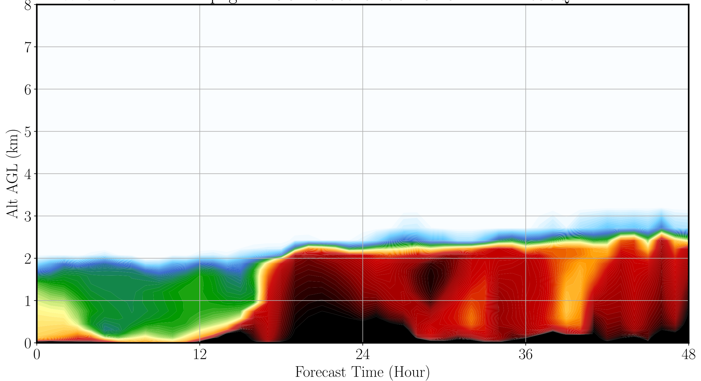
WRF-Chem Anthropogenic CO 20190725 00UTC 48h fcst at RO3QET lidar site
