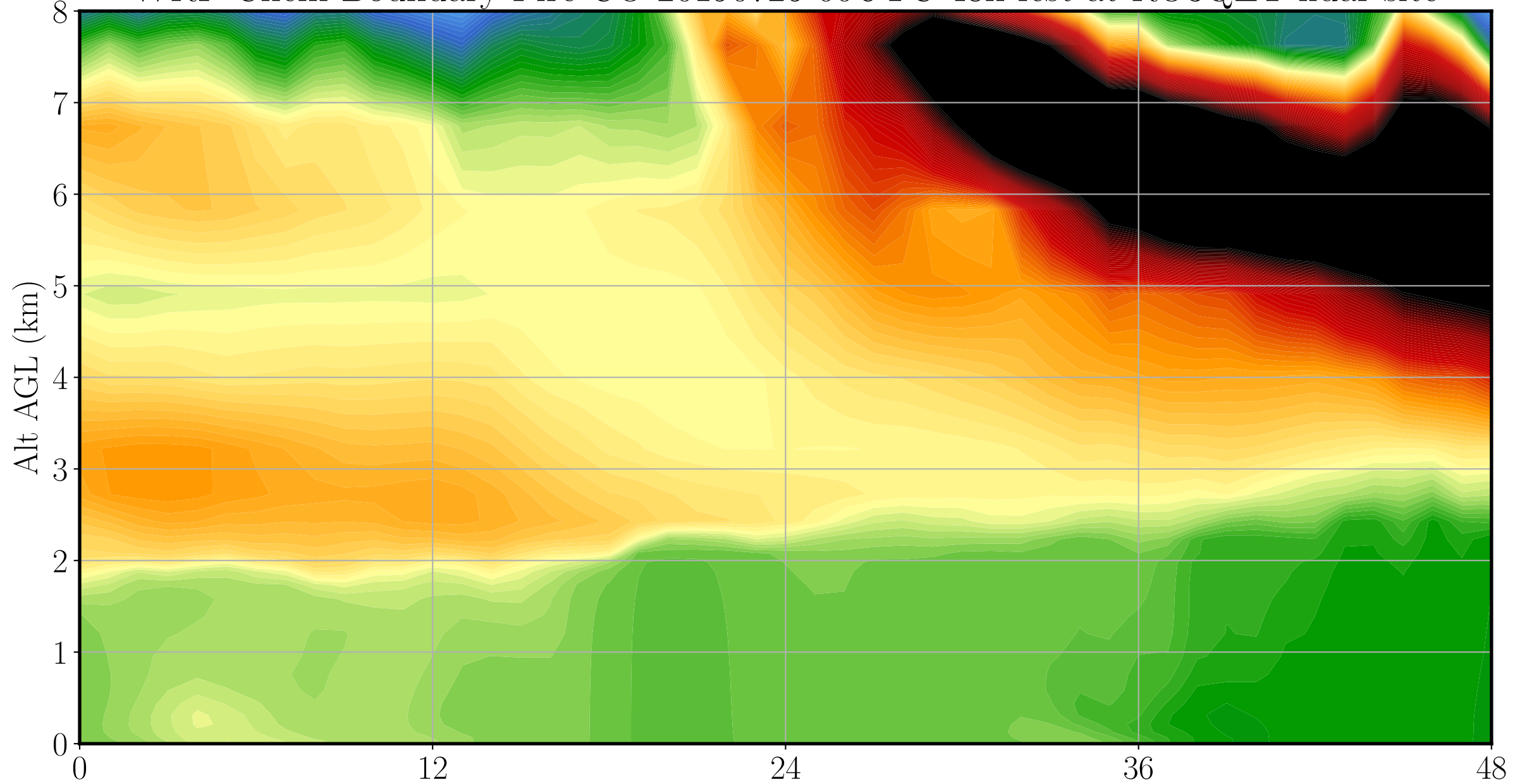
WRF-Chem Boundary Fire CO 20190725 00UTC 48h fcst at RO3QET lidar site
