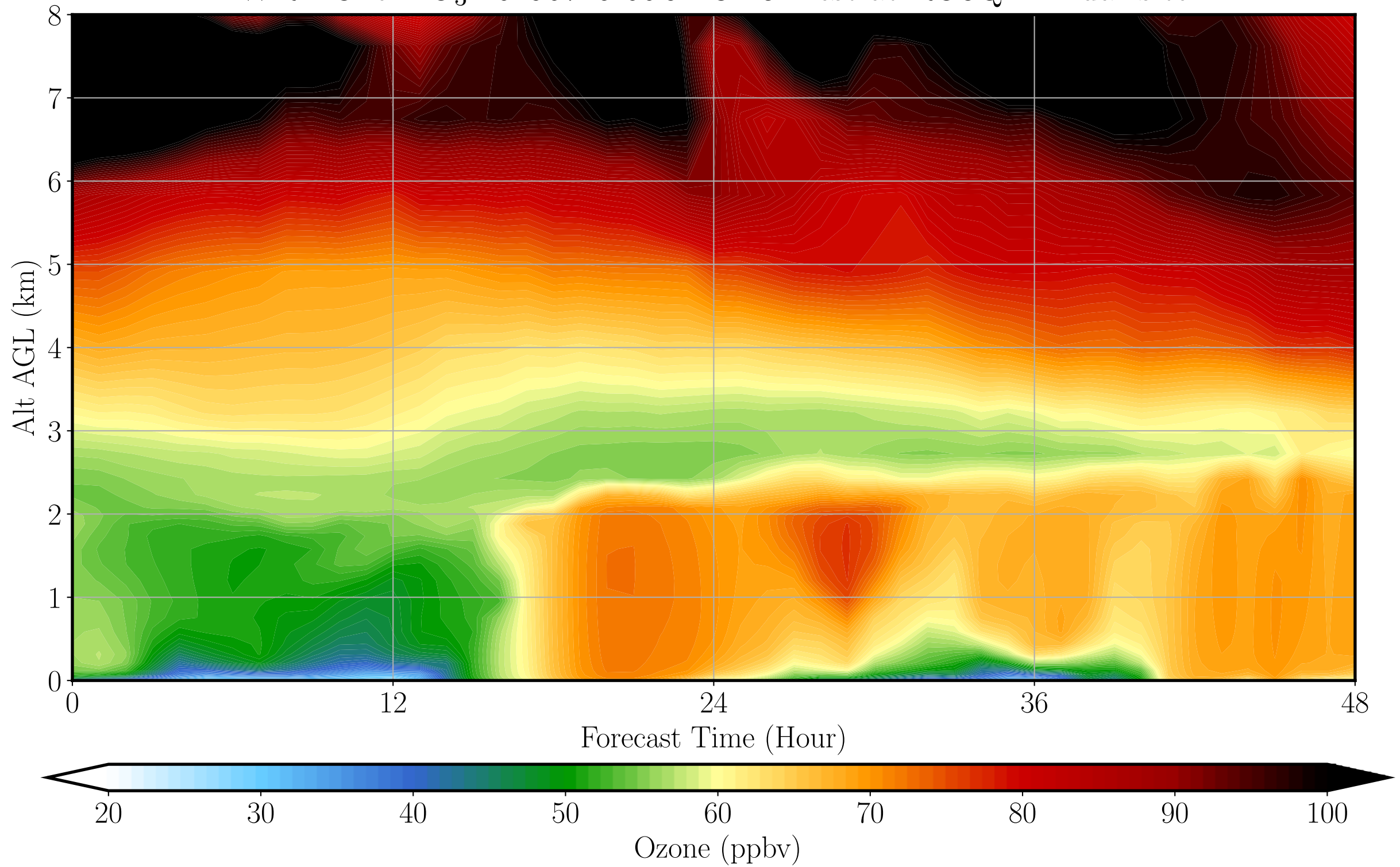
WRF-Chem O 3 20190725 00UTC 48h fcst at RO3QET lidar site
