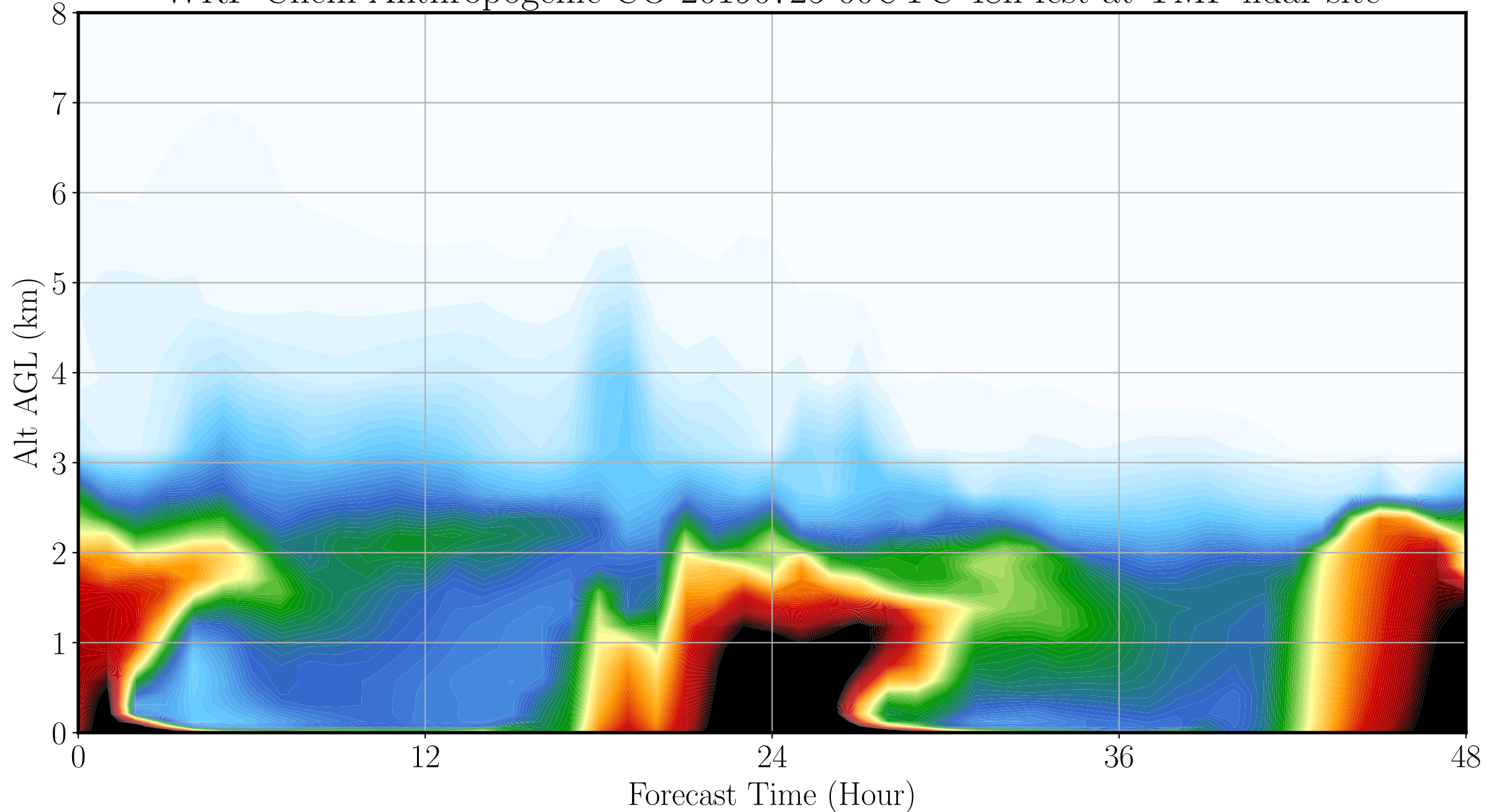
WRF-Chem Anthropogenic CO 20190725 00UTC 48h fcst at TMF lidar site
