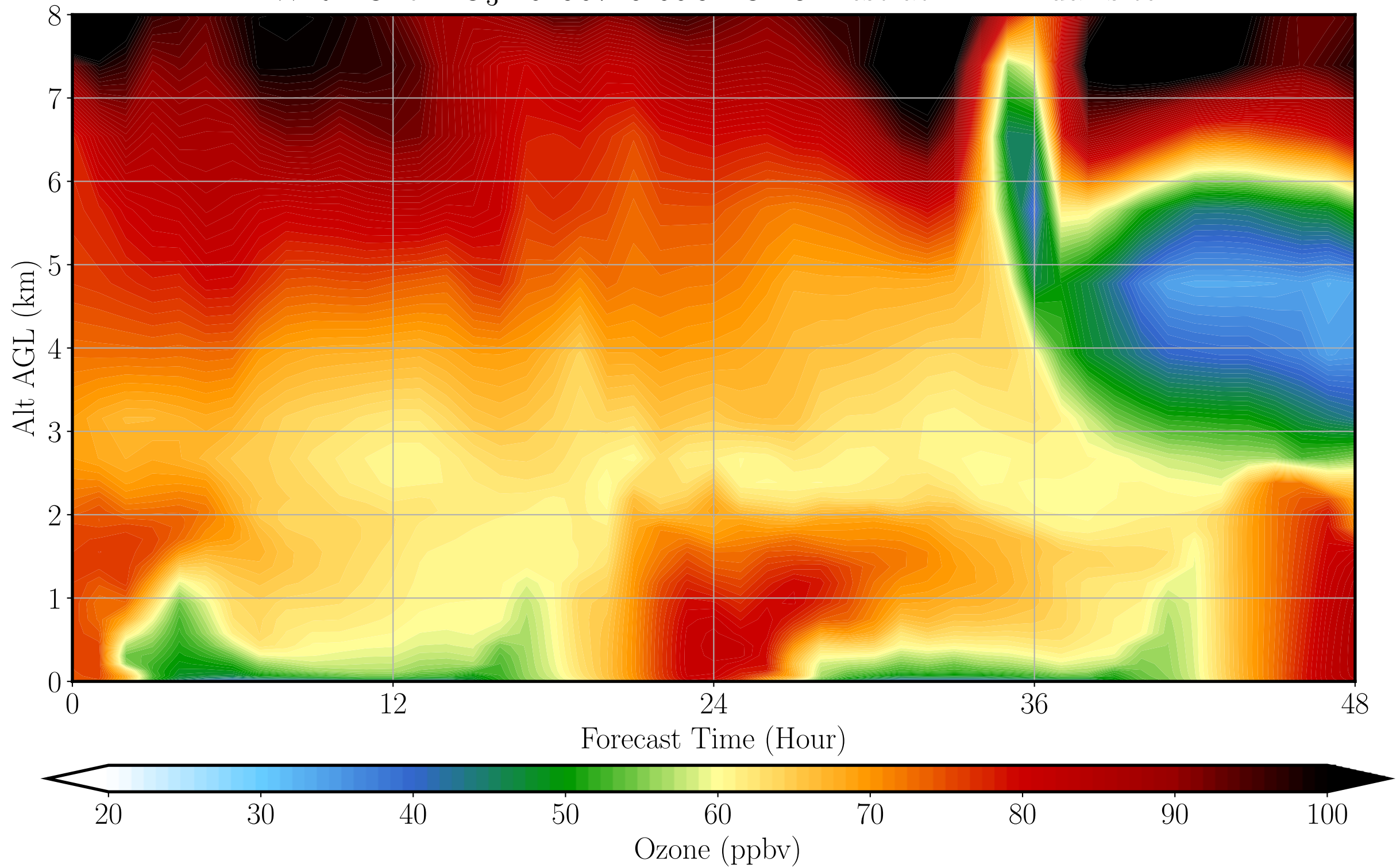
WRF-Chem O 3 20190725 00UTC 48h fcst at TMF lidar site
