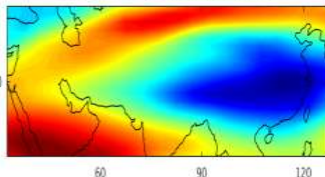
EOF5 var=1.39e+04 4.84%
