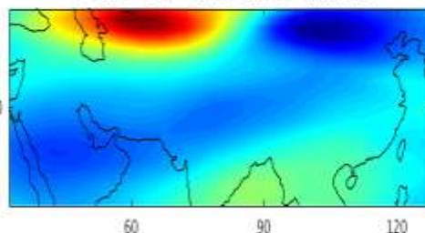
EOF6 var=9.18e+03 3.19%
