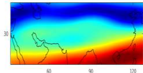
EOF2 var=4.61e+04 16%
