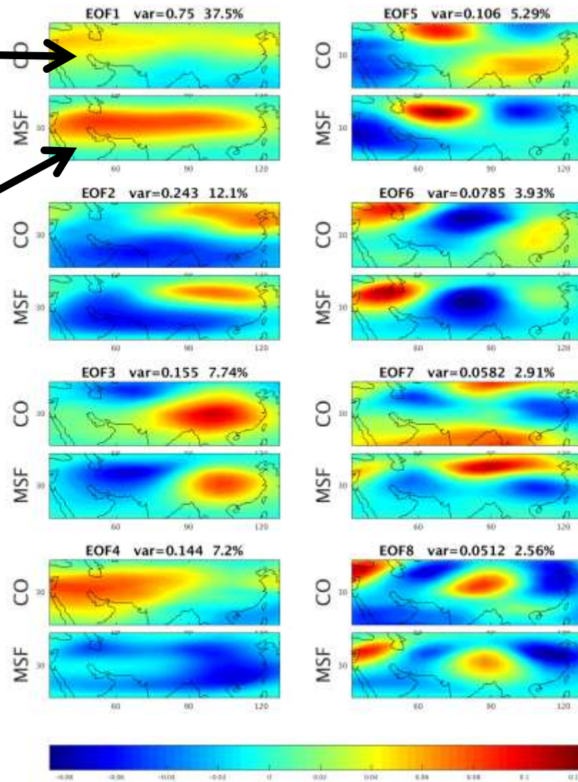
Joint EOFs of CO and MSF
