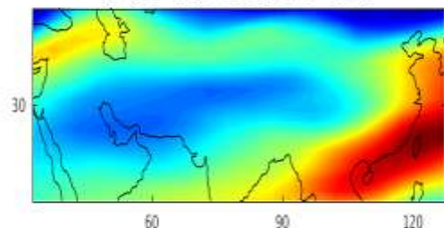
EOF3 var=2.16e+04 7.53%
