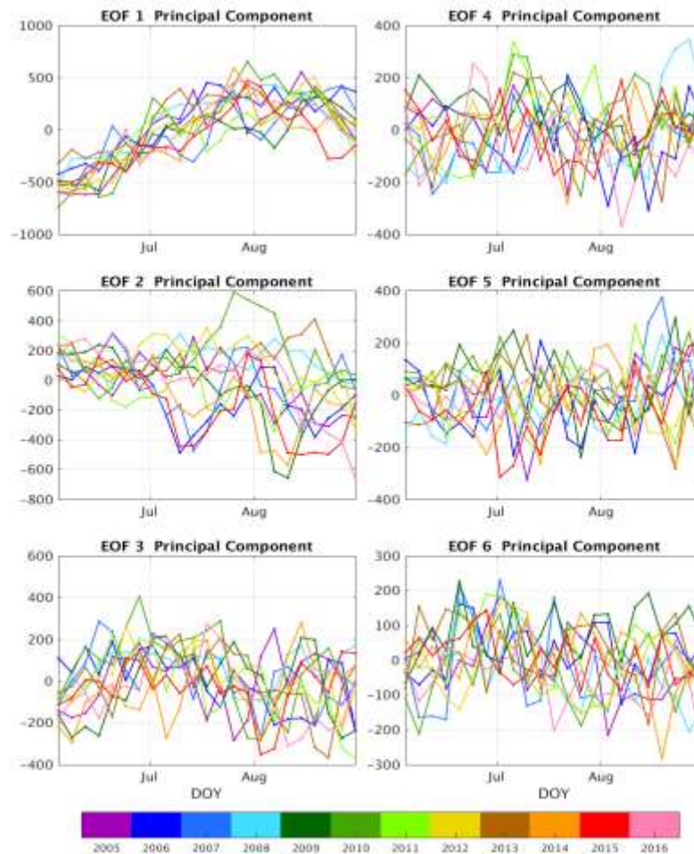
O3 370K Principal Components 2005–2016 200ppmv Ceiling
